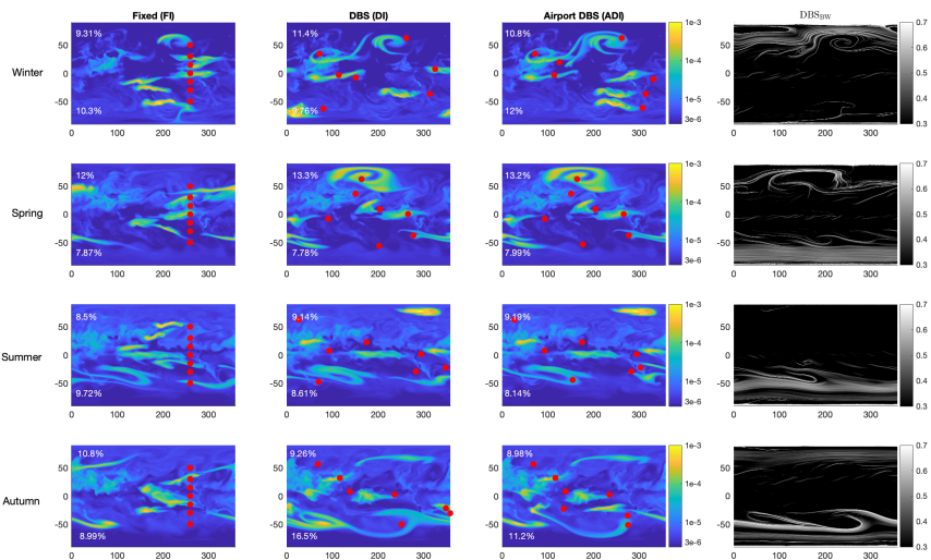
370 Figure 10: Analysis of CESM2 (WACCM6) output showing the \text{SO}_4 burden after seven days of transport for the three injection protocols in each season. The percent of the earth's surface covered by an \text{SO}_4 burden greater than the global mean from the week prior to injection is noted in the top left of each panel. Original injection locations for each experiment are shown as red dots. Units for the colormap are \text{kg m}^{-2} .
