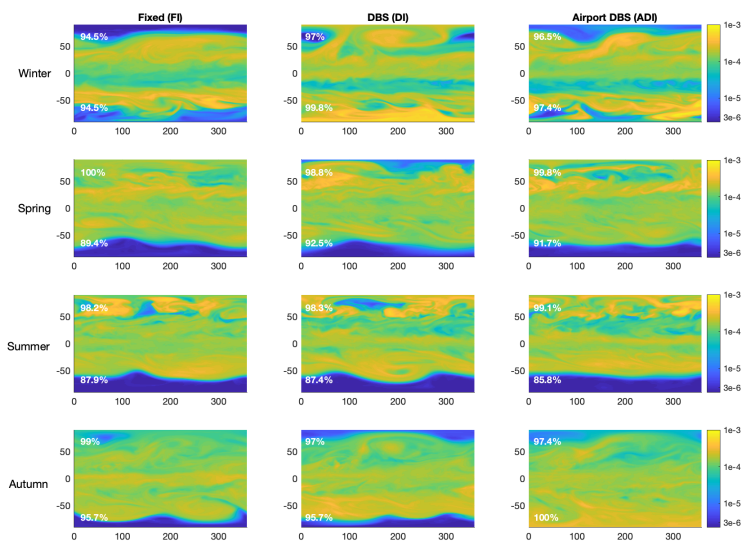
410 Figure 11: Analysis of CESM2 (WACCM6) output showing the \text{SO}_4 burden after eight weeks of transport for the three injection protocols in each season. The percent of the earth's surface covered by an \text{SO}_4 burden greater than the global mean from the week prior to injection is noted in the top left of each panel. Units for the colormap are \text{kg m}^{-2} .
