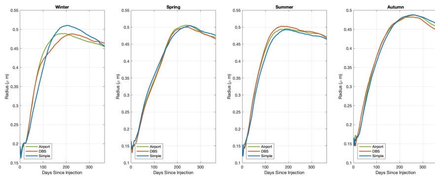
Figure 12: Mass-averaged effective radius of injected SO 4 aerosols on the 540 K isentrope spanning one year of CESM2(WACCM6) simulations after injection.
