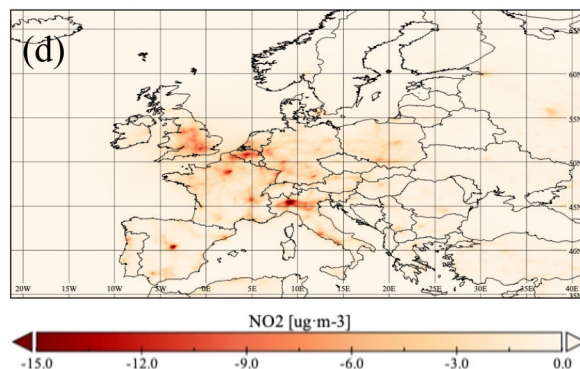
Daily average NO 2 differences (23/03/2020 – 26/04/2020)
