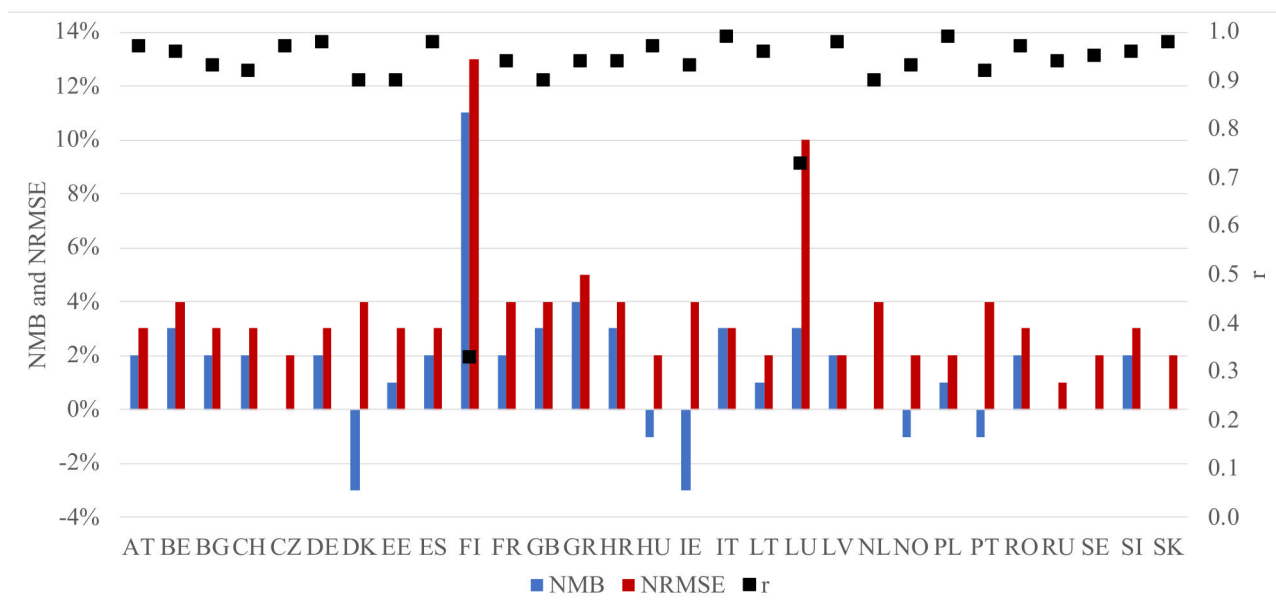
785 Figure 2: Summary of the statistics (normalized mean bias, NMB; normalized root mean square error, NRMSE and correlation, r) obtained from the comparison between measured and computed electricity demand during the first two months of 2020 for selected countries.
