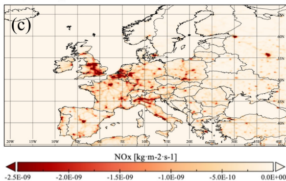
Daily average NO x differences (23/03/2020 – 26/04/2020)
