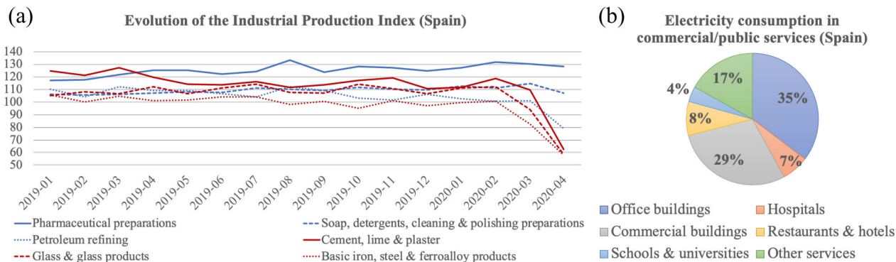
Figure 4. Evolution of the Industrial production Index in Spain for selected manufacturing industrial branches between January 2019 and April 2020 (INE, 2020) (a). Contribution of each commercial and public service branch to total electricity consumption in Spain for 2017 (IDAE, 2018) (b).
