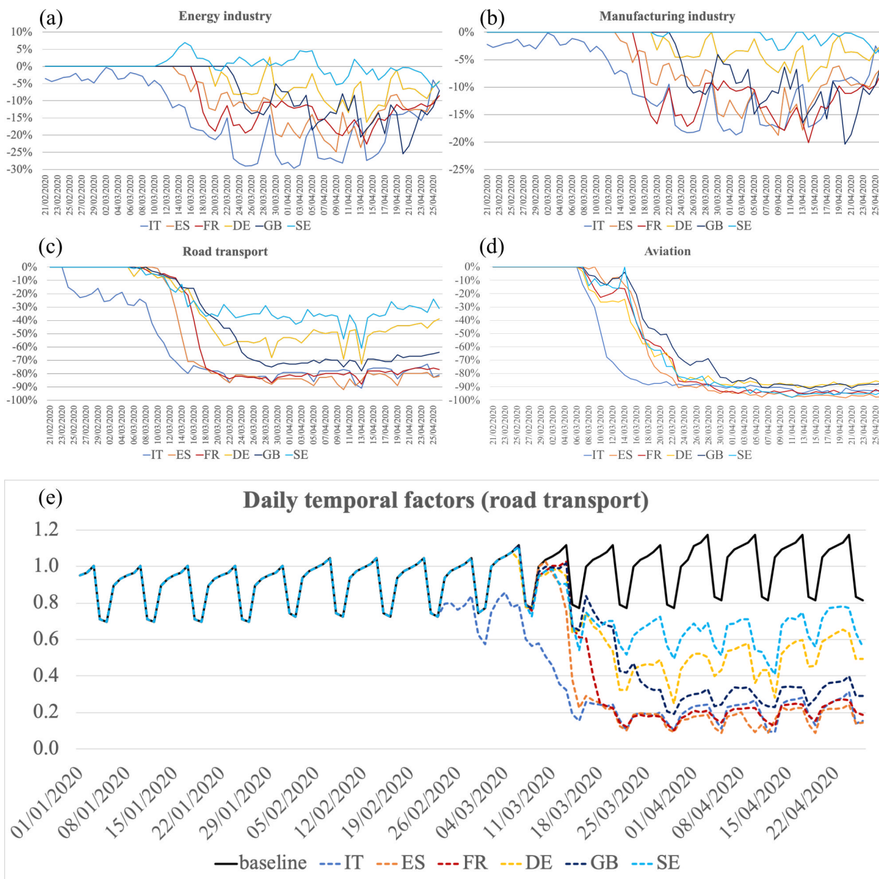
790 Figure 3. Emission reduction factors computed for the energy (a) and manufacturing (b) industry, road transport (c) and aviation (d) for selected countries (IT, Italy; ES, Spain; FR, France; DE, Germany; GB, Great Britain; SE, Sweden) for the period 21 February to 26 April 2020. Original and COVID-19 version of the emission daily temporal factors computed for the road transport sector and used for emission modelling (e).
