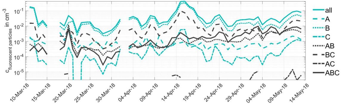
Figure A2: Time series of fluorescent particle number concentrations. The number concentrations of fluorescent particles measured by WIBS in different excitation emission wavelength pair combinations (fluorescence groups) are shown from 11 March 2018 to 13 May 2018. The definition of the different fluorescence groups is based on the categorization given in Savage et al. (2017). A summary of this categorization is given in Section 2.3.
