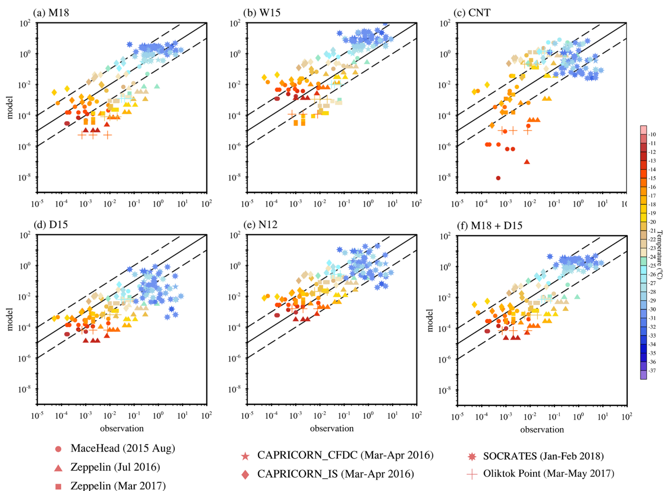
Figure 4. Comparison of simulated versus observed INP number concentrations for different simulations: (a) MOA INPs from M18 (McCluskey et al., 2018), (b) MOA INPs from W15 (Wilson et al., 2015), (c) dust INPs from CNT (Wang et al., 2014), (d) dust INPs from D15 (DeMott et al., 2015), (e) dust INPs from N12 (Niemand et al., 2012), and (f) the sum of dust and MOA INPs from D15 and M18. Simulated INP data are sampled at the same pressures, longitudes, and latitudes as the field measurements. Dashed lines outline a factor of 10 about the 1 : 1 line (solid) in all the panels. The color bar shows the observed temperature in degrees Celsius, while different markers represent different field campaigns. The Zeppelin site is located at 78.9081° N, 11.8814° E, 475 m above mean sea level in Ny Ålesund, Svalbard; the INP data were collected during July 2016 and March 2017 (Tobo et al., 2019). The Oliktok Point site is located at 70.50° N 149.89° W; the INP data were collected from March to May 2017 (Creamean et al., 2018). The CAPRICORN (Clouds, Aerosols, Precipitation, Radiation, and Atmospheric Composition over the Southern Ocean) INP data were collected on ships from 13 March to 15 April in 2016 over the Southern Ocean (McCluskey, et al., 2018a). The Mace Head site is located at 53.32° N, 9.90° W; the INP data were collected during August 2015 (McCluskey et al., 2018b). The SOCRATES (Southern Ocean Clouds, Radiation, Aerosol Transport Experimental Study) INP data were collected on flights in January and February 2018 over the Southern Ocean by Paul DeMott ( https://data.eol.ucar.edu/master_lists/generated/socrates/ , last access: February TSI 2021).
