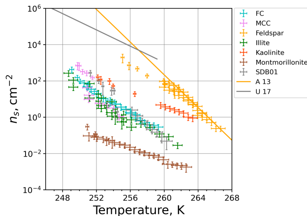
Figure 11. INAS densities of the investigated materials as function of temperature. The data points are composites from M-WT and M-AL measurements and are corrected for the cooling rate. Orange and gray solid lines show parameterizations for feldspar (Atkinson et al., 2013) and desert dust (Ullrich et al., 2017), respectively.
