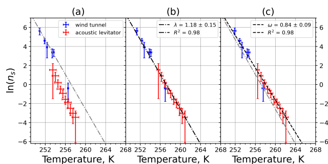
Figure A12. (a) Composite INAS density spectrum of Sahara dust from the uncorrected M-WT (blue) and M-AL (red) measurements. (b) and (c) show the temperature corrected data points from the M-WT and M-AL experiments based on \lambda and \omega , respectively. The dash-dotted line in (c) is the regression line on corrected data points obtained by employing the optimal \lambda -value as in (b).
