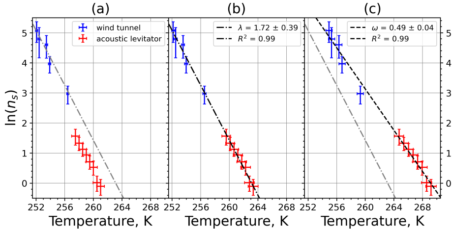
Figure 9. (a) Composite INAS density spectrum of kaolinite from the uncorrected M-WT (blue) and M-AL (red) measurements. (b) and (c) show the temperature-corrected data points from the M-WT and M-AL experiments based on \lambda and \omega , respectively. The dashed-dotted line in (c) is the regression line for the corrected data points obtained by employing the optimal \lambda -value as in (b).
