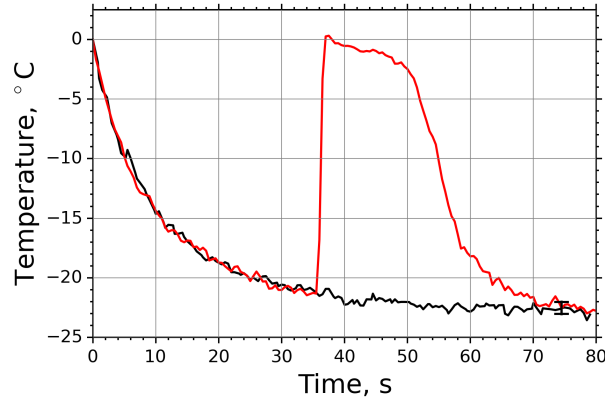
Figure 3. Measured surface temperatures of two droplets levitated in M-AL: examples of freezing (red line) and non-freezing (black line) events. The measurement uncertainty of the temperature was \pm 0.5\text{K} .
