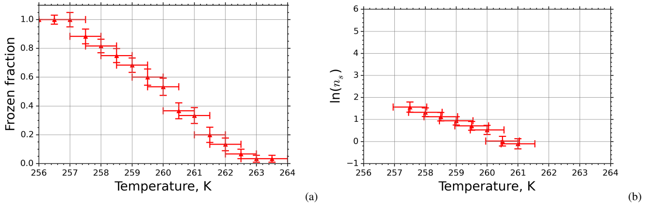
Figure 7. (a) Frozen fraction of 2 mm aqueous suspension droplets containing 1.265 g L -1 kaolinite measured in M-AL. (b) INAS density of kaolinite as function of temperature determined from the spectrum shown in (a).
