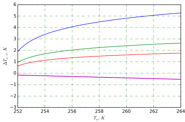
Figure B4. Temperature shift calculated for three different \lambda values (red: 0.8, green: 1.6., and blue: 2.4) in relation to temperature difference between drop surface and volume averaged drop temperature (magenta curve).
