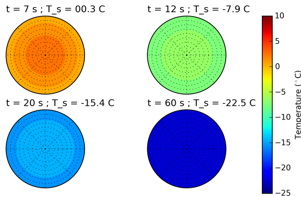
Figure B2. Internal temperatures at four different time instances for a continuously cooling drop of 2 mm diameter in M-AL following Fig. B1, based on numerical simulation of the heat conduction equation.
