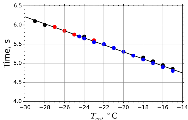
Figure 2. Time needed to approach the equilibrium temperature T_e with an accuracy of 0.2^\circ\text{C} as the function of air temperature T_\infty . Calculations carried out for dew point temperatures -30 , -27.5 , and -25^\circ\text{C} are plotted by black, red, and blue dots, respectively. The data points were calculated using Eq. (B21). The regression line is t_a = 3.46 - 0.09T_\infty ( T_\infty in ^\circ\text{C} ).
