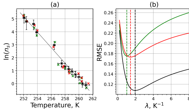
Figure 10. (a) Original (black; same as in Fig.9a ), and two within the experimental error interval randomly generated data sets (red and green) using the measured INAS densities of kaolinite. The black solid line is the linear fit to the original experimental data set. (b) RMSE as the function of lambda for two of the 1000 randomly generated data sets. The vertical dashed lines indicate the optimal lambda values for the red, green and black curves.
