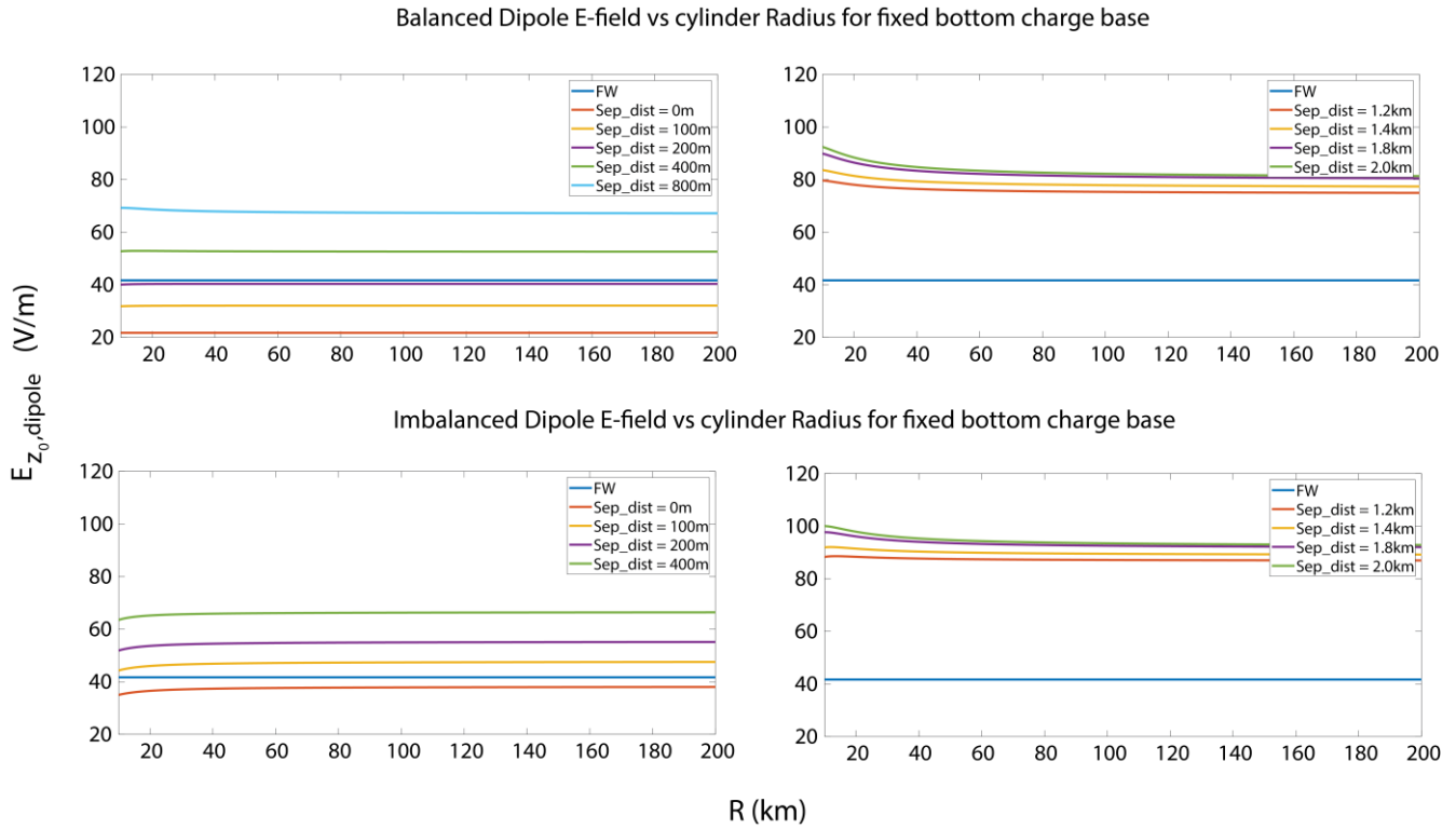
845 Fig. 10. Dipole electric field strength at ground level ( E_{z_0,dipole} ) as a function of the cylinder radius R , with the bottom cylinder at 2 km fixed central height within the dust layer. The separation distance between the upper and bottom charged layer increases as the upper cylinder moves towards the top of the dust layer, for both cases of balanced and imbalanced dipoles.
