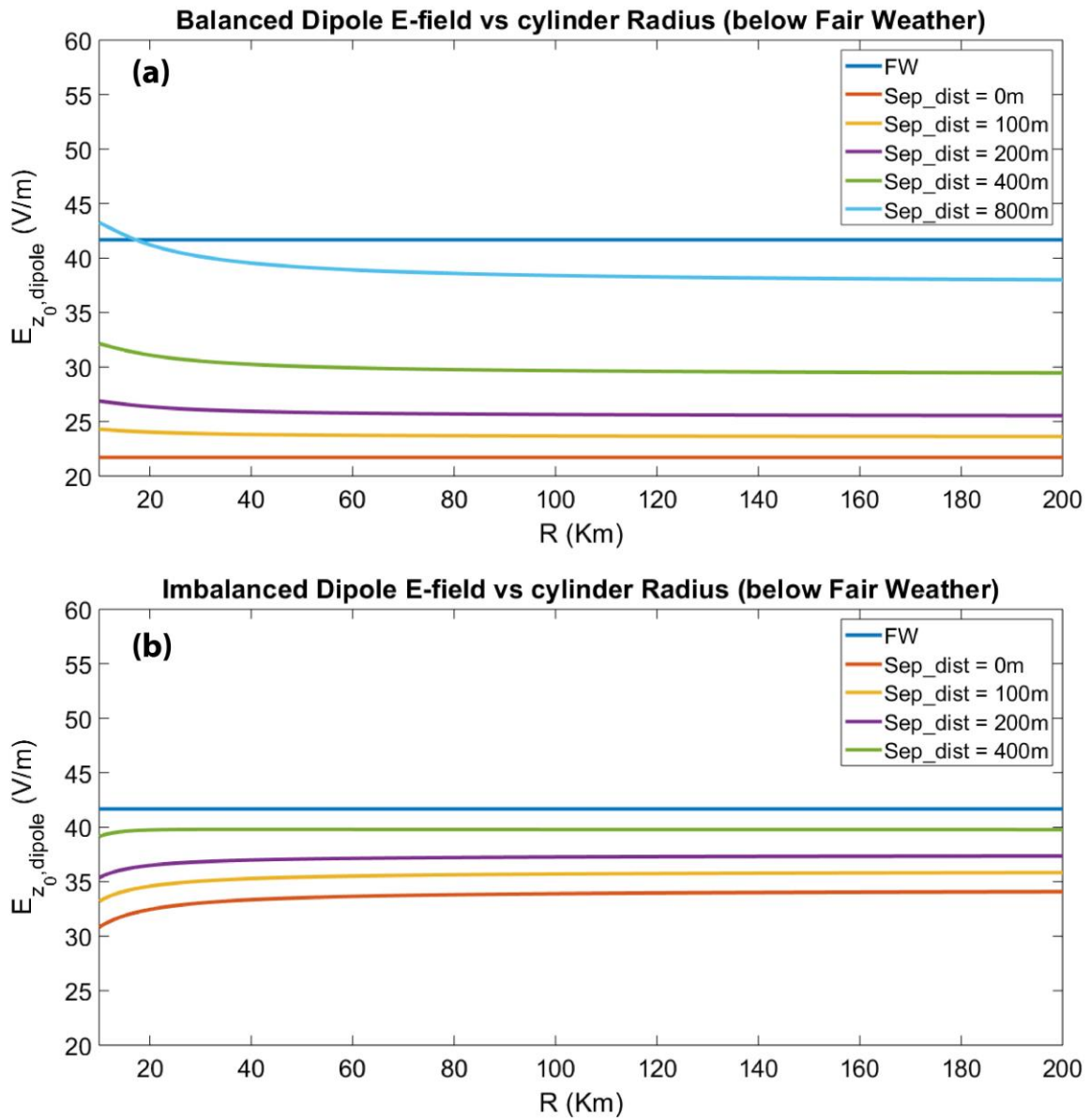
785 Fig. 4. Vertical electric field strength at ground level ( E_{z_0,dipole} ) below the fair weather field (blue line), for a dipole of: (a) finite uniformly charged cylinders and (b) non uniformly charged cylinders exhibiting a charge imbalance of 8%, within an elevated dust layer as a function of the cylinder radius R . E_{z_0,dipole} is calculated for separation distances of 0 (electrically neutral dust), 100, 200, 400 and 800 m (balanced dipole case only) between the charged layers.
