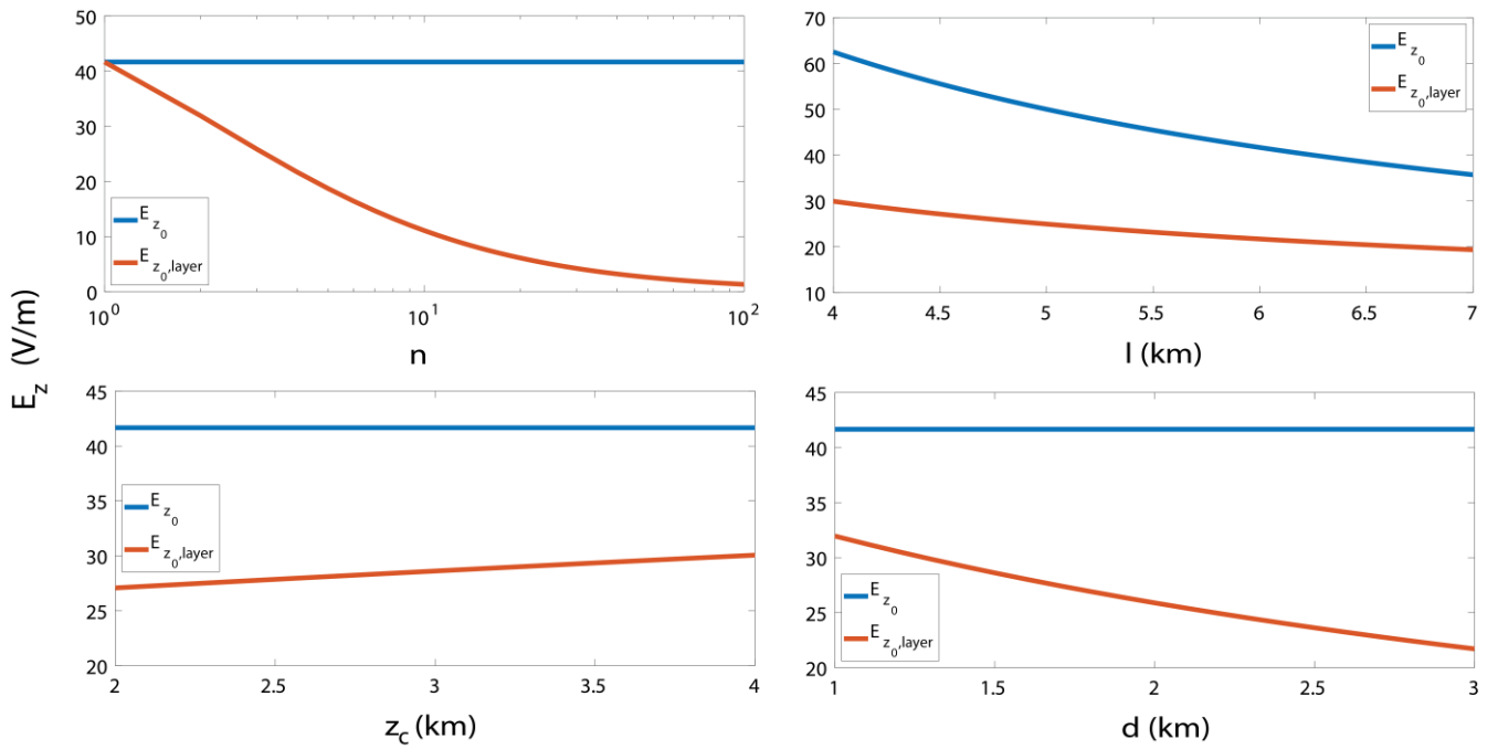
Fig. A1. Dependence of the vertical electric field at ground level, under fair weather ( E_{z_0} , blue line) and under the influence of an uncharged dust layer ( E_{z_0,layer} , red line) on: (a) the reduction factor n , (b) the scaling height l , (c) the central layer height z_c and (d) the dust layer depth d , for 1/\sigma_0 = 3 \cdot 10^{13} \Omega m , V_{ion} = 250 kV and H = 70 km.
