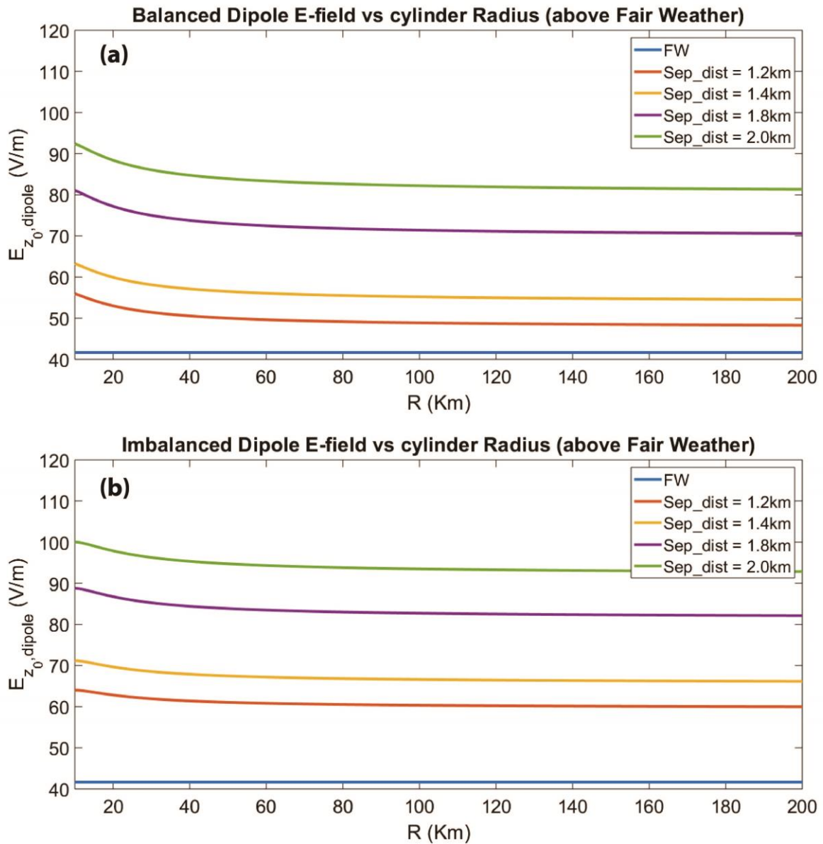
Fig. 5. Vertical electric field strength at ground level ( E_{z_0, \text{dipole}} ) above the fair weather field (blue line), for a dipole of: (a) finite uniformly charged cylinders and (b) non uniformly charged cylinders exhibiting a charge imbalance of 8%, within an elevated dust layer as a function of the cylinder radius R . E_{z_0, \text{dipole}} is calculated for separation distances of 1.2, 1.4, 1.8 and 2 km between the two charged layers.
