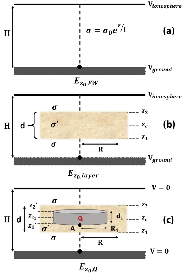
Fig. 3. Schematic of the formalism for the calculation of the steady state near-ground electric field bounded between the ground potential ( V_{ground} ) and ionospheric potential ( V_{ionosphere} ) at height H , under: (a) fair weather conditions ( E_{z_0,FW} ) where atmospheric conductivity \sigma , follows an exponential distribution along the altitude z with respect to the scaling height l , (b) the presence of an electrically neutral dust layer ( E_{z_0,layer} ) with depth d and radius R , which modifies conductivity to \sigma' and (c) the hypothesis of a cylindrical charged monopole ( E_{z_0,Q} ) within the dust layer, with depth d_1 , radius R_1 and total charge Q . The monopole case is a superposition of the electrically neutral dust layer with the charged cylinder within the bounded atmospheric potential.
