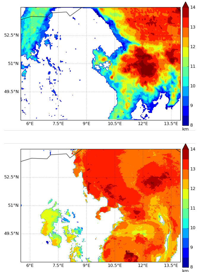
Figure A2. Observed (top) and simulated (bottom) horizontal distribution of CTHs of ice clouds at 22 UTC for 4 July 2015 over Germany. CTHs below 8 km are not shown.
