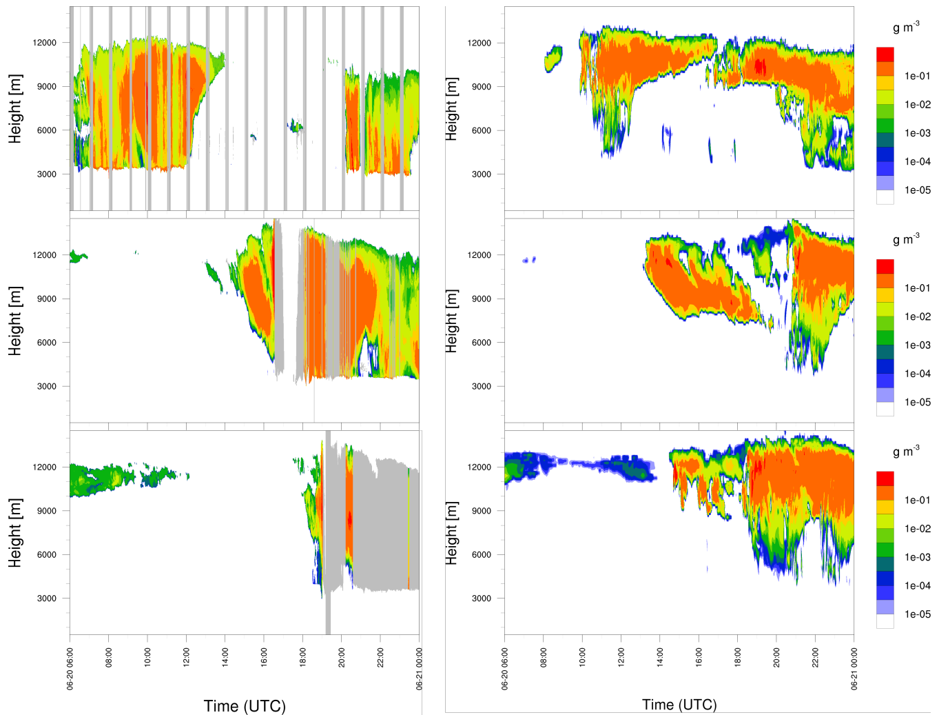
Figure 3. Temporal evolution of ice water content observed by Cloudnet with a 30 s temporal resolution (left) vs. simulated by ICON-LEM (right) for three stations: Jülich (top), Leipzig (middle) and Lindenberg (bottom) for 20 June 2013. Grey shaded areas indicate missing values within the Cloudnet data or points in time where the retrieval could not evaluate ice water content due to falling precipitation. The periodically reoccurring data gaps in the Jülich data are caused by a radar scan every hour in which the antenna is not vertically pointed and thus no Cloudnet retrieval is possible.
