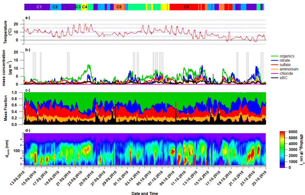
655 Figure 1: Time series of the ambient temperature (a), the particulate near-PM 1 chemical composition as measured by the AMS and completed by MAAP for equivalent black carbon (b), the corresponding mass fraction (c), and particle number size distribution (d) during HCCT-2010 at the site of Goldlauter. The colored bars and numbers at the top refer to the six different air mass clusters (see section 3.4), and the grey bars refer to the different cloud and non-cloud events as defined in Table SI-2.
