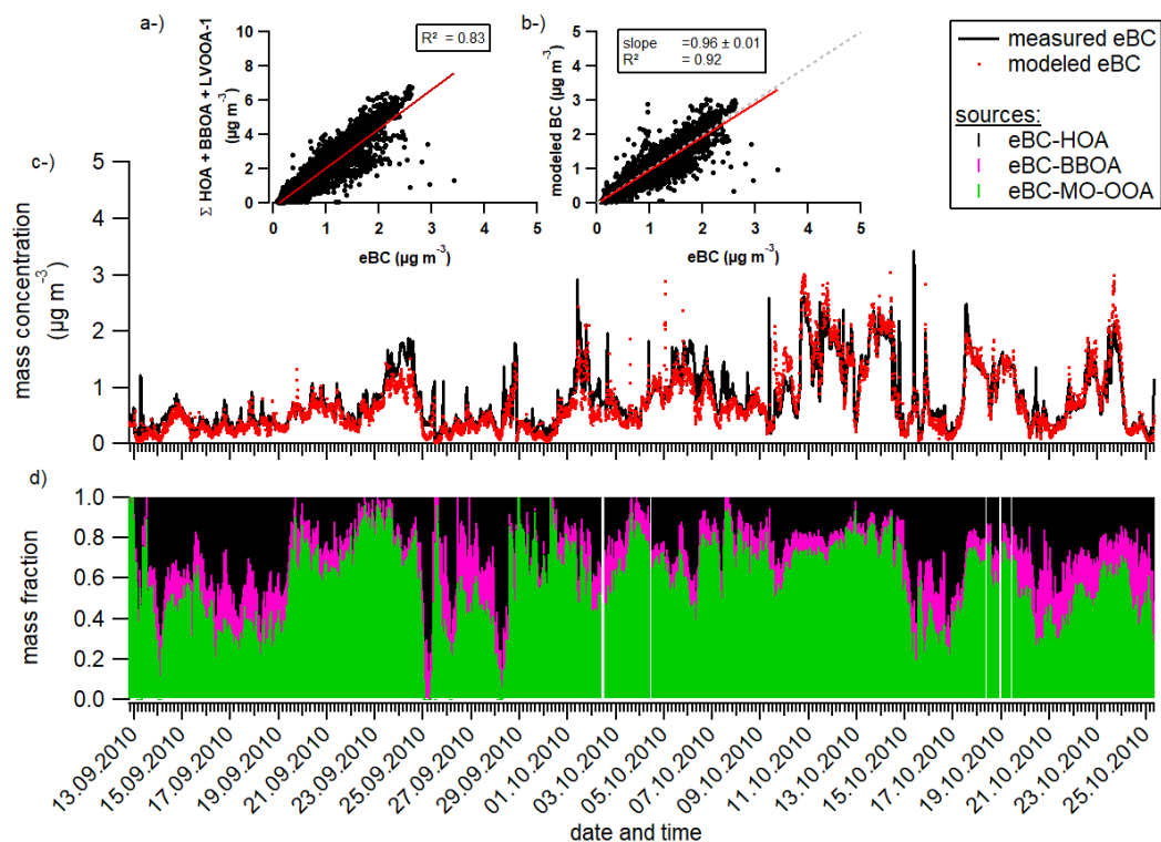
690 Figure 7: Contribution of the different organic factors to the eBC mass concentration. The scatter plots present the correlation between the sum of the OA factors and the measured eBC (a), and the estimated eBC concentration compared to the measured one (b). Time series show comparisons between measured and modeled eBC (c) and contributions of each source to the modeled eBC concentration (d). The correlation curves (red lines) were calculated using the least orthogonal distance fit method.
