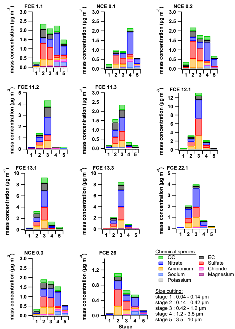
Figure 2: Size distribution of OC, EC, and major water-soluble ions from Berner-impactor measurements for the different events.
