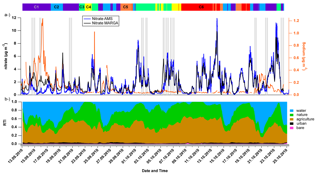
Figure 3: Influence of marine air masses on nitrate size distribution: (a) nitrate mass concentrations measured by AMS and MARGA as well as sodium mass concentrations by MARGA, (b) the residence time index (RTI) of the 96 h backward trajectories above different land cover as developed by van Pinxteren et al. (2010). The colored bars and numbers at the top refer to the 6 different air mass clusters (see section 3.4), and the grey bars refer to the different cloud and non-cloud events as defined in Table SI-2.
