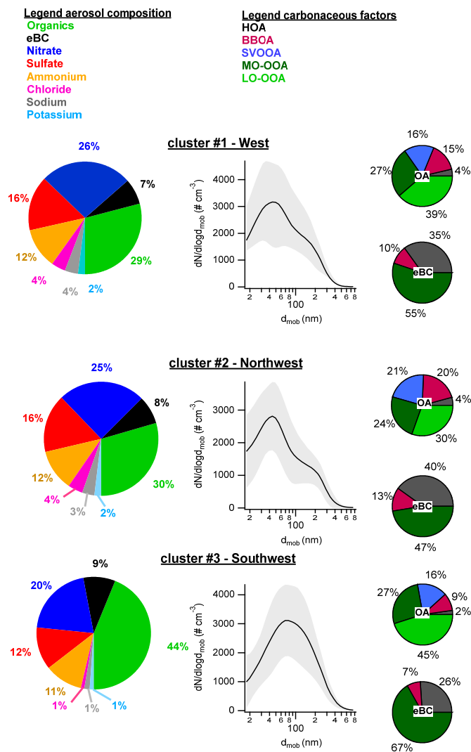
700 Figure 10: Overview of the chemical composition and the PNSD for each cluster: on the left, the mean estimated PM 10 aerosol particle chemical composition; in the middle, the averaged particle number size distribution ( \pm standard deviation in grey); and on the right, the source apportionment results for organic aerosol (top right) and eBC (bottom right).
