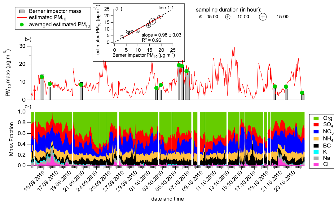
Figure 4: Estimation of the PM 10 mass concentration by combining AMS, MAAP, and MARGA: (a) Comparison with total PM 10 mass concentration measured by Berner-impactors during intensive sampling periods, (b) mass concentration time series, (c) mass fraction of the main components. The size of the point on the scatter plot (a) refers to the sampling duration of the Berner-impactor. The red line in the insert panel represents regression fit by least orthogonal distance fit forced to zero.
