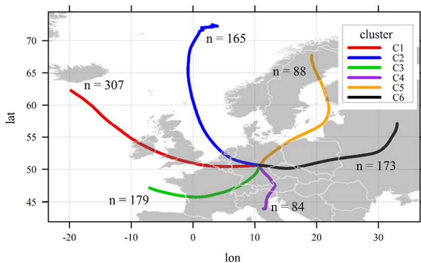
Figure 9: Cluster results of the 96 h backward air mass trajectories calculated for the entire sampling period. The “n” indicates the sum of air mass trajectories associated with each cluster.
