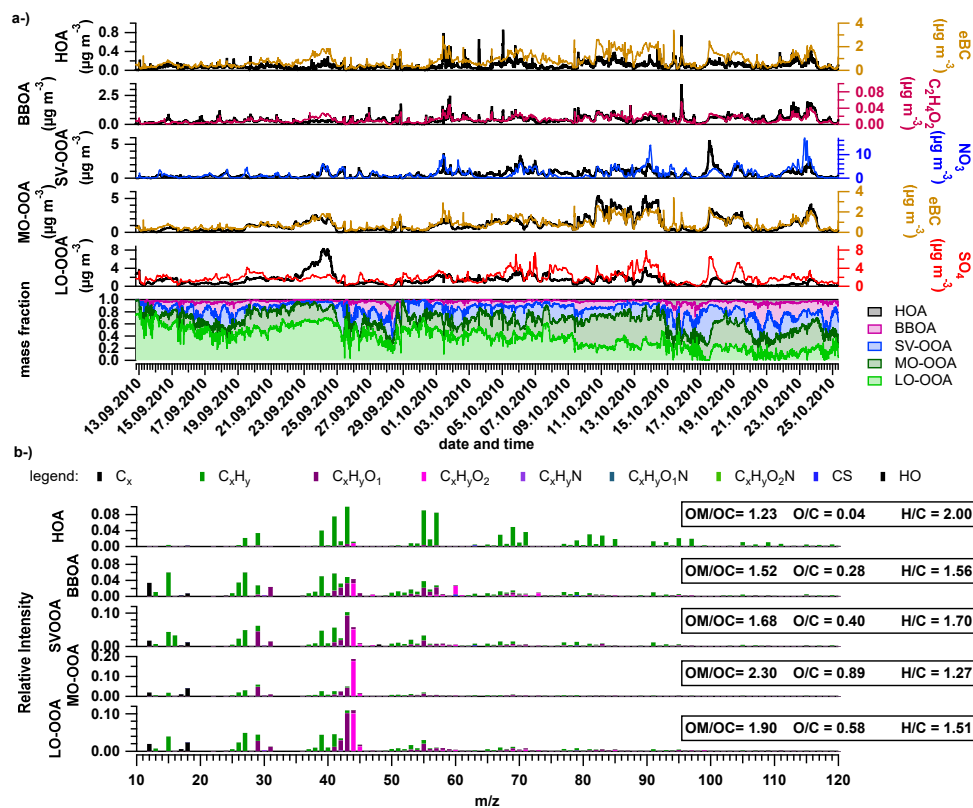
680 Figure 5: Overview of the ME-2 results. a) Time series of the 5-factors solution mass concentration and their corresponding tracers as well as mass fraction of each factor throughout the experiment. b) High-resolution mass spectra colored by the different groups of fragments and the elemental ratios of the identified factors.
