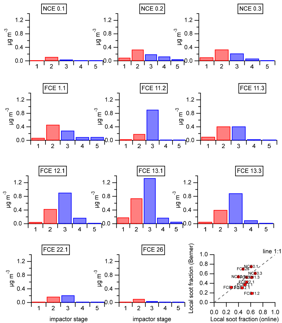
Figure 8: Overview of the EC size distribution measured by the 5-stages Berner impactor. Color corresponds to the following EC classification: red = local and blue = regional/transport. The scatter plot on the bottom right shows the comparison between the local soot fractions estimated using the two different approaches: Berner impactor (y-axis) and on-line multilinear regression (x-axis).
