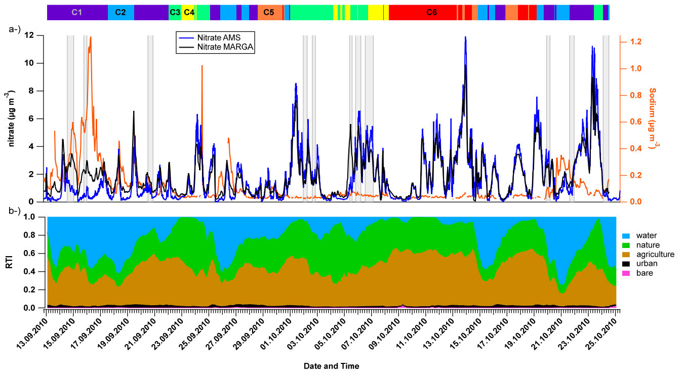
680 Figure 3: Influence of marine air masses on nitrate size distribution: (a) nitrate mass concentrations measured by AMS and MARGA as well as sodium mass concentrations by MARGA, (b) the residence time index (RTI) of the 96 h backward trajectories above different land cover as developed by van Pinxteren et al. (2010). The colored bars and numbers at the top refer to the 6 different air mass clusters (see section 3.4), and the grey bars refer to the different cloud and non-cloud events as defined in Table SI-2.
