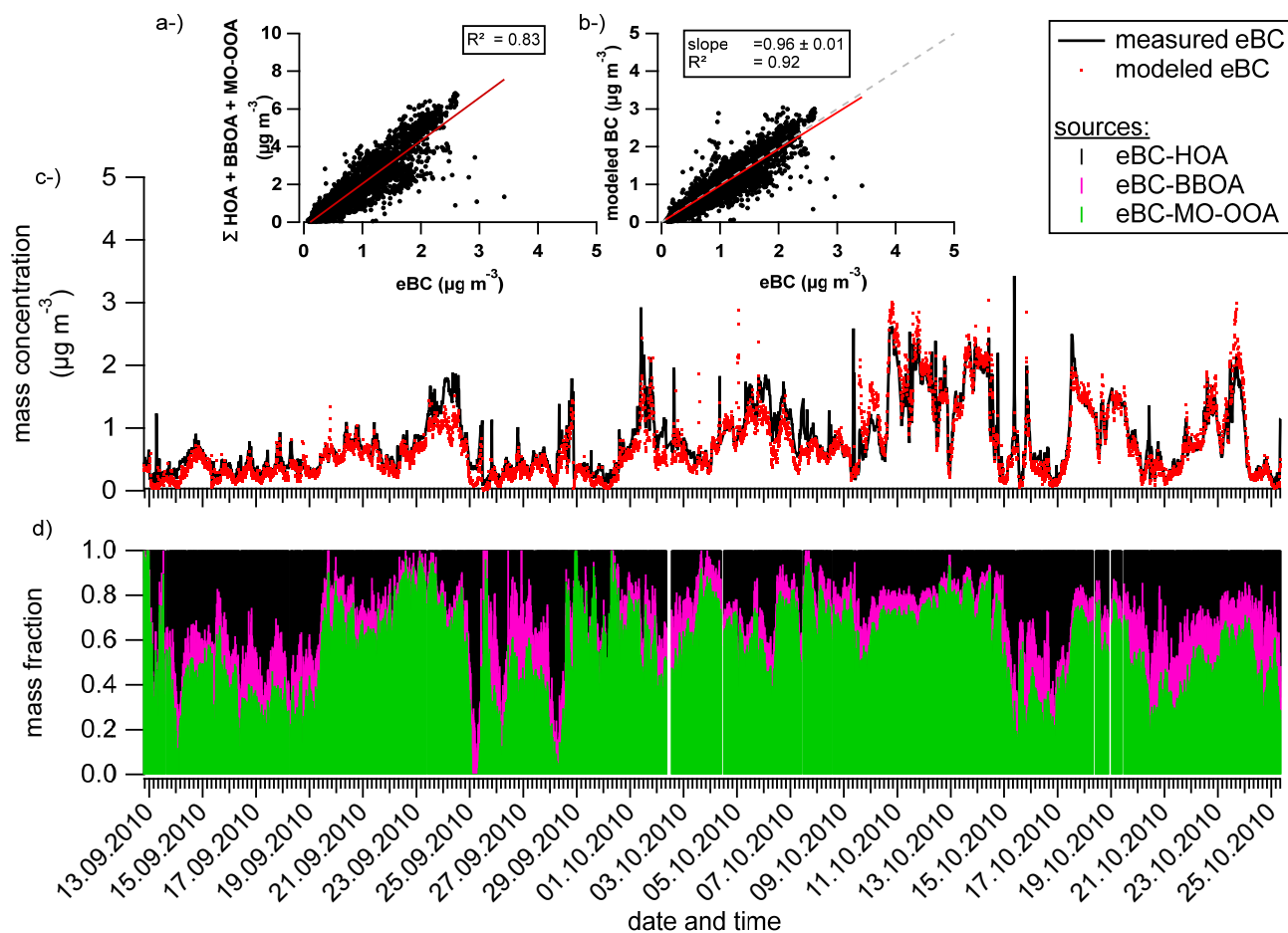
700 Figure 7: Contribution of the different organic factors to the eBC mass concentration. The scatter plots present the correlation between the sum of the OA factors and the measured eBC (a), and the estimated eBC concentration compared to the measured one (b). Time series show comparisons between measured and modeled eBC (c) and contributions of each source to the modeled eBC concentration (d). The correlation curves (red lines) were calculated using the least orthogonal distance fit method.
