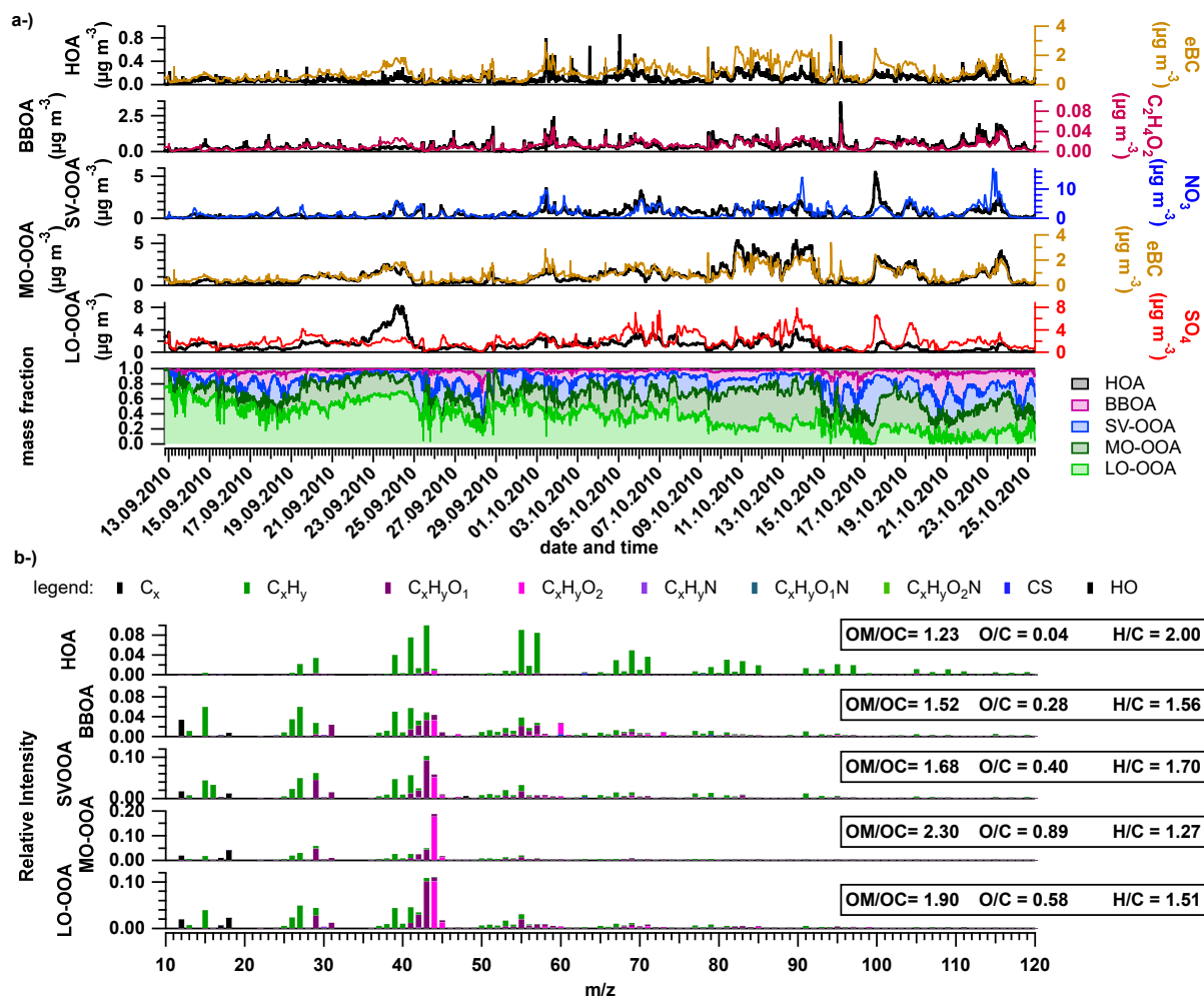
Figure 5: Overview of the ME-2 results. a) Time series of the 5-factors solution mass concentration and their corresponding tracers as well as mass fraction of each factor throughout the experiment. b) High-resolution mass spectra colored by the different groups of fragments and the elemental ratios of the identified factors.
