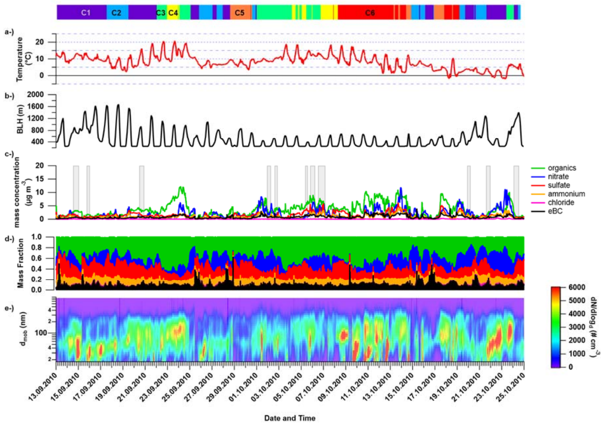
665 Figure 1: Time series of the ambient temperature (a), estimated boundary layer height (BLH) obtained from HYSPLIT GDAS input (b), the particulate near-PM1 chemical composition as measured by the AMS and completed by MAAP for equivalent black carbon (c), the corresponding mass fraction (d), and particle number size distribution (e) during HCCT-2010 at the site of Goldlauter. The colored bars and numbers at the top refer to the six different air mass clusters (see section 3.4), and the grey bars refer to the different cloud and non-cloud events as defined in Table SI-2.
