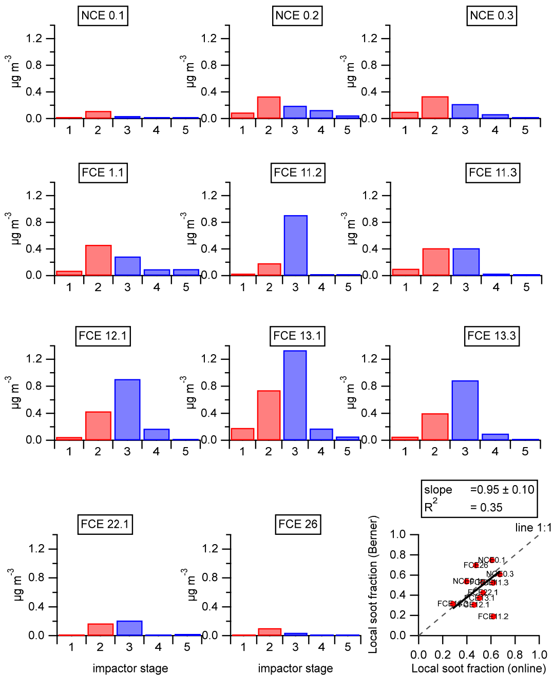
705 Figure 8: Overview of the EC size distribution measured by the 5-stages Berner-impactor. Color corresponds to the following EC classification: red = local and blue = regional/transport. The scatter plot on the bottom right shows the comparison between the local soot fractions estimated using the two different approaches: Berner-impactor (y-axis) and on-line multilinear regression (x-axis). Regression (black line) was made using the least orthogonal distance fit method.
