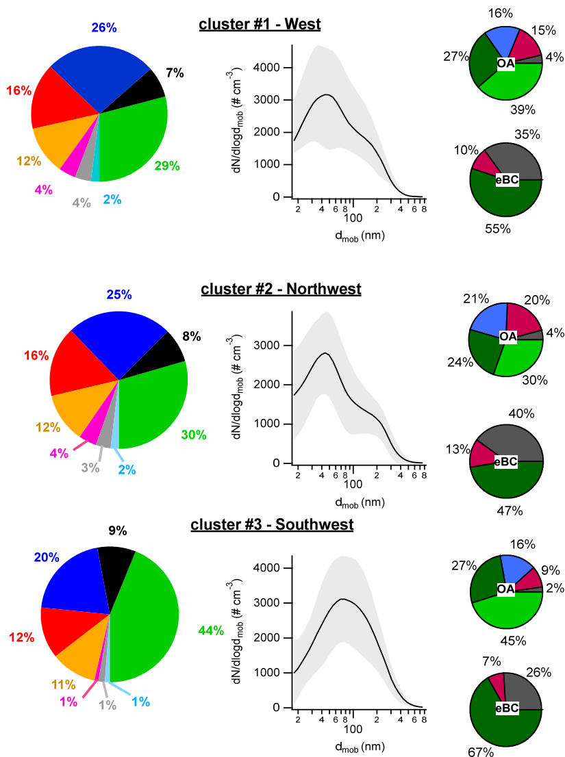
715 Figure 10: Overview of the chemical composition and the PNSD for each cluster: on the left, the mean estimated PM 10 aerosol particle chemical composition; in the middle, the averaged particle number size distribution (± standard deviation in grey); and on the right, the source apportionment results for organic aerosol (top right) and eBC (bottom right).
