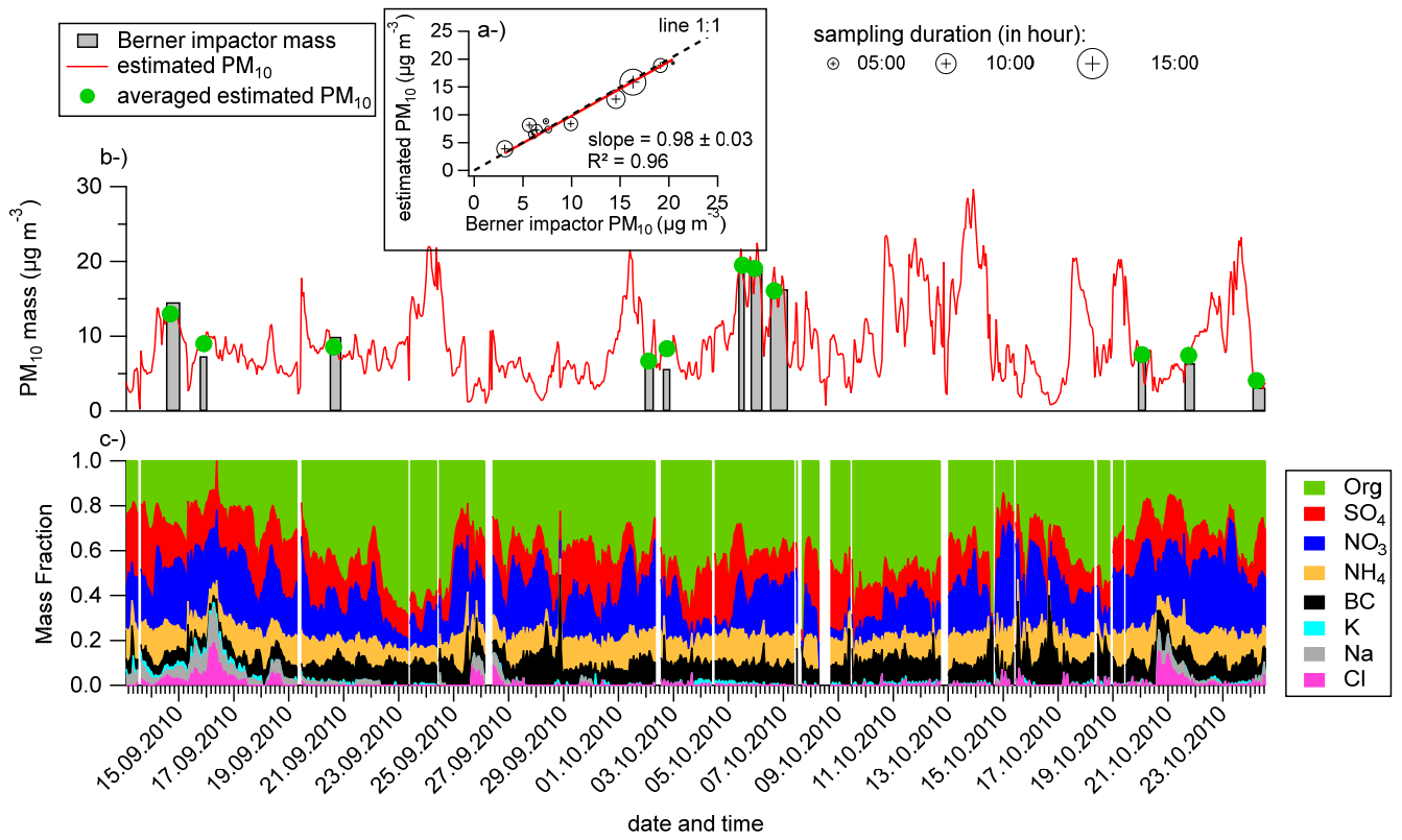
685 Figure 4: Estimation of the PM 10 mass concentration by combining AMS, MAAP, and MARGA: (a) Comparison with total PM 10 mass concentration measured by Berner-impactors during intensive sampling periods, (b) mass concentration time series, (c) mass fraction of the main components. The size of the point on the scatter plot (a) refers to the sampling duration of the Berner-impactor. The red line in the insert panel represents regression fit by least orthogonal distance fit forced to zero.
