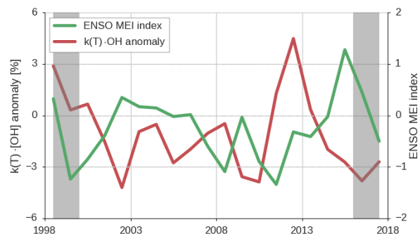
Figure 8. Variations in the annual mean ENSO-MEI index ( left-right axis ) and variations in global, annual mean k(T) \cdot [OH] ( right-left axis ), as derived in the REF inversion. Gray bars indicate a spin-up and spin-down period of 1.5 years.
