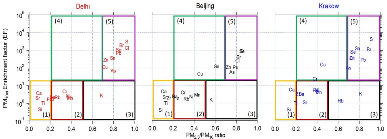
615 Figure 2: Classification of the measured elements in five groups for Delhi, Beijing, and Krakow based on their enrichment factor (EF) vs PM 2.5 /PM 10 values. PM 10 EF vs PM 2.5 /PM 10 values and PM 2.5 EF vs PM 2.5 /PM 10 values for all four sites are shown in Supplementary (Fig. S5).
