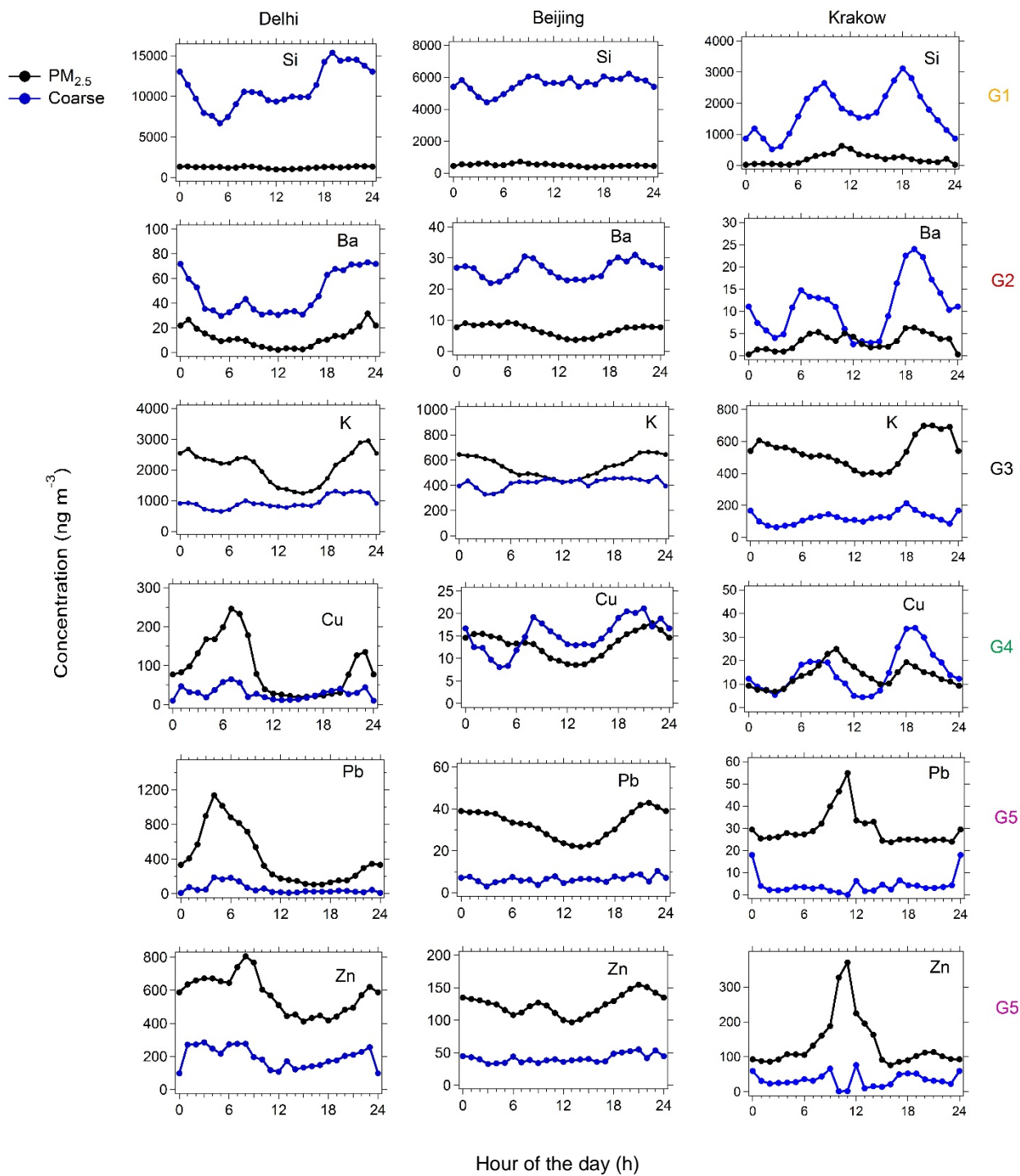
630 Figure 5: Diurnal variations of elements representative of each group (G1: Group 1, G2: Group 2, G3: Group 3, G4: Group 4, G5: Group 5) in PM_{2.5} and coarse size fractions ( PM_{10-PM_{2.5}} ) at Delhi, Beijing, and Krakow (see Fig. S8 for London).
