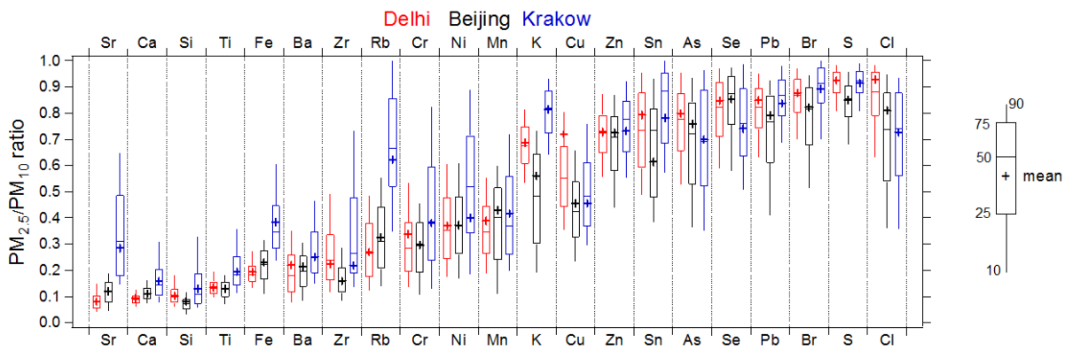
620 Figure 3: Box-whisker plot of the measured elemental PM_{2.5}/PM_{10} ratios at Delhi, Beijing, and Krakow (Fig. S4 is shown for all four sites). Box: First to third quartile range, -: median line, +: mean, whiskers: 10-90% percentiles.
