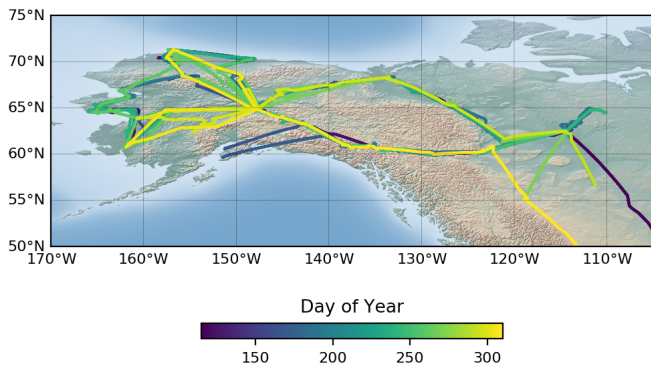
Figure 3 Arctic-CAP flight paths colored by day of year (DOY). Later paths are plotted on top, masking flights from earlier in the year along the same routes. Profile locations span 50-75 °N and 105-165 °W and sampled environmental conditions from the spring thaw (~DOY 125) through the early cold season (> DOY 300) (© Google Maps).
