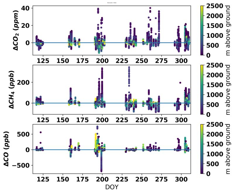
880 Figure 9. Observation-model differences in mole fractions below 3000 masl. Corrections have been made for observation-model offsets above 3000 masl (Fig. 7). Colors show the altitude of each deviation. Dark blue indicates differences near the surface while yellow indicates differences near 3000 masl.
