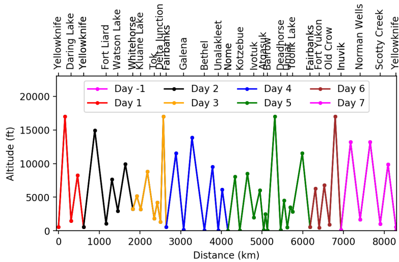
845 Figure 2. Locations and maximum altitudes of the 25 vertical profiles that were acquired during each Arctic-CAP campaign. The colors match the flight lines illustrated in Fig. 1.
