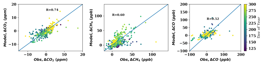
875 Figure 8. Modelled versus observed average boundary layer enhancements or depletions in \text{CO}_2 , \text{CH}_4 and \text{CO} for individual profiles from 3000 masl down to the surface level.
