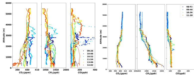
885 Figure 10. Observation (dotted lines) and model estimates (thin lines) of profiles on July 10, 2017 (left) and August 30, 2017 (right) from a transect up the Mackenzie River in the Northwest Territory of Canada. Dotted lines show observations and thin lines show model estimates corresponding to specific times during the transect.
