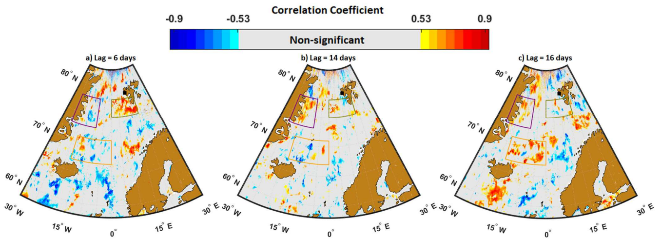
Figure 7: Correlation maps for nINP_{PMI} at T = -15^{\circ}C with (left) 6, (center) 14 and (right) 16 days time lag. The color scale indicates the correlation coefficient; not significant ( p > 0.05 ) pixels are reported in grey. The purple, green and orange boxes highlight sea regions characterized by high correlation at a certain time lag.
