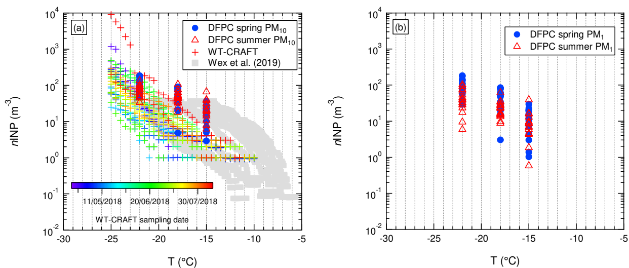
955 Figure 2: Ambient n_{\text{INP}} as a function of the activation T assessed for samples from GVB during 2018 by DFPC and WT-CRAFT. DFPC data are divided in spring (blue) and summer (red) samples, while WT-CRAFT data are color coded according to the sampling date. (a) \text{PM}_{10} (DFPC) and TSP (WT-CRAFT) data. (b) \text{PM}_1 data (available only for DFPC). For comparison purposes, the data from Wex et al. (2019), which refer to \text{PM}_{10} samples, are also reported in plot (a).
