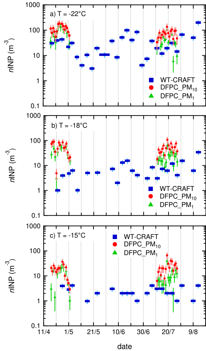
Figure 4: Time series of n_{\text{INP}} at GVB during 2018 measured by DFPC ( \text{PM}_{10} and \text{PM}_1 ) and WT-CRAFT. Horizontal bars indicate the time span of WT-CRAFT samples (ca. 4 days for the majority of samples). Vertical bars indicate the overall measurement uncertainty as indicated in the Sect. 2.
