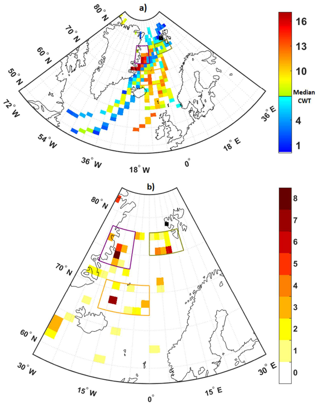
Figure 8. (a) CWT source map for the n\text{INP}_{\text{PM1}} at T = -15^\circ\text{C} dataset. The color scale indicate the CWT value. (b) Spatial distribution of fine INP sources identified by merging the results of the spatio-temporal correlation analysis and of the CWT algorithm. The color scale reflects how many times a given pixel has \text{CWT} \geq \text{median} and significant correlation coefficient by running time lag from 5 to 20 days. The same purple, green and orange boxes of Figure 7 are reported to facilitate the comparison.
