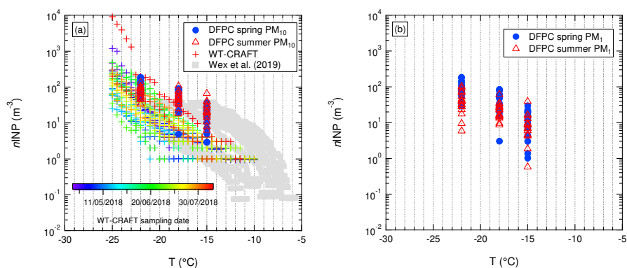
Figure 2: Ambient n_{\text{INP}} as a function of the activation T assessed for samples from GVB during 2018 by DFPC and WT-CRAFT. DFPC data are divided in spring (blue) and summer (red) samples, while WT-CRAFT data are colour-coded according to the sampling date. (a) \text{PM}_{10} (DFPC) and TSP (WT-CRAFT) data. (b) \text{PM}_1 data (available only for DFPC). For comparison purposes, the data from Wex et al. (2019), which refer to \text{PM}_{10} samples, are also reported in the plot (a).
