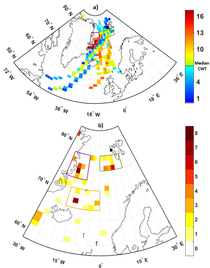
Figure 8. (a) CWT source map for the n\text{INP}_{\text{PM1}} at T = -15^\circ\text{C} dataset. The color scale indicates the CWT value. (b) Spatial distribution of fine INP sources identified by merging the results of the spatio-temporal correlation analysis and of the CWT algorithm. The color scale reflects how many times a given pixel has \text{CWT} \geq \text{median} and significant correlation coefficient by running time lag from 5 to 20 days. The same purple, green and orange boxes of Figure 7 are reported to facilitate the comparison.
