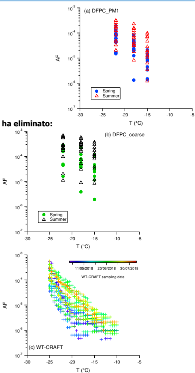
Figure 3: AF as a function of T assessed for samples from GVB during 2018 by DFPC in sub-micrometer (a) and coarse (b) size ranges and by WT-CRAFT (c). Particle size ranges used to calculate AF are 0.1-1 \mu\text{m} , 0.1-10 \mu\text{m} and 0.1-10 \mu\text{m} for DFPC PM 1 , DFPC PM 10 and WT-CRAFT samples, respectively.
