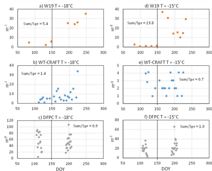
Figure S3. Seasonal evolution of nINP in this study (GVB, 2018) compared to the results by Wex et al. (2019), here indicated as W19, obtained at GVB in spring-summer 2012.
