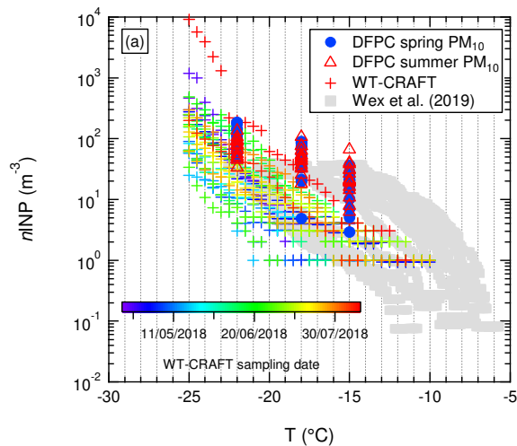
Figure 2: Ambient n_{\text{INP}} as a function of the activation T measured at GVB during 2018 by DFPC and WT-CRAFT. DFPC data are divided in spring (blue) and summer (red) samples, while WT-CRAFT data are color coded according to the sampling date. (a) \text{PM}_{10} (DFPC) and TSP (WT-CRAFT) data.
