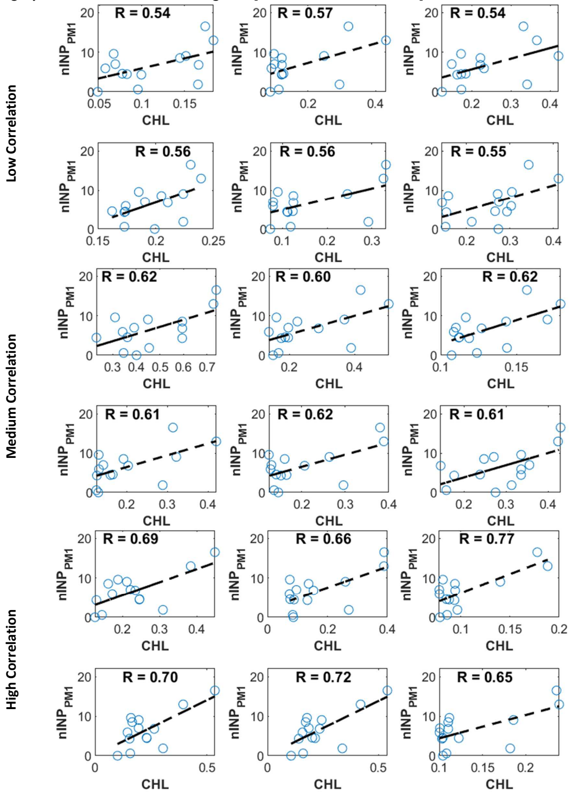
Figure A2: Same as Figure A1, but for seawaters close to the Greenland coast.
