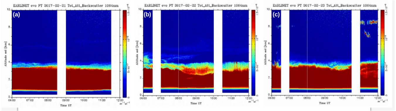
Figure 10. Quicklook images corresponding to the total attenuated backscatter at 1064 nm observed with the EARLINET Évora lidar for the 21 st (panel a), the 22 nd (panel b) and the 23 rd (panel c) of February 2017 show nicely the evolution of this particular dust event ( https://quicklooks.earlinet.org/ ) (Blue colors indicate weak backscattering signal and yellow and red colors indicate higher backscattering signal)
