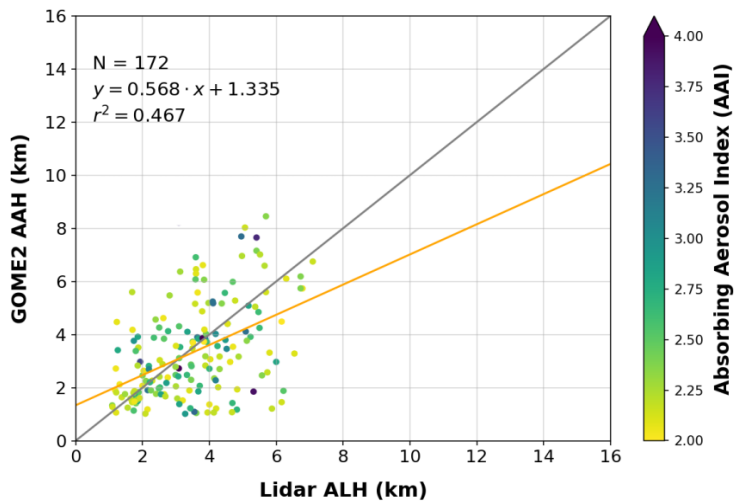
Figure 9. Scatterplot between GOME-2 AAH and aerosol layer height from EARLINET stations, for the total of collocated cases. The associated AAI value is color-coded.
