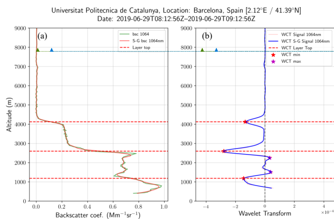
Figure 2. Barcelona lidar station (Universitat Politecnica de Catalunya, Barcelona – UPC): (panel a) Lidar backscatter profile at 1064nm and (panel b) resulting WCT profile on June 29, 2019. The horizontal red dashed line represents the detected aerosol layer top applying the WCT methodology. The label “S-G” indicates that a Savitzky-Golay filter was used to reduce to noise variance in the backscatter profile. The colored “star” symbols represent the local maxima (purple) and minima (red) of wavelet transform signal.
