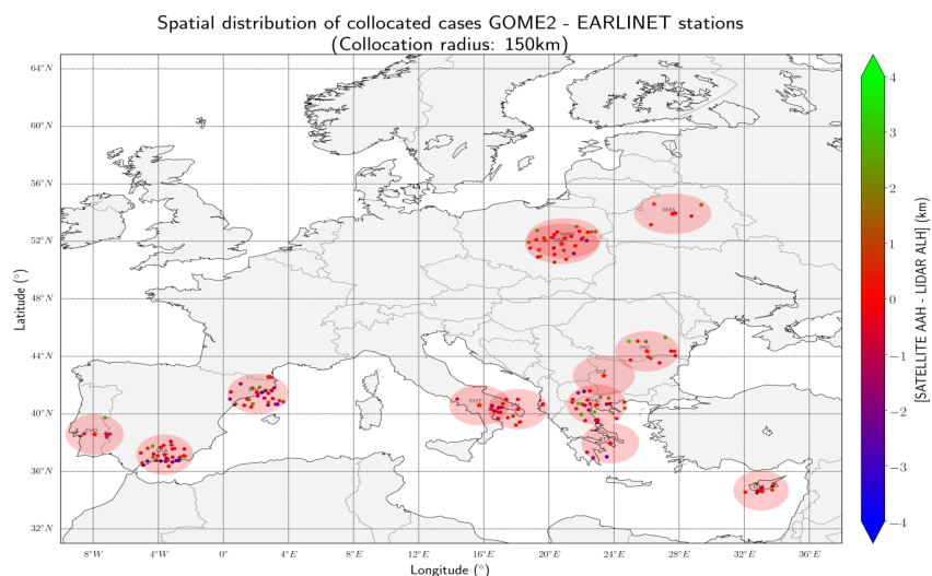
Figure 5. Spatial distribution of collocated pairs between GOME-2/MetOp and EARLINET stations for the sites including in the validation study. The color-codes denote the absolute difference between GOME-2/MetOp AAH and the retrieved aerosol height from EARLINET data for each collocated pair. The concentric red circles denote regions of 150 km from the location of EARLINET stations refer to Table 2 for the EARLINET code names shown in the legend.
