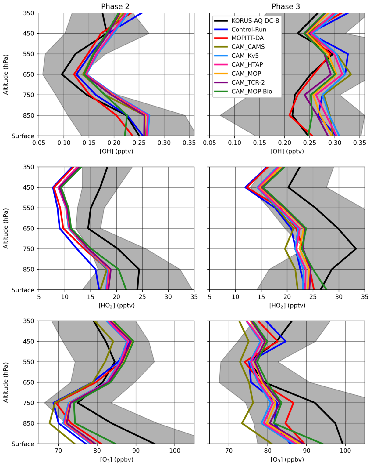
Figure 9: Average LaRC box model OH and HO 2 and measured O 3 for phase 2 (left column) and phase 3 (right column) of KORUS-AQ.
