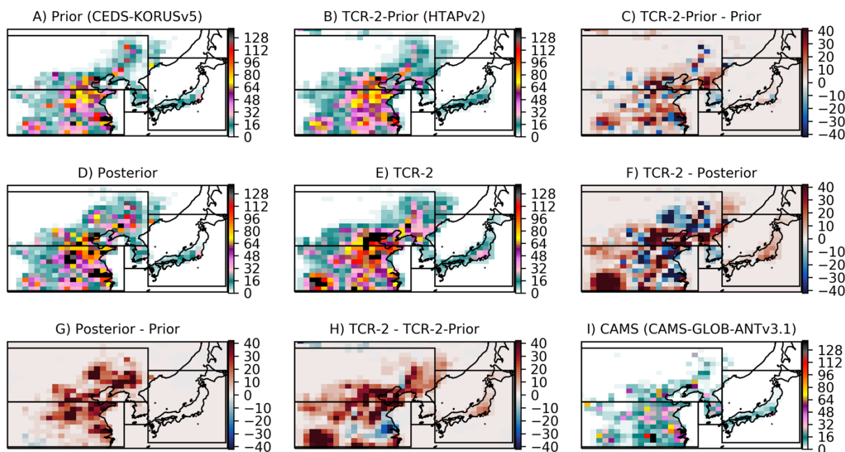
640 Figure 5: Emissions flux for May 2016 in \text{MgCO}\cdot\text{month}^{-1} . Prior (A, CEDS-KORUS v5), TCR-2-Prior (B, HTAP v2) and the difference between the 2 priors (C, TCR-2-Prior – Prior). The second row shows the Posterior (D, estimated by DART/CAM-Chem), the TCR-2 (E) and the difference between the 2 posteriors. The last row shows the emissions increments, the difference between the Posterior and the Prior (G) and between TCR-2 and TCR-2-Prior (H). The CAMS emissions are shown on the last panel (I). 645
