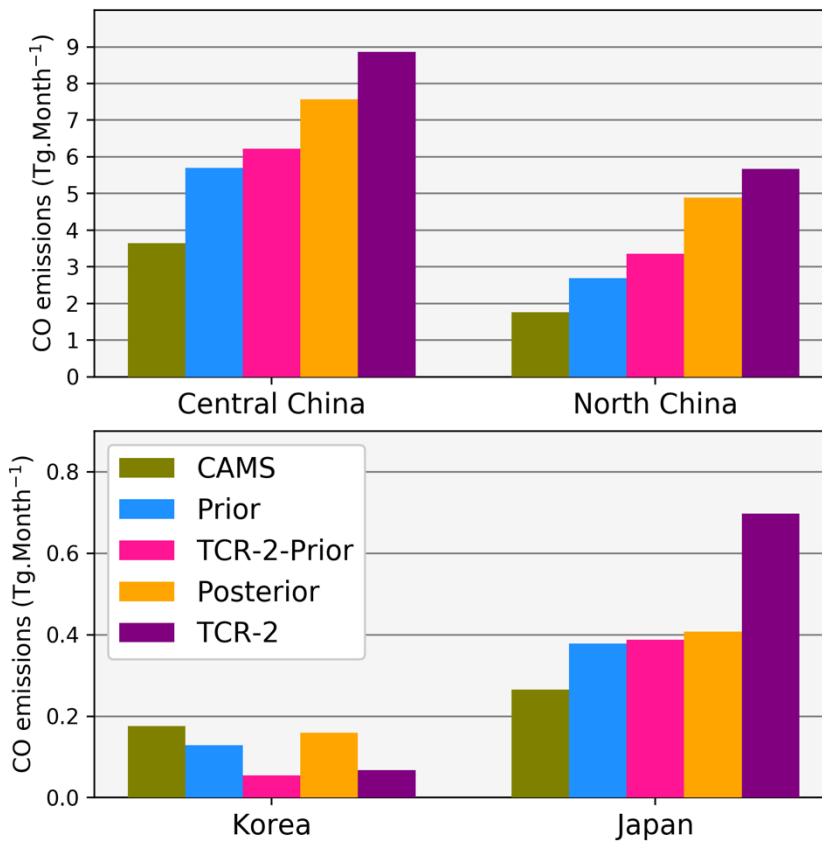
695 Figure 6: Anthropogenic CO emissions for May 2016 for Central China (91E, 29N to 124E, 38N), North China (91E, 38N to 130E, 49N), South Korea (125E, 33.5N to 129E, 38N) and Japan (130E, 30N to 146E, 44N).
