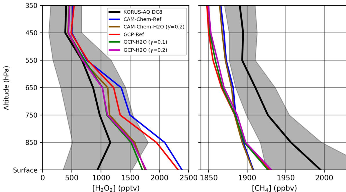
Figure B1: Average \text{H}_2\text{O}_2 profiles (left panel) and \text{CH}_4 profiles (right panels) for all KORUS-AQ. The mean (black line) and standard deviation (shaded grey) of the DC-8 observations are calculated for each 100 hPa bins and only the mean is shown for model simulations.
