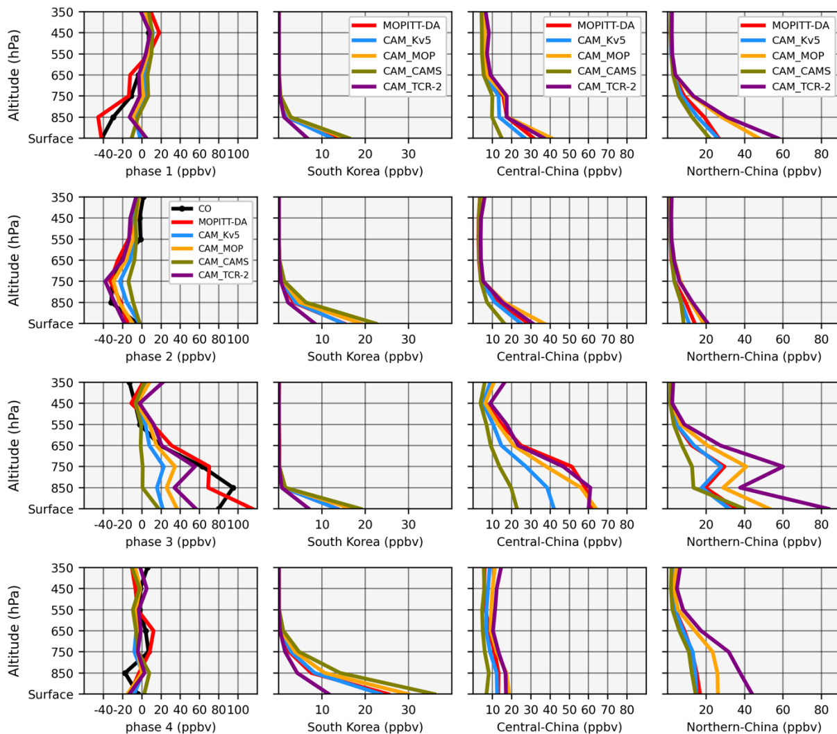
785 Figure 8: Average CO anomalies for the four different phases of KORUS-AQ (first column). The anomaly is defined by subtracting the respective average vertical profile (see Fig. 2). Absolute vertical profiles of the CO
