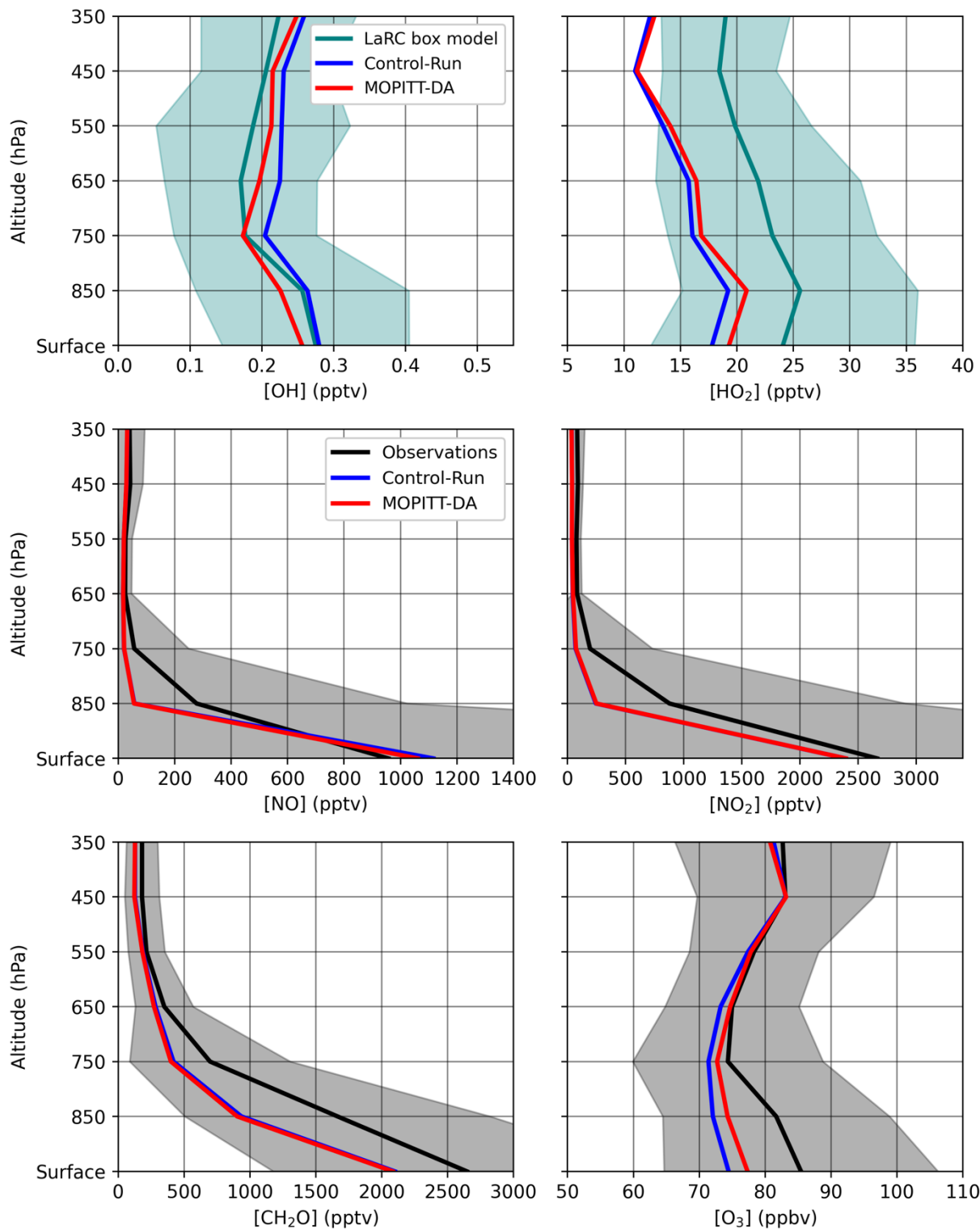
630 Figure 4: Average vertical profiles of OH (top left) HO 2 (top right) for the 1-sec merge and the LaRC box model estimates (Schroeder et al., 2020). Results are shown for DC-8 1-min merge observations for NO (middle left), NO 2 (middle right), CH 2 O (bottom left) and O 3 measurements (bottom right). The shaded area corresponds to the standard-deviation around the observed mean.
