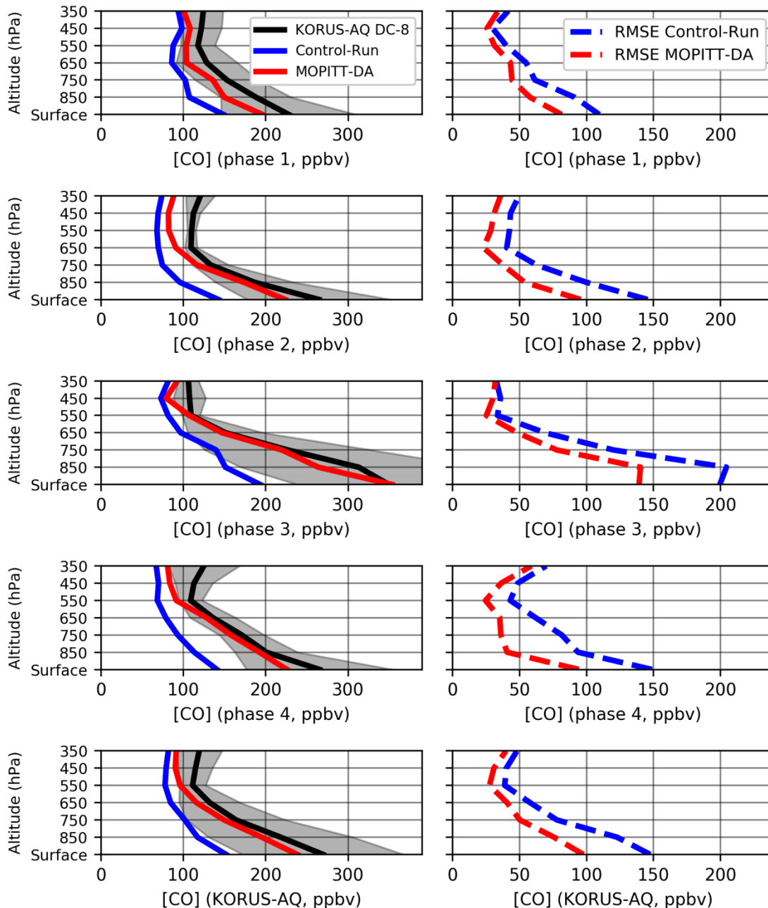
540 Figure 2: Average CO profiles (left panels) and related RMSE (right panels) for the Control-Run and the MOPITT-DA. The mean (black line) and standard deviation (shaded grey) of the DC-8 observations are calculated for each 100 hPa bin. The first 4 rows are averaged over the different weather regimes of the campaign (Peterson et al. 2019). The last row displays the average over the whole campaign.
