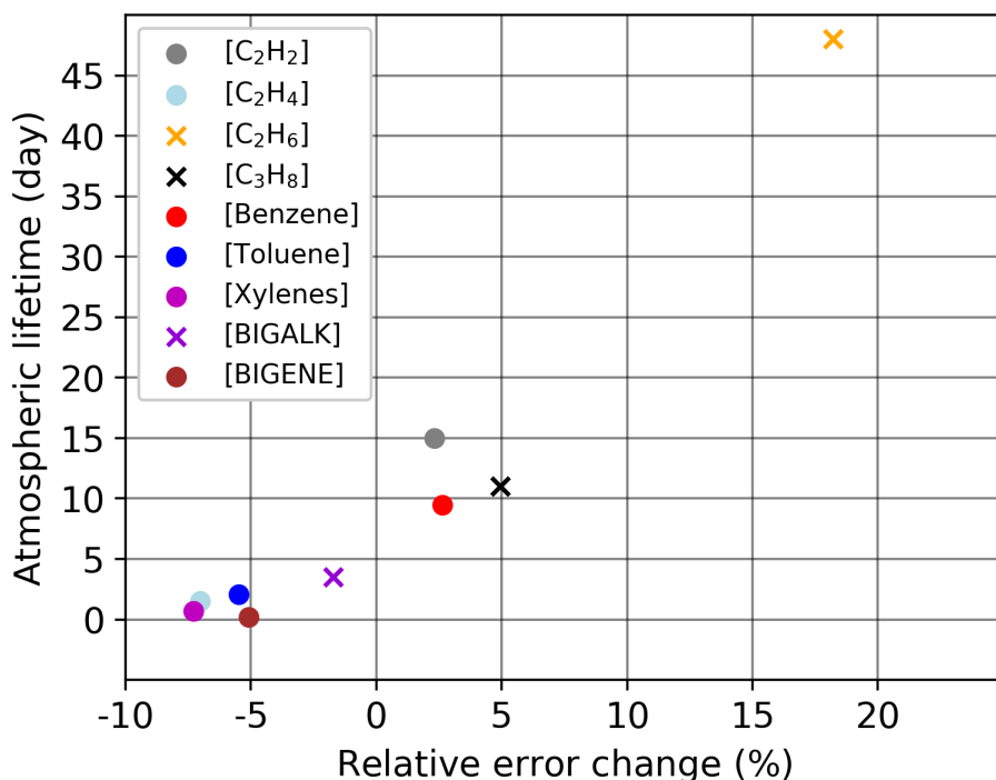
590 Figure 3: Atmospheric lifetime (from Simpson et al., 2020) in days for the VOCs added to the state vector. Xylenes, BIGALK and BIGENES are surrogate species, so an average of the lifetimes is calculated. The relative error change is the opposite of the difference in Root Mean Square Error relative to the Control-Run (i.e., (Control-Run-MOPITT-DA)/Control-Run). Thus, a positive relative error change means an improvement compared to the Control-Run.
