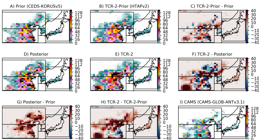
Figure 5: Emissions flux for May 2016 in \text{MgCO}\cdot\text{month}^{-1} . Prior (A, CEDS-KORUS v5), TCR-2-Prior (B, HTAP v2) and the difference between the 2 priors (C, TCR-2-Prior - Prior). The second row shows the Posterior (D, estimated by DART/CAM-Chem), the TCR-2 (E) and the difference between the 2 posteriors. The last row shows the emissions increments, the difference between the Posterior and the Prior (G) and between TCR-2 and TCR-2-Prior (H). The CAMS emissions are shown on the last panel (I).
