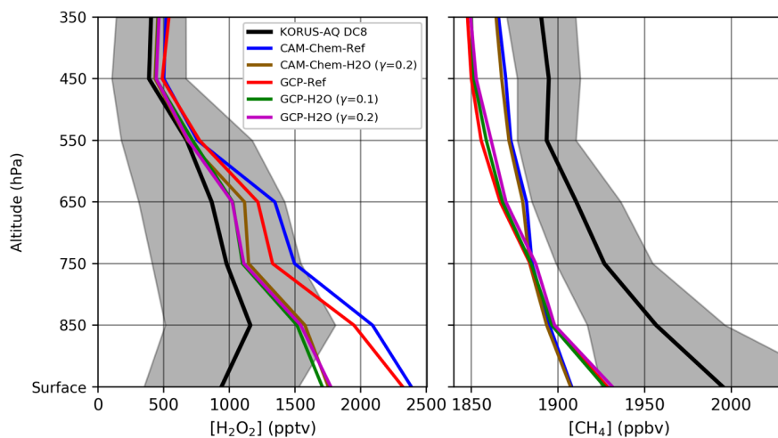
Figure B1: Average \text{H}_2\text{O}_2 profiles (left panel) and \text{CH}_4 profiles (right panels) for all KORUS-AQ. The mean (black line) and standard deviation (shaded grey) of the DC-8 observations are calculated for each 100 hPa bins and only the mean is shown for model simulations.
