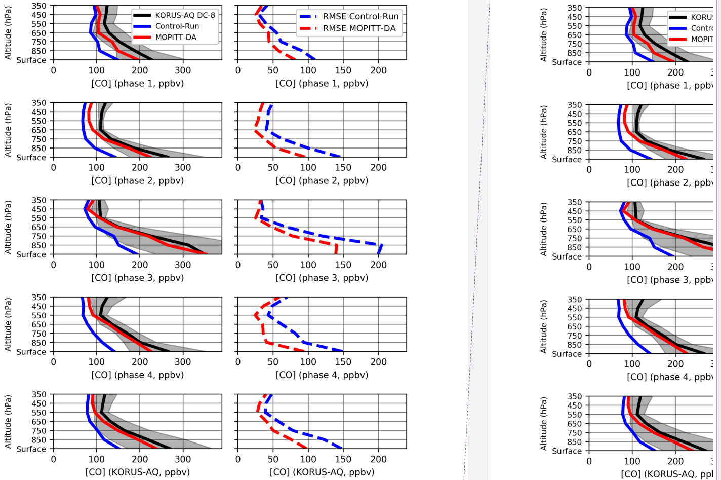
Figure 2: Average CO profiles (left panels) and related RMSE (right panels) for the Control-Run and the MOPITT-DA. The mean (black line) and standard deviation (shaded grey) of the DC-8 observations are calculated for each 100 hPa bin. The first 4 rows are averaged over the different weather regimes of the campaign (Peterson et al. 2019). The last row displays the average over the whole campaign.
