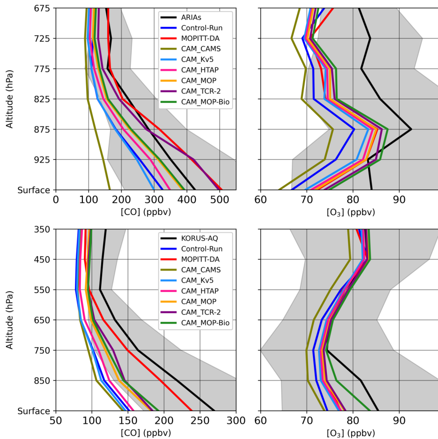
Figure 7: Average CO vertical profiles for the ARIAs campaign (top panel) and the KORUS-AQ (bottom panel). Observations were filtered out when SO 2 was higher than 20 ppbv for ARIAs and benzene higher than 1 ppbv for KORUS-AQ. The black line shows the observation mean and the shaded area is the observation standard deviation. Only mean CO or O 3 are shown for the model simulations.
