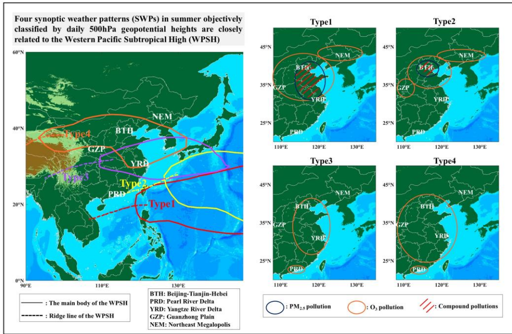
Fig. 1214. Schematic diagrams describing the relationships between the WPSH, four SWPs and summertime O 3 and PM 2.5 pollution in various regions.
