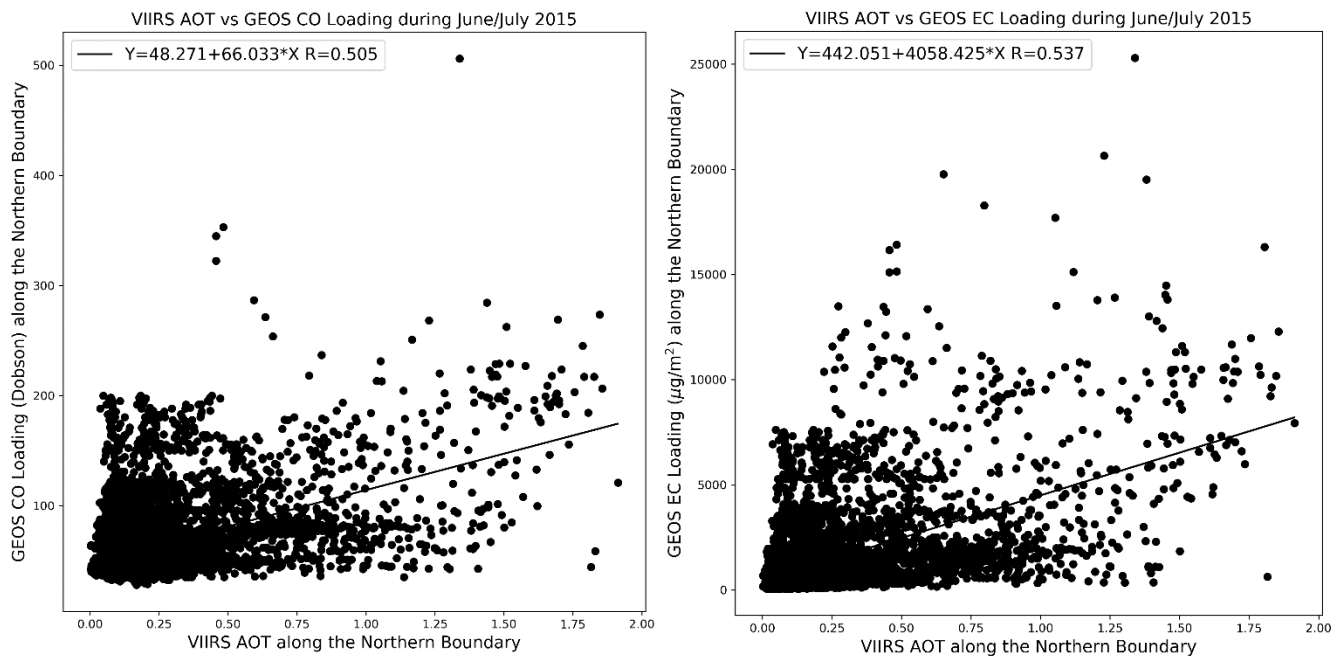
Figure S3. Correlations between AOT/CO (left) and AOT/EC (right) along the Northern Boundary of the CONUS domain during June and July 2015.
