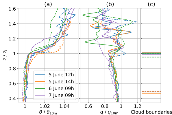
Figure 5. Balloon-borne vertical profiles of (a) potential temperature \theta , (b) specific humidity q and (c) cloud boundaries for four ascents (solid lines) and descents (dashed lines) on 5, 6, and 7 June 2017. The altitude z is normalized to the temperature inversion base height z_i . Potential temperature \theta and the specific humidity q are normalized to their near-surface values. The cloud top is derived from the irradiance profile, the cloud base is derived from Cloudnet data. The profiles are named after the start time (cf. Fig. 2).
