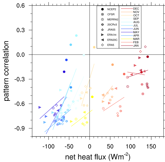
Figure 4: Net heat flux averaged over sea ice zone (x-axis: Wm -2 , where positive indicates net flux from atmosphere to ocean), against the pattern correlation between reanalysis SIC and Sat (i.e. values plotted in Figure 3b). Data points are colored by month with different markers for each reanalysis. Colored lines show the best-fit line for each month estimated by Ordinary Least Squares regression.
