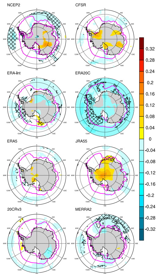
Figure 5: Panels a-h) 1980-2010 December-January mean reanalysis SAT trends over the climatological sea ice zone ( ^{\circ}\text{C}/\text{year} ); only trends that are statistically-significant at the 90% level are shown. Hatched regions show where the sign of statistically-significant reanalysis SIC and SAT trends are the same (i.e. the unexpected result of both a warming (cooling) and an increase (decrease) in sea ice cover). The magenta line shows climatological sea ice edge.
