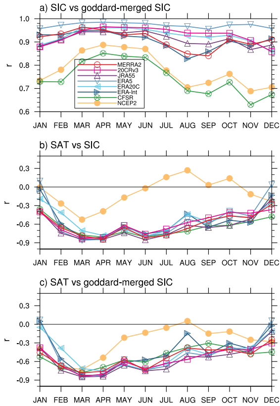
505 Figure 3: Uncentered pattern correlations by month between 1980-2010 SIC and SAT trends: a) correlations between the observed SIC trend and each reanalysis' SIC; b) correlations between each reanalysis SAT trend that reanalysis' SIC trend; c) correlation between reanalysis SAT trend and observed SIC trend. Differences between each reanalysis SIC and the Goddard merged SIC product for each month are shown in the Supplemental Material as Figures S13-S24.
