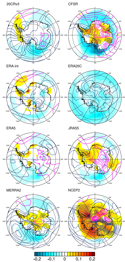
495 Figure 1: 1980-2010 trends in annual-mean SAT (shading: °C/year) and MSLP (contour lines: positive trends in blue, negative trends in magenta, with contour spacing = 2.5 Pa/year), for eight individual reanalyses (refer to Table 1 for details). Trend patterns for each month are shown in the Supplemental Material as Figures S1-S12.
