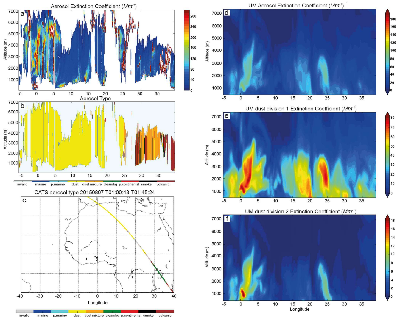
1060 Figure 17: (a-c) CATS and (d-f) MetUM data for 00z on the 7 th August, in the form of vertical cross-sections along the satellite track: (a) CATS extinction coefficient; (b) CATS feature type; (c) CATS overpass track; (d) MetUM total dust extinction coefficient; (e) MetUM d1 dust extinction coefficient; and (f) MetUM d2 dust extinction coefficient.
