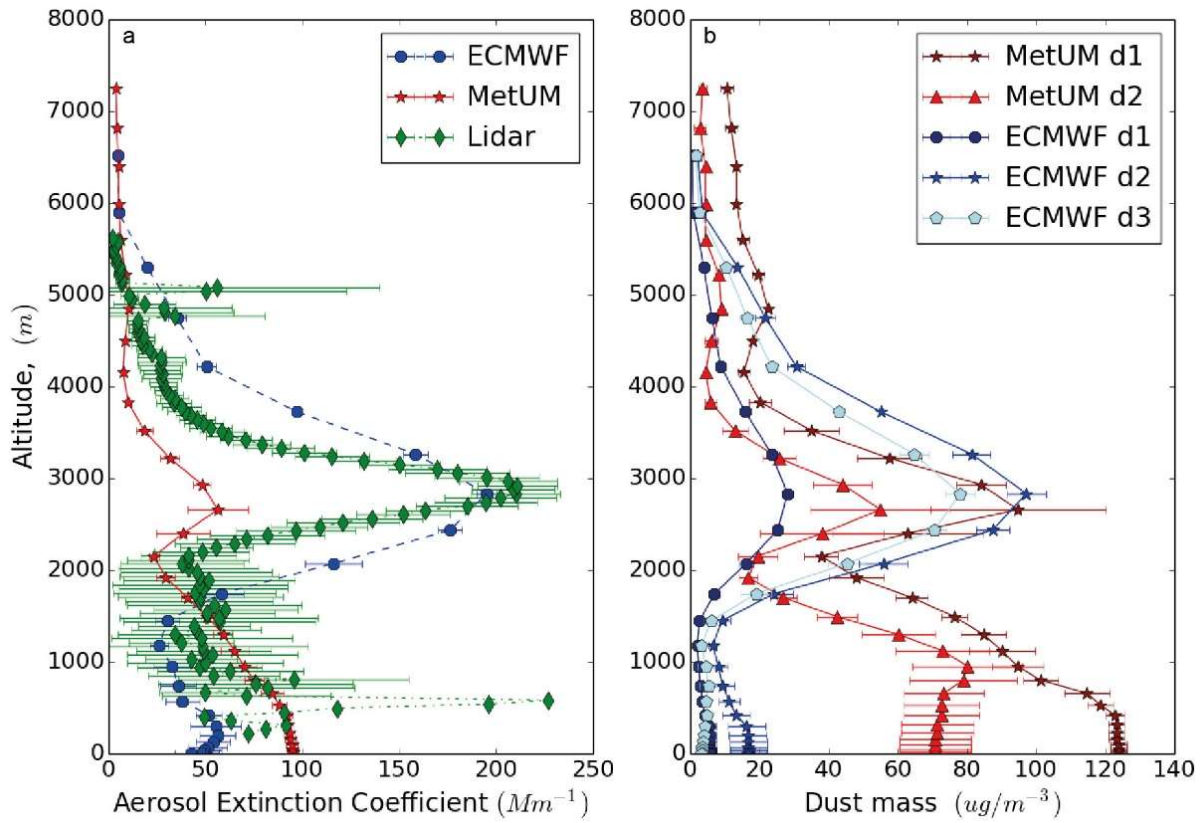
1035 Figure 13: Case Study 3: B927, 15 th August, R1: (a) Mean and standard deviation of the lidar (green), MetUM (red) and ECMWF (blue) extinction profiles. (b) Modelled MetUM dust concentration for divisions 1 (dark red) and 2 (red), and modelled ECMWF concentration for divisions 1 (dark blue), 2 (blue) and 3 (light blue) dust concentration.
