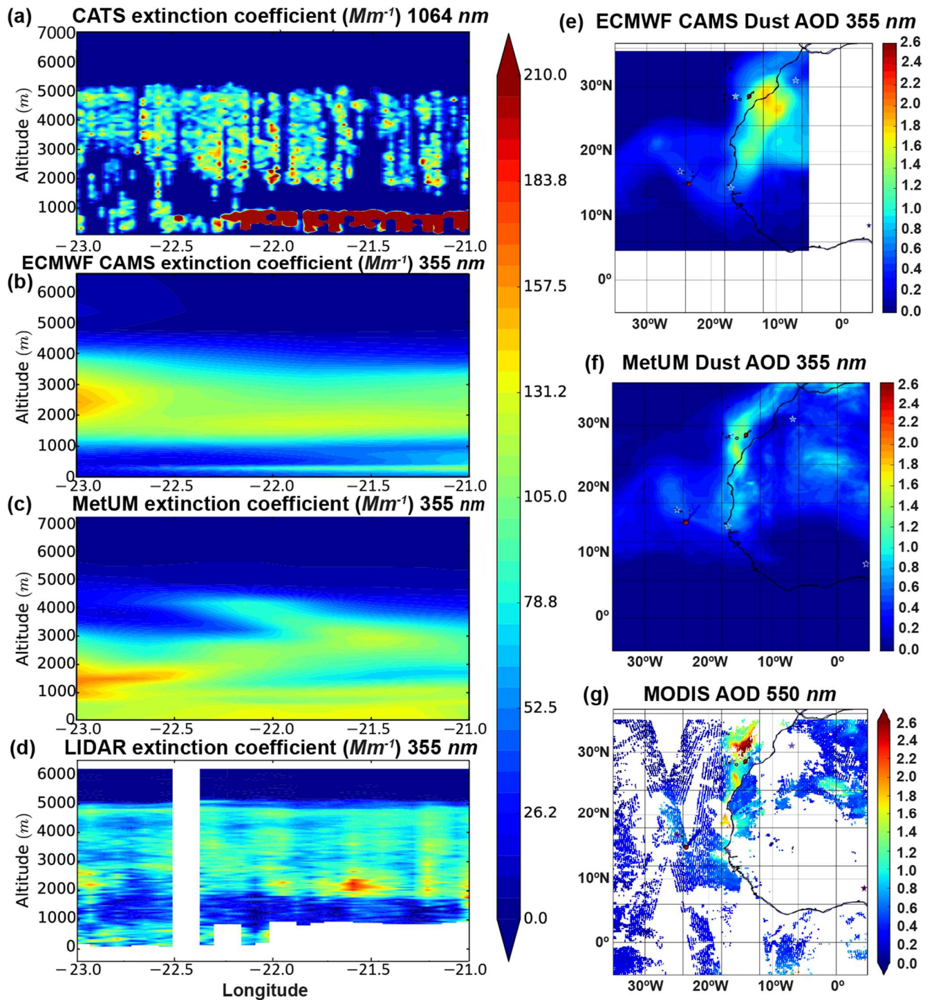
965 Figure 3: Case study 1, B920, 7 th August, R6: (a-d) Vertical cross –section along the flight track showing the aerosol extinction coefficient for the CATS lidar (a), ECMWF CAMS (b), MetUM (c) and the aircraft lidar (d), the colour scale is the same for all four plots. (e) ECMWF AOD map, (f) MetUM AOD map and (g) AOD map from combined observations from MODIS, AERONET (stars) and aircraft lidar (dots).
