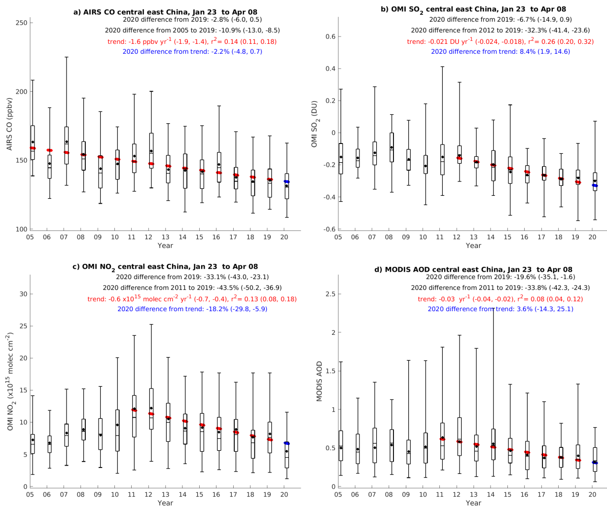
Figure S1. Same as Figure 5, but when daily values are calculated from the median of individual retrievals over central east China, rather than the mean.
