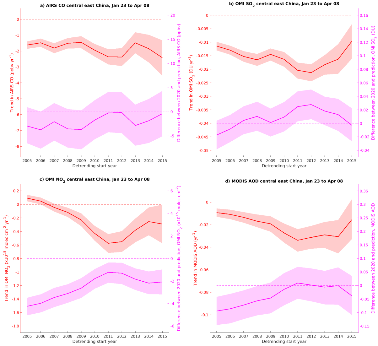
Figure S2. Same as Figure 7, but when daily values are calculated from the median of individual retrievals, rather than the mean.
