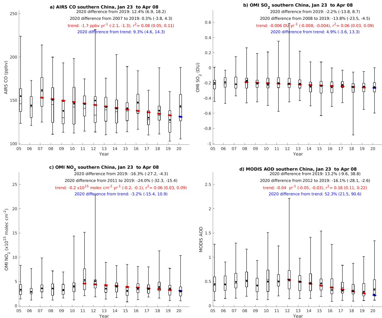
Figure S3. Same as Figure 7, but when daily values are calculated from the median of individual retrievals, rather than the mean.
