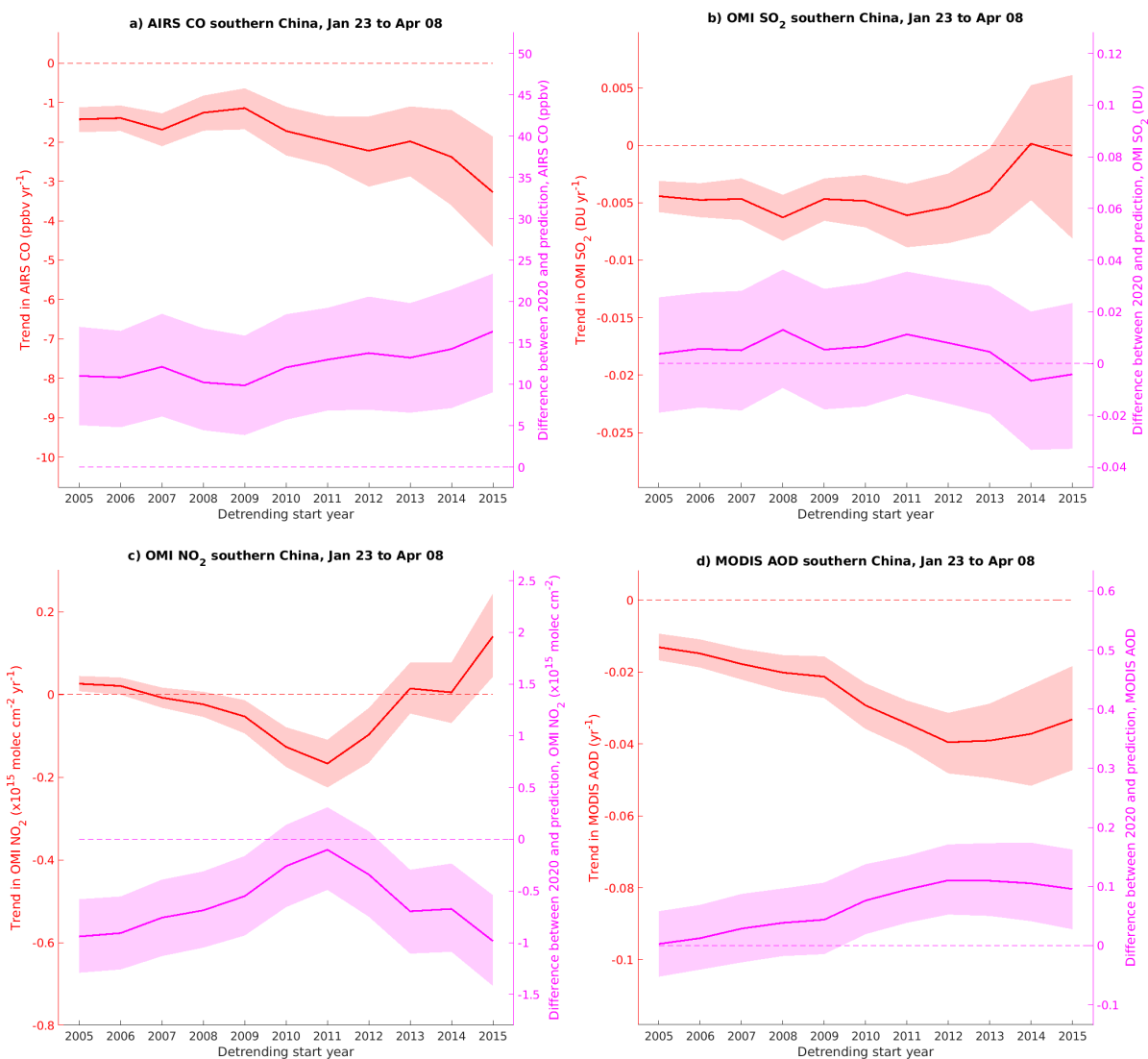
Figure S4. Same as Figure 7, but when daily values are calculated from the median of individual retrievals, rather than the mean.
