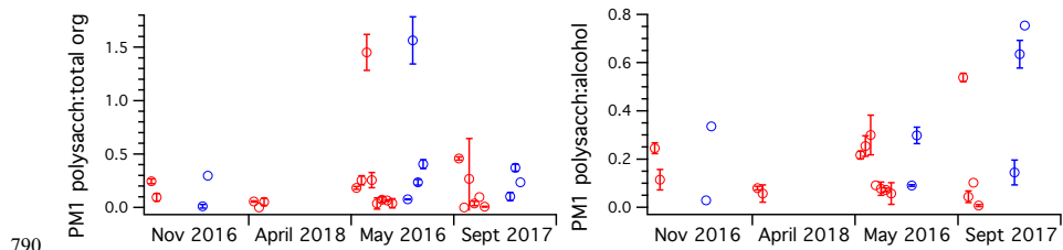
795 Figure 6: Ratio plots of (left) TDCIMS polysaccharide to FTIR total organics and (right) TDCIMS polysaccharide mass to FTIR alcohol group mass ratios for PMI aerosol filter samples taken over the 4 NAAMES cruises, organized by season. Any negative (below background) signals were removed from the analysis. One standard deviation error bars are plotted for samples with replicate runs on TDCIMS.
