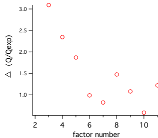
655 Figure 2: Change in the ratio of Q to Q expected as a result of increasing to a given factor number. Relatively strong improvements are seen for changes up to five factors, with additions to 6 and 7 factors showing much smaller improvement. Above 5 factors the ratio is variable and improvement is marginal.
