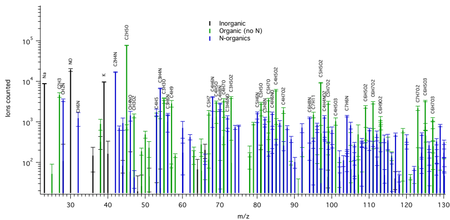
650 Figure 1: Example mass spectrum of background-corrected TDCIMS-derived positive ion signals for an ambient submicron aerosol sample collected UTC 15:15 May 26 – 09:00 May 27, 2016. Ion types are color-coded: inorganic (black), organic with no N (green), and N-containing organics (blue). All labeled organic ion compositions can be assumed to include an H + adduct. Only a subset of the mass range is shown for clarity. Peaks of over 2000 ion counts are labeled, except when overlapping with a higher peak. The square root of counted ions is plotted as error bars.
