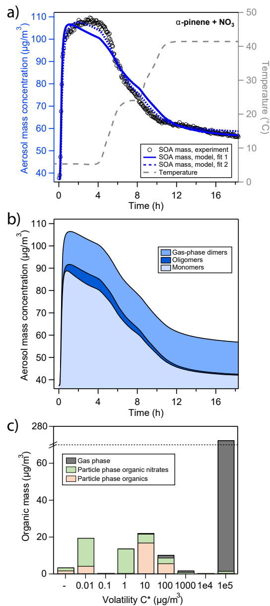
Figure 3. (a) Comparison of experimental and modelling results of aerosol mass for oxidation of \alpha -pinene with \text{NO}_3 . Open black markers are experimental aerosol masses obtained using an SMPS. The blue solid line represents the best fit model result, the blue dotted line an alternative model fit and the grey dashed line corresponds to the experimental temperature profile. (b) Analysis of the oligomerization state of particle-phase products in the model according to fit 1. (c) Analysis of the occupation of volatility bins of all products according to fit 1 and during peak SOA mass. Shadings in the bar plot denote where molecules of a certain volatility bin reside: gas phase (grey) or particle phase (colored). Products in the particle phase are further distinguished as organic nitrates (green) and non-nitrated organics (orange).
