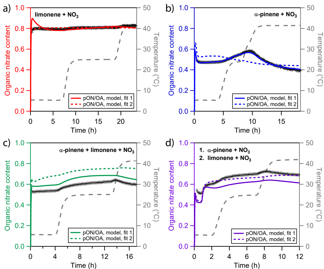
Figure 5. Experimental and modelling results of particulate organic nitrate content (pON/OA) for four different types of chamber-generated SOA. (a) only limonene, (b) only \alpha -pinene, (c) a mixture of \alpha -pinene and limonene and (d) sequential oxidation of firstly \alpha -pinene and secondly limonene. Cross markers are experimental nitration degrees inferred using a High Resolution Time-of-Flight Aerosol Mass Spectrometer (HR-ToF-AMS). The colored solid and dotted lines represent results of the kinetic model. The grey dashed line indicates the experimental temperature profile.
