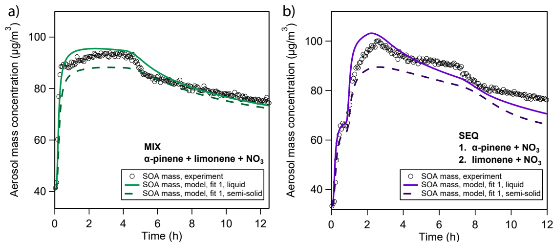
Figure 6. Sensitivity study on the influence of viscosity on model simulation results based on the best case fitting scenario in the (a) MIX and (b) SEQ experiments. Model simulations were performed for the default well-mixed case (solid lines) and at a diffusivity coefficient of 1 \times 10^{-16} \text{ cm}^2/\text{s} , which corresponds to a bulk viscosity of 1 \times 10^7 \text{ Pa}\cdot\text{s} according to the Stokes-Einstein relation and falls within the semi-solid phase state range.
