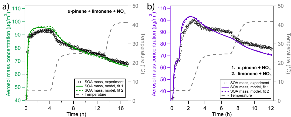
Figure 4. Overview of experimental and modelling results of aerosol mass for experiments with mixed monoterpene precursors. The experiments in the two panels differ in the way the precursors were added: (a) simultaneous oxidation of a mixture of \alpha -pinene and limonene, (b) sequential oxidation of firstly \alpha -pinene and secondly limonene with \text{NO}_3 . Open black markers are experimental aerosol mass obtained using an SMPS. The colored solid and dotted lines represent model results from two different fits to the experimental data. The grey dashed line indicates the experimental temperature profile.
