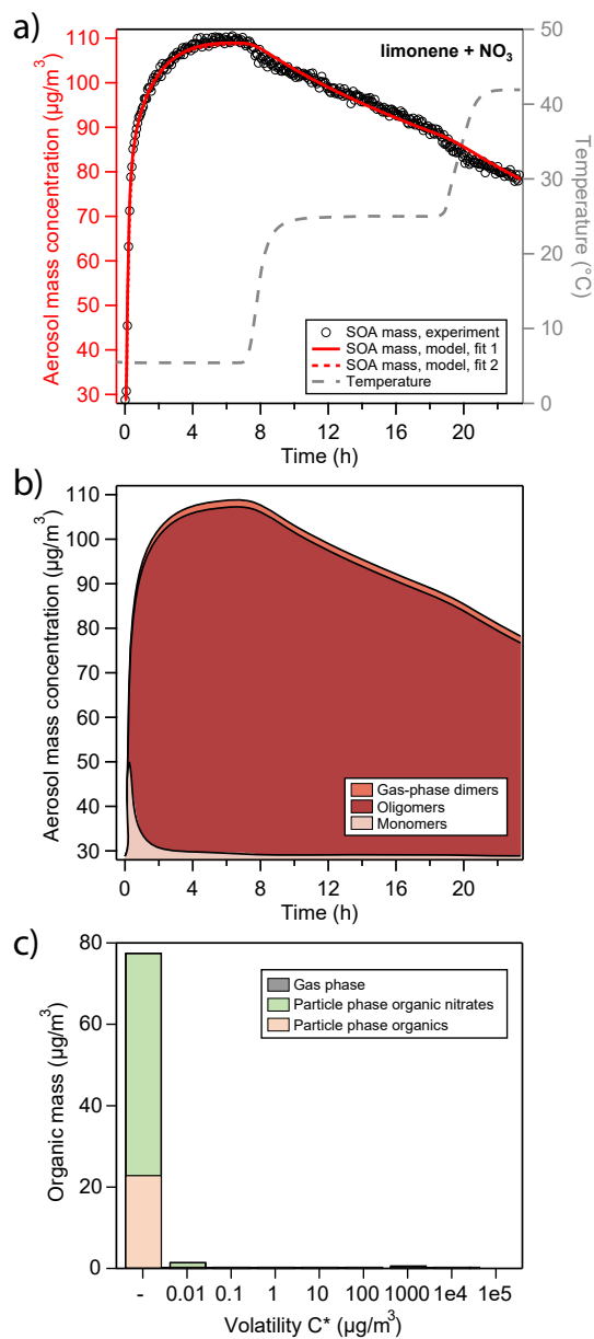
Figure 2. (a) Comparison of experimental and modelling results for oxidation of limonene with \text{NO}_3 . Open black markers are experimental aerosol mass obtained using an SMPS. The red solid line represents the best fit model result, the red dotted line an alternative model fit and the grey dashed line corresponds to the experimental temperature profile. (b) Analysis of the oligomerization state of particle-phase products in the model according to fit 1. (c) Analysis of the occupation of volatility bins of all products according to fit 1 and at peak SOA mass. Shadings in the bar plot denote where molecules of a certain volatility bin reside: gas phase (grey) or particle phase (colored). Products in the particle phase are further distinguished as organic nitrates (green) and non-nitrated organics (orange).
