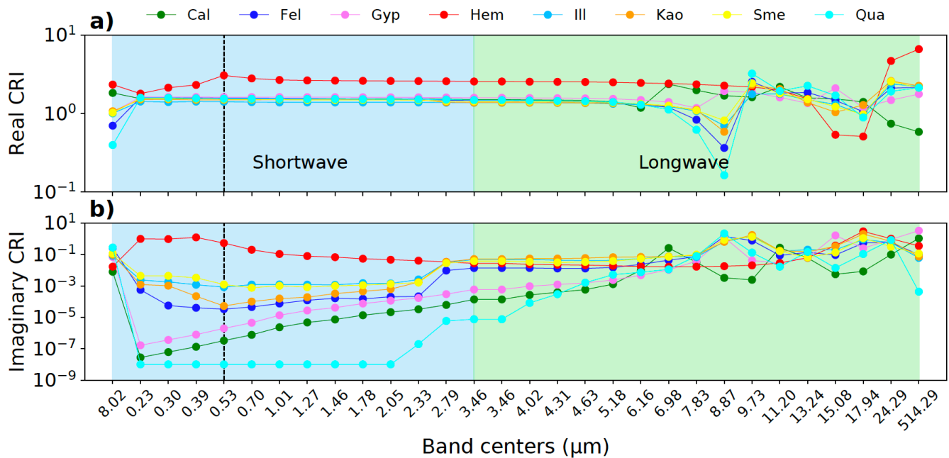
415 Figure 1. Real (a) and imaginary (b) complex refractive index (CRI) of each mineral for shortwave (blue shading) and longwave (green shading) bands (band centers shown as x-axis labels) implemented into CAM5/6. CRI values were derived for each band with original data taken from Scanza et al. (2015). The imaginary CRI of goethite was assumed to be half of hematite with the same spectral shape, while the real part of goethite is assumed to be identical as that of hematite. Vertical dash lines indicate the 420 shortwave Band 10 centered at 0.53 \mu\text{m} at which DOD and single scattering albedo for CAM5/6 were calculated (see Table 5). Note the band centered at 8.02 \mu\text{m} (leftmost) is broad with the low and high boundaries of 3.84 and 12.20 \mu\text{m} , respectively. This broad band has been included in the model as shortwave bands by model developers.
