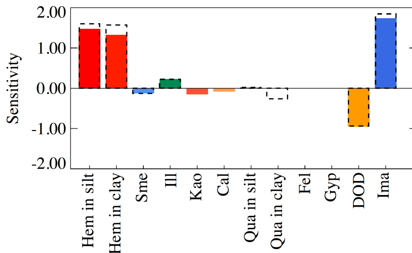
1485 Figure 10: Sensitivity parameter (unitless) of the shortwave DRE to simulated minerals (hematite, smectite, and illite), DOD, and the prescribed imaginary complex refractive indices within the known uncertainty in CAM5. The sensitivity is measured by the ratio of the relative change of shortwave DRE to that of parameters considered. Bars: values associated with higher (in color) and lower bounds (dash with opposite signs to real values) of minerals, DOD, and imaginary complex refractive index. X-axis labels: Hem-hematite; Sme-smectite; Ill-illite; Kao-kaolinite; Cal-calcite; Qua-quartz; Fel-feldspar; Gyp-gypsum; DOD; Ima-Imaginary; 1490 J. iron oxide-iron oxide in J2014. Sensitivity for parameters other than hematite, DOD, and imaginary complex refractive index, was derived from the “normalized” cases (see Section 2.3.1 ).
