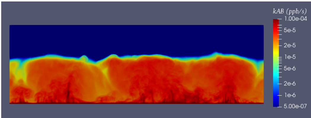
Figure 2: The top panel of Figure 2 in the manuscript ( top panel ) and the color map of the same simulation with a time-averaged field of the production field over the last 30 minutes of the simulation ( bottom panel ).
