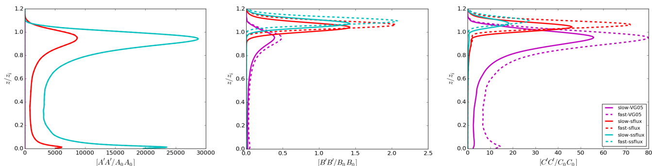
Figure 4: The vertical profiles of the concentration variances of Tracer A ( left panel ), B ( middle panel ) and C ( right panel ) normalised by the corresponding characteristic concentrations.
