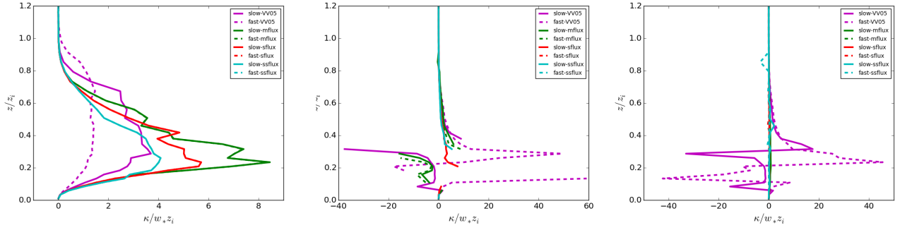
Figure 3: The vertical profiles of the horizontally-averaged exchange coefficients ( \kappa ) of Tracer A (left panel), B (middle panel) and C (right panel) normalised by the product of the boundary layer height z_i and the convective velocity w_* . Here the same simulation cases are shown as in Figure 3 of the manuscript. The data here are averaged every 8 vertical levels to lessen the effect of the noise.
