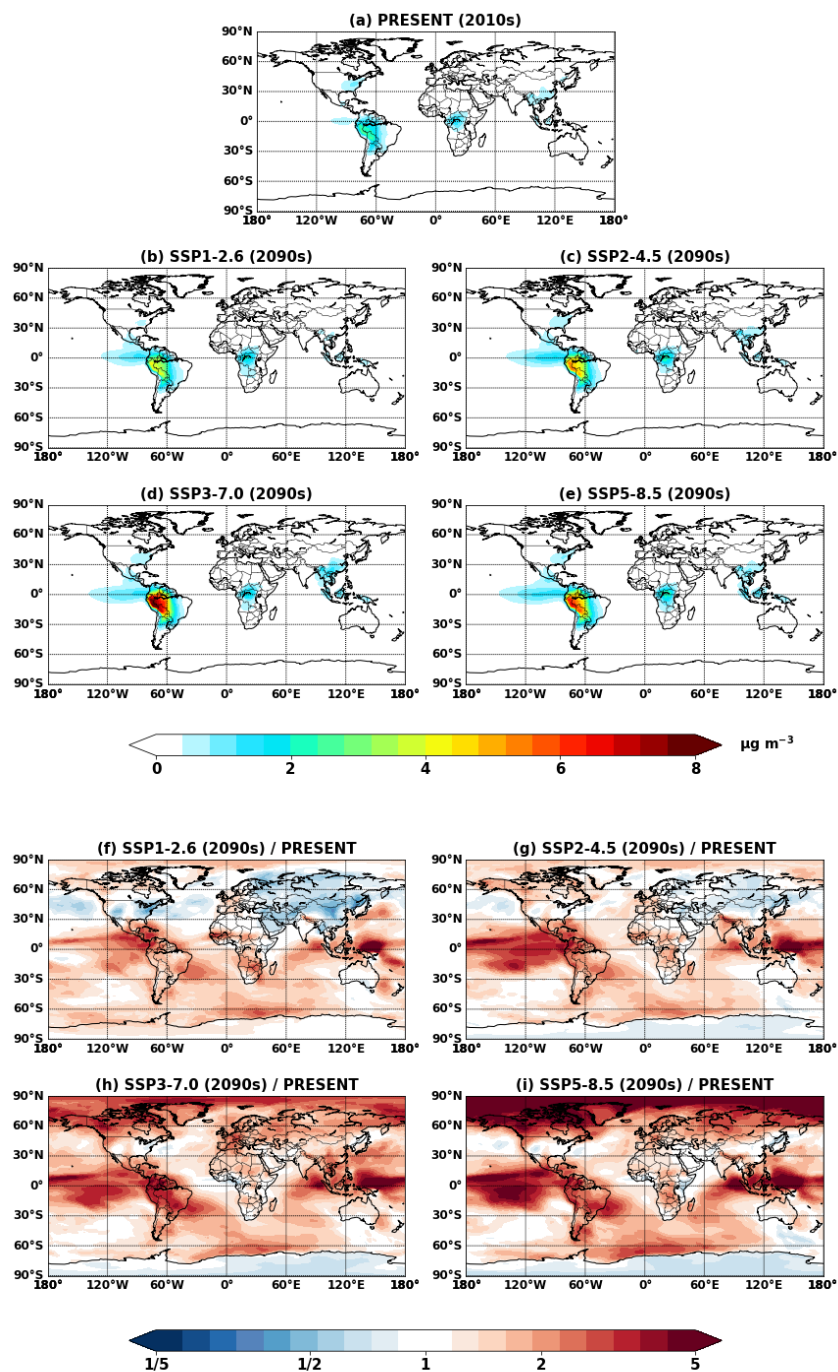
680 Figure 9. Global mean IEPOX-SOA concentrations at the surface simulated in (a) Explicit_CO2_2010 and (b-e) Explicit_CO2_2090_SSPx. (f-i) Ratios of IEPOX-SOA between future (b-e) and present (a) conditions.
