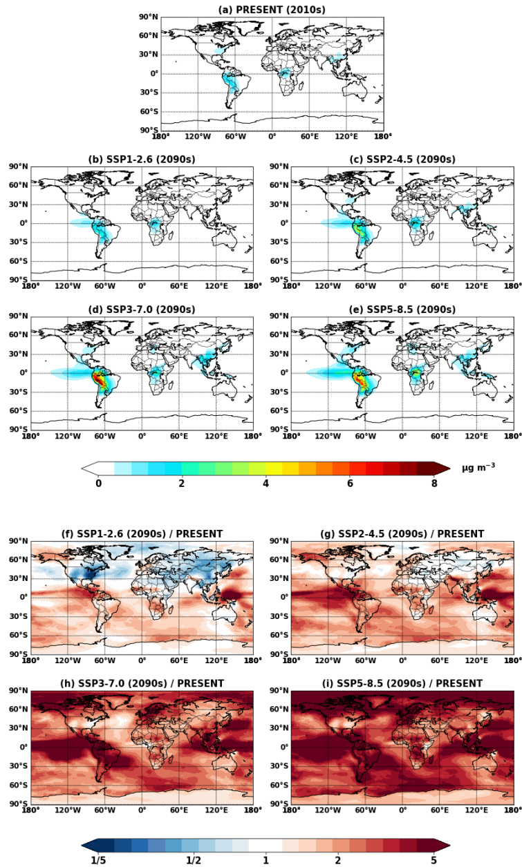
Figure 7. Global mean IEPOX-SOA concentrations at the surface simulated in (a) Explicit_SS_2010 675 and (b-e) Explicit_SS_2090_SSPx . (f-i) Ratios of IEPOX-SOA between future (b-e) and present (a) conditions.
