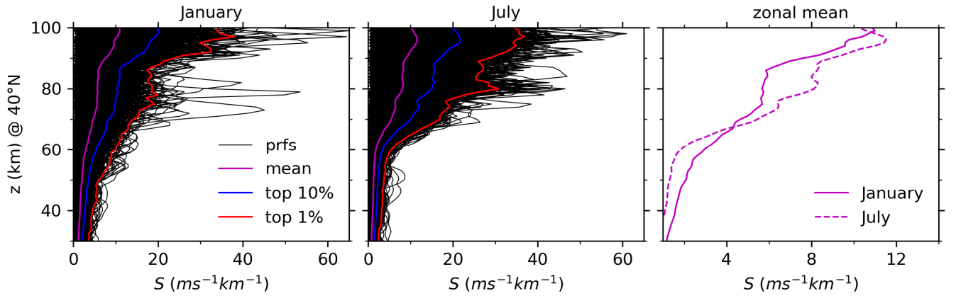
Figure 13. Same caption as Fig. 5 but for the GW-perturbed profiles derived under the medium frequency assumption f/\hat{\omega}_j = 0 and at 40^\circ\text{N}
