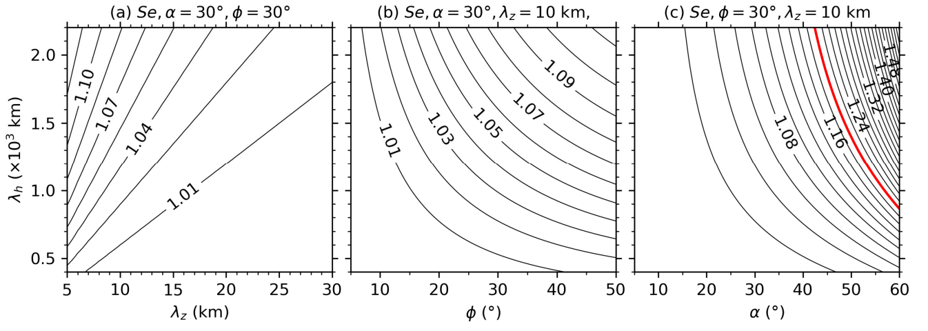
Figure 3: Dependencies of S_e on the horizontal and vertical wavelengths for \alpha = 30^\circ and \phi = 30^\circ (a), on the latitude \phi for \alpha = 30^\circ and \lambda_z = 10 \text{ km} (b) and on the angle \alpha for \phi = 30^\circ (c). The red contour line in (c) indicates S_e = 1.2 . All panels have the same y-axis scale.
