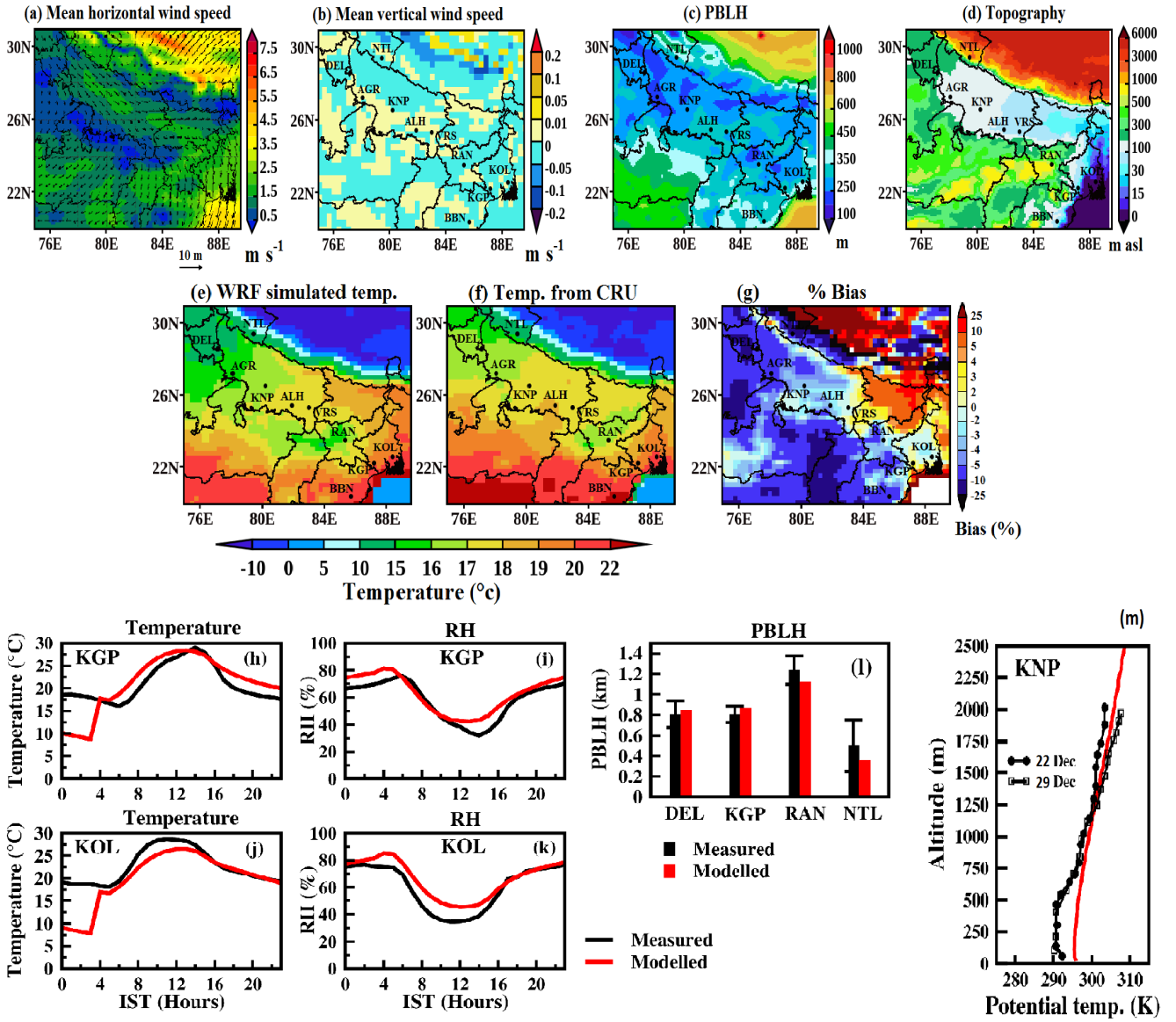
Figure 2. Spatial distribution of WRF simulated (a–c) winter monthly mean of (a) horizontal wind field (note the color scale is for wind speed in m s^{-1} and the arrows indicate the direction of the mean field), (b) vertical wind speed at 1000 hPa, (c) planetary boundary layer height (PBLH in m), and (d) topography (m above sea level, m asl); (e–g) spatial distribution of winter monthly mean of surface temperature from (e) WRF simulations, (f) observations from CRU, (g) percentage bias in winter-monthly-mean-temperature-from-WRF-estimates ; (h–k) validation comparison of hourly distribution of winter monthly mean of (h,j) surface temperature, (i,k) relative humidity from WRF simulations with observations at stations (Kharagpur, KGP; Kolkata, KOL); (l) comparison between-measured-and-simulated-of winter monthly mean of PBLH during day hours between-measured-and-simulated-values at stations under study. The error bars present-represent the standard deviation ( \sigma ) in measured PBLH. Refer-to-Table-2-for-details-on-observational-data ; (m) comparison-of-vertical-profile-of-potential-temperature-obtained-from-WRF-winter-monthly-mean and measurements (two days).
