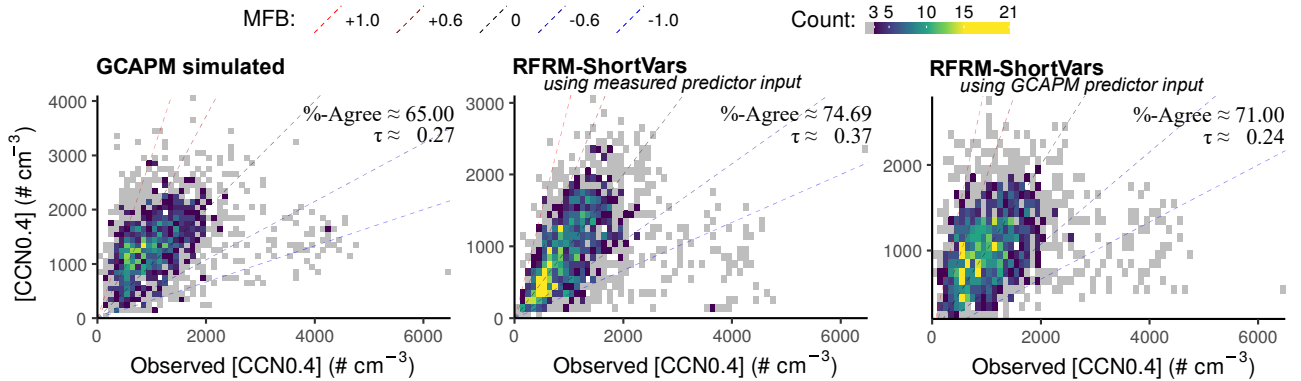
Figure 12. (a) Time series (daily-aggregated) for [CCN0.4] derived by RFRM-ShortVars ( top two ) and ORF ( middle two ), compared to SGP measured ( bottom-left ) and GCAPM-simulated ( bottom-right ). (b) Performance comparison of the models in quantifying [CCN0.4] compared to its measured values for the SGP site— left : GCAPM, centre : RFRM-ShortVars with measurements of predictors as input, and right : RFRM-ShortVars with GCAPM-simulated predictors as input. The summary performance metrics are \tau : Kendall’s rank correlation coefficient and %-Agree: the percentage of pairwise model–observation compared values within the good-agreement range defined as -0.6 < \text{MFB} < +0.6 .
