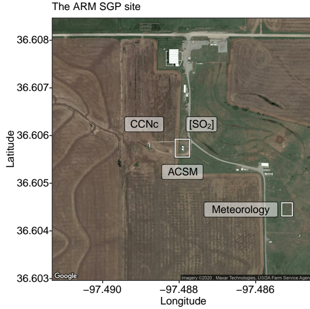
Figure 1. The ARM SGP site in Lamont, Oklahoma, U.S.A with marked locations of the instruments. Legend — Meteorology: temperature and relative humidity measurements from the ARM Surface Meteorology Systems (MET) (Holdridge and Kyrouac, 1993; Chen and Xie, 1994). ACSM: Aerodyne Aerosol Chemical Speciation Monitor (Ng et al., 2011). [SO 2 ]: concentrations of SO 2 measured by the ARM Aerosol Observing System (AOS; Hageman et al., 1996). CCNc: Cloud Condensation Nuclei Particle Counter (CCNc) (Shi and Flynn, 2007; Smith et al., 2011a, b; Hageman et al., 2017). This image is adapted from satellite imagery © 2020 Maxar Technologies, USDA Farm Service Agency obtained through the Google Maps Static API.
