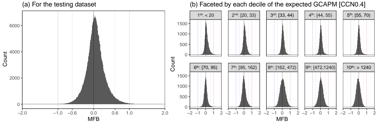
Figure 9. Mean fractional bias (MFB) of RFRM derived [CCN0.4] compared to expected values from GCAPM in the testing dataset (441756 values). Histogram shows the counts of the pairs by MFB. The lines indicate perfect agreement (black), MFB of +1 (dashed red), and MFB of -1 (dashed blue). The dotted lines indicate MFB of +0.6 (dotted red) and -0.6 (dotted blue).
