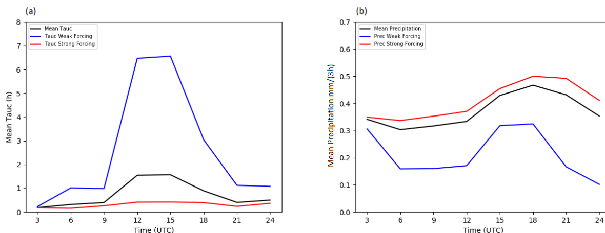
Figure 5. Aggregated diurnal cycle of the ensemble mean convective adjustment time-scale (a) and 3-hourly precipitation (b) averaged over the full SOP1 period (black) and over weakly (blue) and strongly forced weather regimes (red) across the Northwestern Mediterranean domain.
