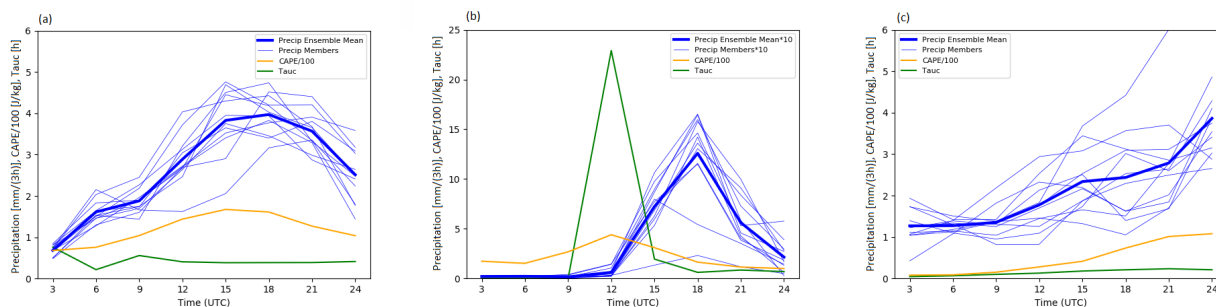
Figure 6. Time series of ensemble mean area averaged precipitation, CAPE and convective adjustment timescale \tau_c for the prominent cases (a) HyMeX IOP16a, (b) HyMeX 11 Sep 2012 and (c) NAWDEX 13 Oct 2016. Additionally the precipitation timeseries of the individual ensemble members highlights intra-ensemble variability. Note the different scale on 11 Sept 2012.
