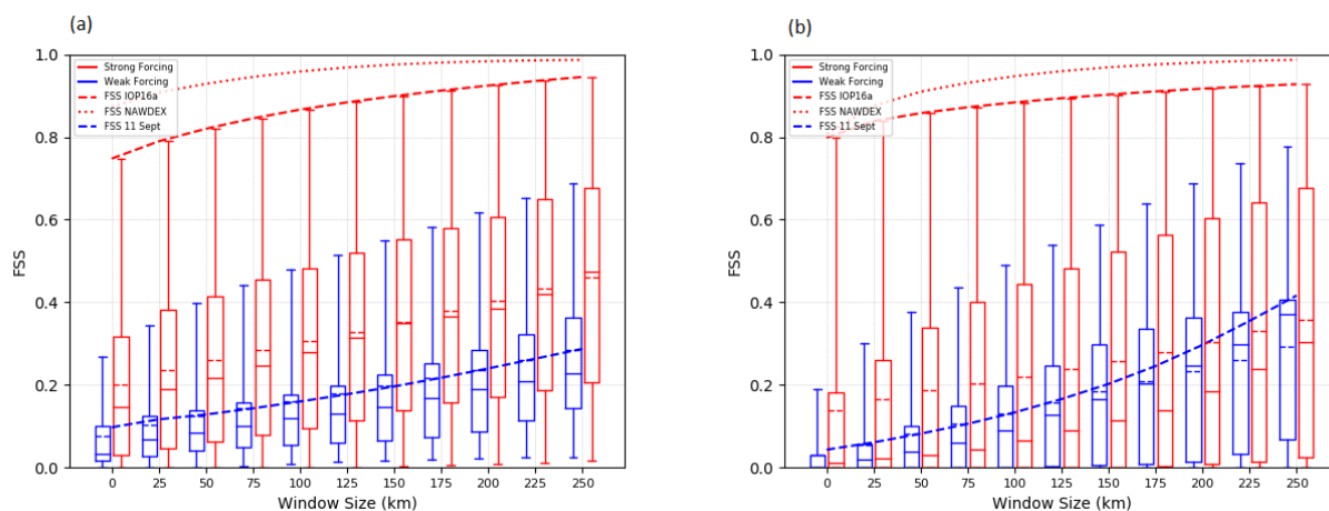
Figure 13. Fraction Skill Score FSS of ensemble mean 3-hourly precipitation vs interpolated rain-gauge observations as a function of neighborhood size conditional to weather regime: (a) 0.3\text{mm}(3\text{h})^{-1} and (b) 10\text{mm}(24\text{h})^{-1} , all averaged for the entire HyMeX SOP1. The horizontal line (dashed line) within the boxes indicates the median (mean), respectively. The boxes and whiskers are slightly displaced at the discrete window sizes (weak to the left, strong to the right) to increase readability. Additionally, the FSS of the prominent cases is depicted.
