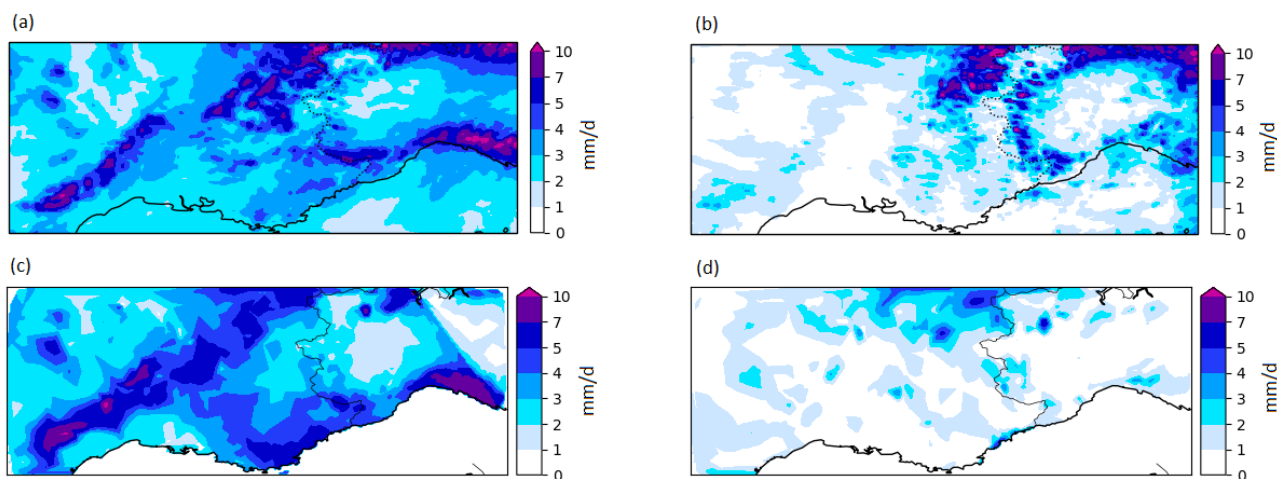
Figure 4. Aggregated mean daily precipitation divided into strong (a,c) and weak (b,d) forcing conditions. Displayed are ensemble mean (a,b) and interpolated rain-gauge observations (c,d) of 24 h precipitation for the 2-months period in autumn 2012.
