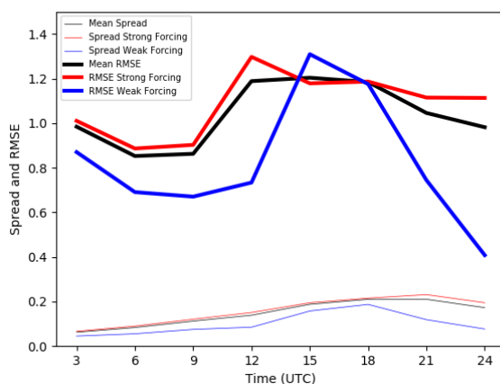
Figure 11. Aggregated time series of the spread (standard deviation) and skill (RMSE) averaged over the full SOP1 period (black) and over weakly (blue) and strongly forced weather regimes (red). The RMSE is the ensemble mean of the member RMS forecast error.
