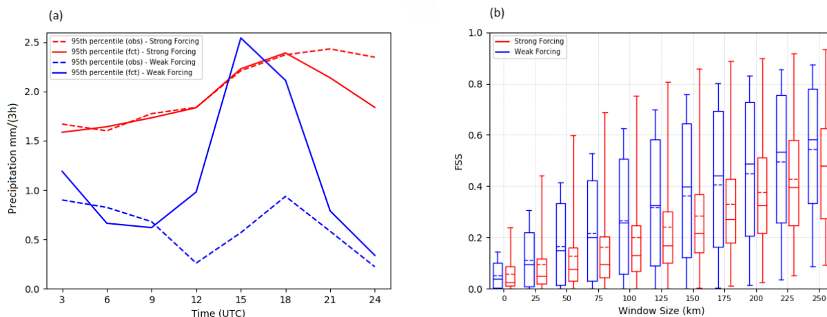
Figure 14. (a) Aggregated diurnal cycle of 3-hourly precipitation values corresponding to the 95th percentiles, both stratified in weakly (blue) and strongly forced weather regimes (red) and averaged over the full SOP1 period. (b) FSS of 95th percentiles of 3-hourly precipitation as a function of neighborhood size conditional to weather regime averaged for the entire HyMeX SOP1 between 12 and 18 UTC.
