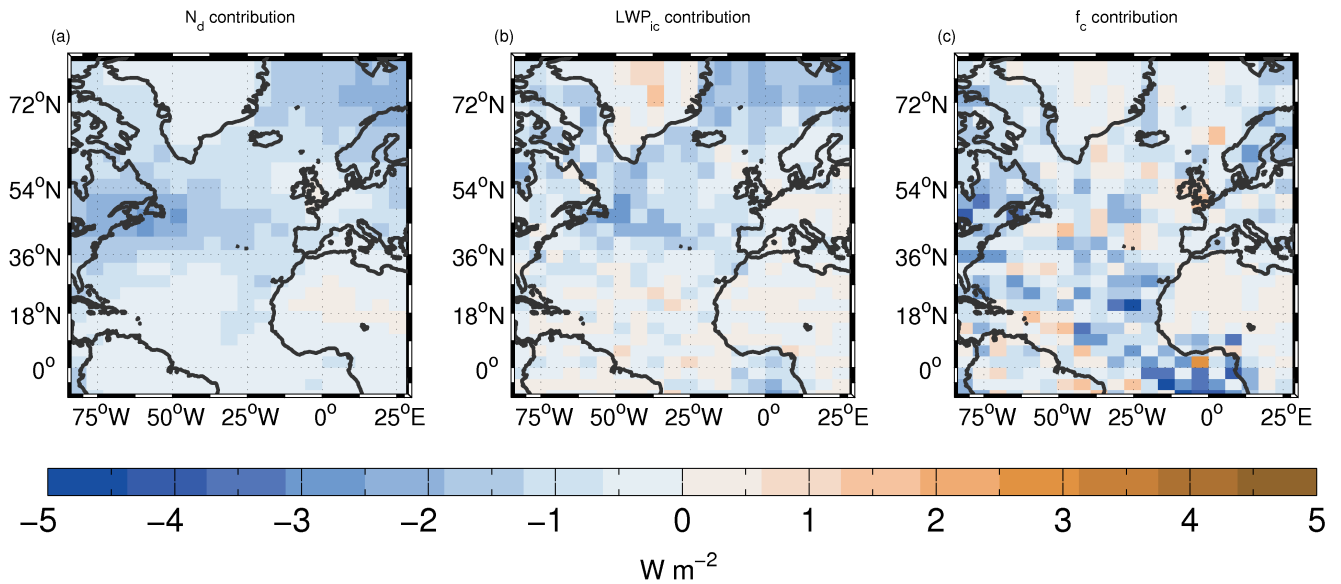
Figure 15. Estimated contributions to the surface ACI forcing from changes in N_d (left), LWP_{ic} (middle) and f_c (right). Fig. 14c shows the sum of these three terms.
