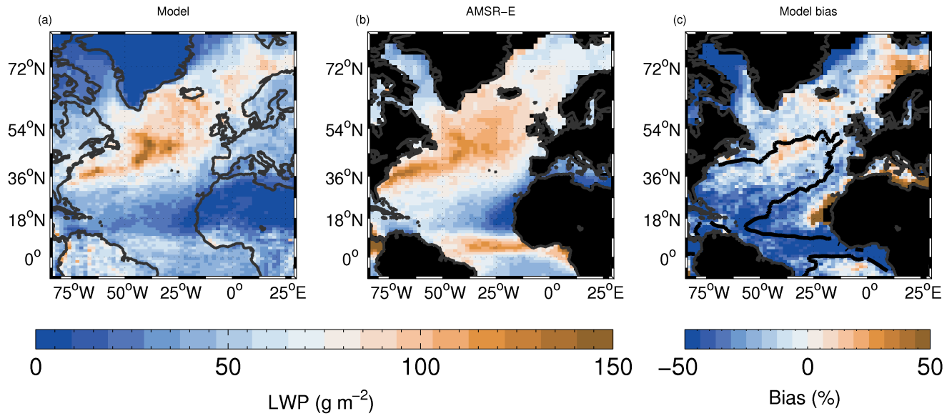
Figure D1. Time-mean all-sky (i.e., including cloudy and clear regions) LWP model evaluation for both day and night overpasses. c) includes a contour of the 0.9 value of f_{LWP} ; see Fig. 4 for the full map of f_{LWP} for reference.
