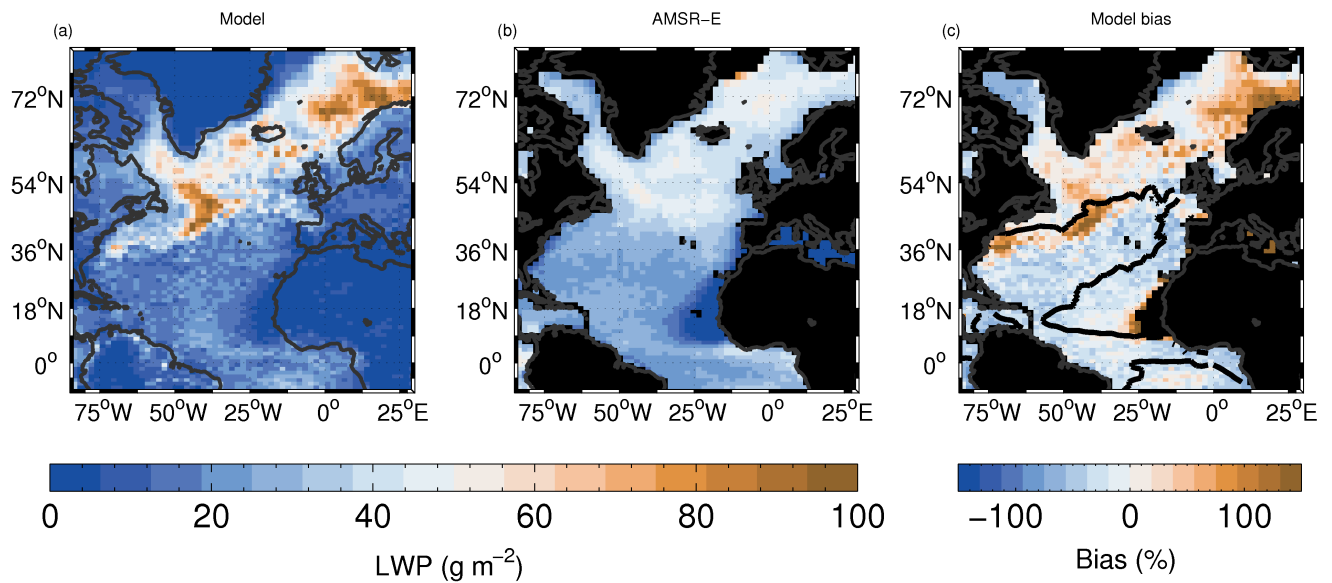
Figure D2. As for Fig. D1 except both the model and satellite data has been filtered before time averaging to only include datapoints for which f_{LWP} is greater than 0.99. This quantity is denoted as LWP_{0.99} .
