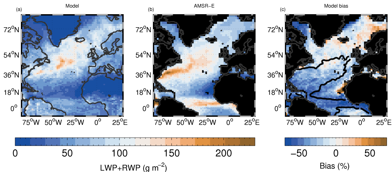
Figure D3. As for Fig. D1 except with the addition of the all-sky rain water path (RWP) for both the model and AMSR-E satellite data. No filtering for f_{LWP} has been applied.
