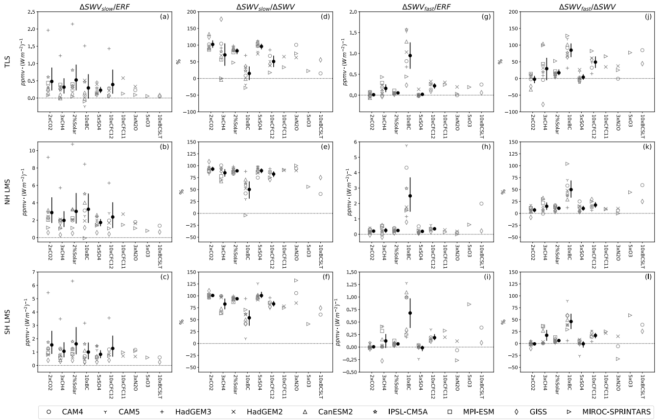
630 Figure 1. Panels (a)-(c): equilibrium \Delta SWV_{slow} normalized by ERF ( \text{ppmv} \cdot (\text{Wm}^{-2})^{-1} ) in TLS (70 hPa, 30°N-30°S), NH LMS (200 hPa, 50°N-90°N), and SH LMS (200 hPa, 50°S-90°S). Panels (d)-(f): Contribution (%) of equilibrium \Delta SWV_{slow} to total equilibrium \Delta SWV . Panels (g)-(i): \Delta SWV_{fast} normalized by ERF ( \text{ppmv} \cdot (\text{Wm}^{-2})^{-1} ). Panels (j)-(l): Contribution (%) of \Delta SWV_{fast} to total equilibrium \Delta SWV . The marker shapes indicate results from different models. For perturbations that are performed by more than three models, the solid circles and error bars for each perturbation plotted in weighted black are multi-model mean and 2.5%-97.5% percentiles of the model samples. Note that in the second and fourth columns, we took out models with extremely small \Delta SWV magnitudes that yield extremely large \Delta SWV_{slow}/\Delta SWV and \Delta SWV_{fast}/\Delta SWV ratios. 635
