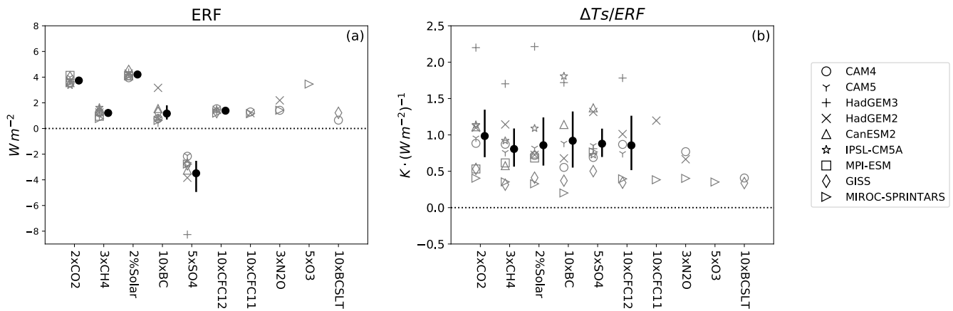
640 Figure 2. Panel (a): Global average ERF ( W m^{-2} ) at the top of atmosphere. Panel (b): Global averaged surface temperature change per unit ERF ( K \cdot (W m^{-2})^{-1} ). The marker shapes indicate results from different models. For perturbations that are performed by more than three models, the solid circles and error bars for each perturbation plotted in weighted black are multi-model mean and 2.5%-97.5% percentiles of the model samples.
