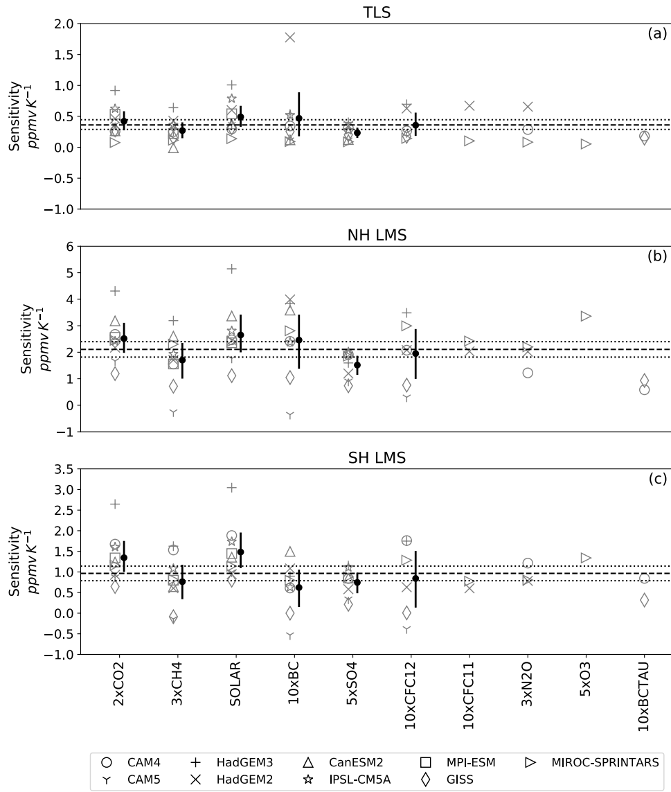
645 Figure 3. Slopes ( \text{ppmv K}^{-1} ) from the linear regression between annual mean \Delta\text{SWV}_{\text{slow}} time series and annual mean \Delta\text{T} s time series. The marker shapes indicate results from different models. For perturbations that are performed by more than three models, the solid circles and error bars for each perturbation plotted in weighted black are multi-model mean and 2.5%-97.5% percentiles of the model samples. The horizontal dashed line is the multi-model mean of all slopes, and the horizontal dotted lines are 2.5%-97.5% percentiles of the model samples.
