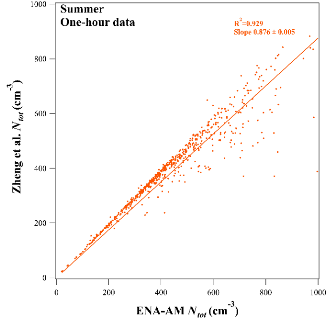
Figure SL.8. Scatter plot of Zheng et al. (2018) and ENA-AM masked one-hour N_{tot} data at C1 in the summer.
