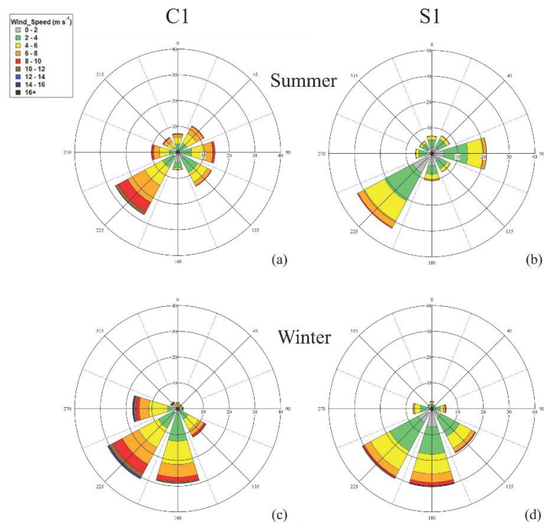
Figure SI.1. Surface wind rose plots during the summer (a, b) and winter (c, d) at C1 and S1. The length of the radial bars is the frequency of different wind speed ranges shown in colour, as a percentage of the time sampled.
