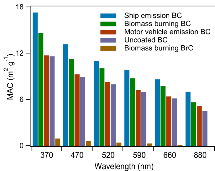
Figure 6. The source-specific mass absorption cross section (MAC) of black carbon (BC) and brown carbon (BrC) at different wavelengths. The MAC of uncoated BC particles at each wavelength are 5 extrapolated from 7.5 \text{ m}^2 \text{ g}^{-1} at 550 nm (Bond and Bergstrom, 2006) by assuming an BC absorption Ångström exponent of 1.1.
