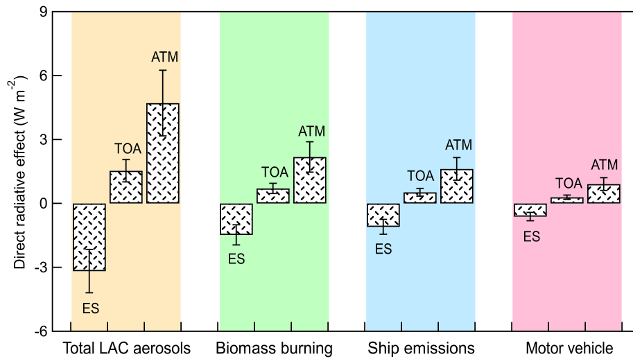
Figure 7. Direct radiative effect (DRE) of light-absorbing carbonaceous (LAC) aerosols from biomass burning, ship emissions, and motor vehicle emissions. The error bar represents one standard deviation. ES, TOA, ATM represent the DRE at the Earth's surface, the top of the atmosphere, and in the atmosphere, respectively.
