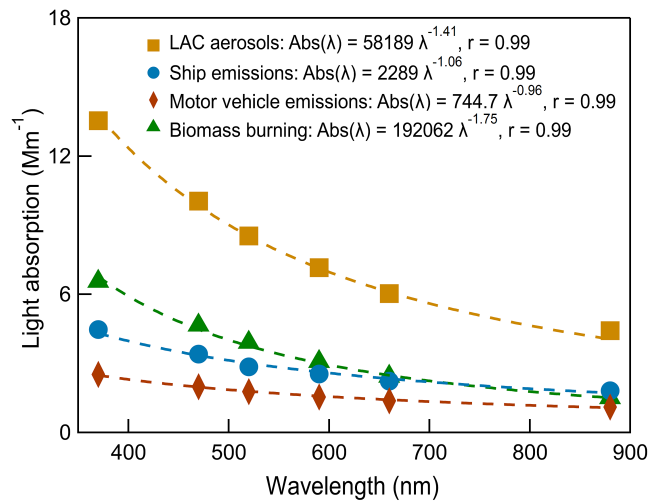
Figure 5. The light absorption ( \text{Abs}(\lambda) ) of light-absorbing carbonaceous (LAC) aerosols from ship emissions, traffic emissions, and biomass burning. The dash line is power law fit.
