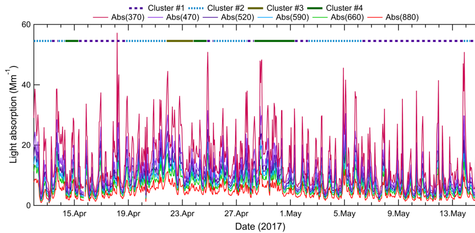
Figure 2. Time series of hourly averaged light absorption at different wavelengths ( \text{Abs}(\lambda) , \lambda = 370, 470, 520, 590, 660, \text{ and } 880 \text{ nm} ). The different types of horizontal lines represent the four clusters of air masses.
