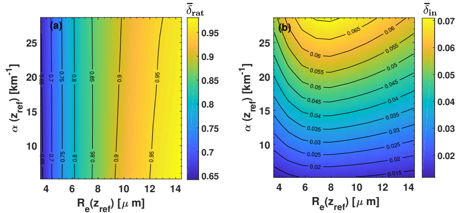
Figure 6. (a) Ratio \bar{\delta}_{rat}(z_{bot}, z_{ref}) of depolarization ratios (see Eq. (27), integration height range of \Delta z_{ref}=75 m) as a function of droplet effective radius R_e(z_{ref}) and cloud extinction coefficient \alpha(z_{ref}) . Cloud base z_{bot} is at 3 km height, z_{ref} is thus at 3.075 km height. (b) Integrated depolarization ratio \bar{\delta}_{in}(z_{bot}, z_{ref}) as a function of R_e(z_{ref}) and \alpha(z_{ref}) . Isolines of \bar{\delta}_{rat} in (a) show the strong dependence of \bar{\delta}_{rat} on the effective radius. The \bar{\delta}_{in} isolines in (b) highlight the dominating influence of the extinction coefficient on \bar{\delta}_{in} . The figures are based on 720 simulated cloud scenarios for each of the FOVs of 1 mrad and 2 mrad.
