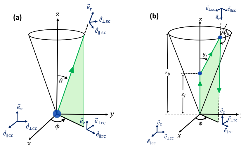
Figure 1. Scattering geometry for (a) one single scattering event and (b) one forward and one backward scattering event.
