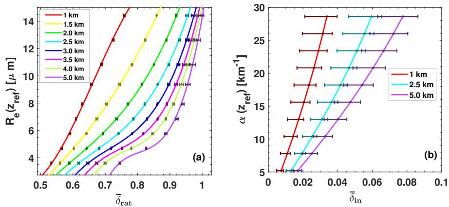
Figure 7. (a) Droplet effective radius R_e(z_{ref}) as a function of \bar{\delta}_{rat} = \bar{\delta}_{in}/\bar{\delta}_{out} for \Delta z_{ref}=75 m and (b) relationship between the measured \bar{\delta}_{in} for FOV=1 mrad and cloud extinction coefficient \alpha . Eight different cloud layers with base height z_{bot} from 1–5 km height (given as numbers in the panels) are simulated in (a), three different layers are simulated in (b). For each cloud layer (indicated by different colors) simulations with all combinations of R_e - \alpha profile pairs (in Table 1) are performed. The small bars in (a) indicate the range of possible \bar{\delta}_{rat} values for a given R_e value and the length of the bars indicate the very low \alpha influence on the R_e retrieval (simulated \alpha range is given in Table 1). A polynomial regression is applied to the mean values of \bar{\delta}_{rat} . This regression analysis is performed for each of the eight cloud layers. The cubic model (Eq. 28) for each cloud layer is indicated as thick solid colored line. The bars in (b) indicate the range of possible \bar{\delta}_{in} values for a given \alpha value. Here, the length of the bars indicate the relatively strong R_e influence on the \alpha(z_{ref}) retrieval (simulated R_e range is given in Table 1). The respective regression analysis leads here to the thick solid lines calculated with Eq. (29).
