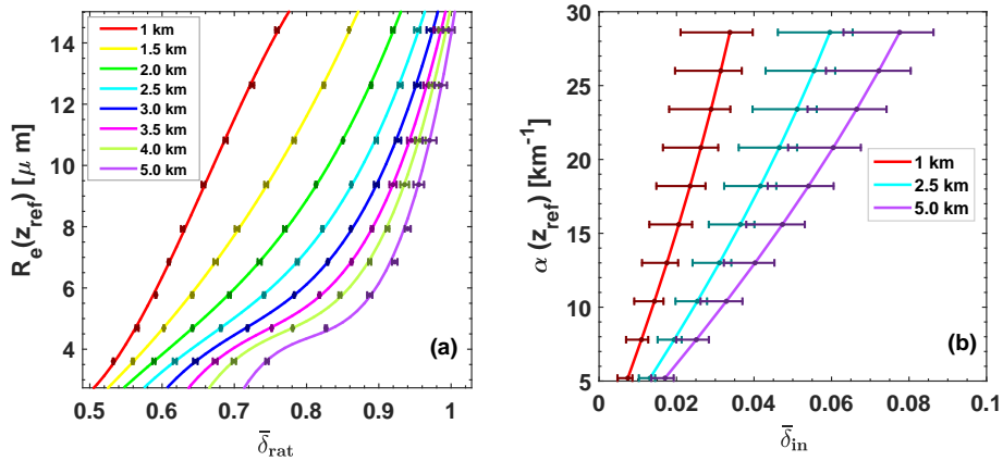
Figure 7. (a) Droplet effective radius R_e(z_{\text{ref}}) as a function of \bar{\delta}_{\text{rat}} = \bar{\delta}_{\text{in}}/\bar{\delta}_{\text{out}} for \Delta z_{\text{ref}}=75 m and (b) relationship between the measured \bar{\delta}_{\text{in}} for FOV=1 mrad and cloud extinction coefficient \alpha . Eight different cloud layers with base height z_{\text{bot}} from 1–5 km height (given as numbers in the panels) are simulated in (a), three different layers are simulated in (b). For each cloud layer (indicated by different colors) simulations with all combinations of R_e - \alpha profile pairs (in Table 1) are performed. The small bars in (a) indicate the range of possible \bar{\delta}_{\text{rat}} values for a given R_e value and the length of the bars indicate the very low \alpha influence on the R_e retrieval (simulated \alpha range is given in Table 1). A polynomial regression is applied to the mean values of \bar{\delta}_{\text{rat}} . This regression analysis is performed for each of the eight cloud layers. The cubic model (Eq. 28) for each cloud layer is indicated as thick solid colored line. The bars in (b) indicate the range of possible \bar{\delta}_{\text{in}} values for a given \alpha value. Here, the length of the bars indicate the relatively strong R_e influence on the \alpha(z_{\text{ref}}) retrieval (simulated R_e range is given in Table 1). The respective regression analysis leads here to the thick solid lines calculated with Eq. (29).
