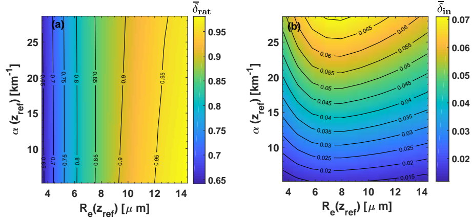
Figure 6. (a) Ratio \bar{\delta}_{\text{rat}}(z_{\text{bot}}, z_{\text{ref}}) of depolarization ratios (see Eq. (27), integration height range of \Delta z_{\text{ref}}=75 m) as a function of droplet effective radius R_e(z_{\text{ref}}) and cloud extinction coefficient \alpha(z_{\text{ref}}) . Cloud base z_{\text{bot}} is at 3 km height, z_{\text{ref}} is thus at 3.075 km height. (b) Integrated depolarization ratio \bar{\delta}_{\text{in}}(z_{\text{bot}}, z_{\text{ref}}) as a function of R_e(z_{\text{ref}}) and \alpha(z_{\text{ref}}) . Isolines of \bar{\delta}_{\text{rat}} in (a) show the strong dependence of \bar{\delta}_{\text{rat}} on the effective radius. The \bar{\delta}_{\text{in}} isolines in (b) highlight the dominating influence of the extinction coefficient on \bar{\delta}_{\text{in}} . The figures are based on 720 simulated cloud scenarios for each of the FOVs of 1 mrad and 2 mrad.
