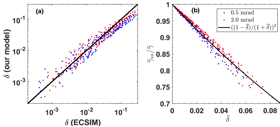
Figure 3. (a) Comparison of the volume linear depolarization ratios \delta(z) computed with our analytical MS model and computed with ESA's Monte-Carlo model ECSIM (more details in the text, 1:1 line is given as solid diagonal line) and (b) comparison of our computations of the relationship between the single-scattering-to-total-scattering-attenuated-backscatter ratio \bar{\gamma}_{ss}/\bar{\gamma} and the cloud-integrated depolarization ratio \bar{\delta} (red and black circles) with the respective values for this relationship as retrieved from CALIPSO multiple scattering observations (solid black line). For the two different FOVs ( 0.5 mrad in black, 2.0 mrad in red) 4 \times 4 R_e(z_{ref}) - \alpha(z_{ref}) combinations are considered together with different cloud penetration depths \Delta z_{ref} from 10 to 70 m (with 10 m step width). All in all more than 200 simulations are included in each of the panels (a) and (b).
