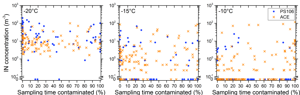
Figure C1. IN concentration vs. sampling time in ship exhaust. Measured IN concentration at -20^{\circ}\text{C} , -15^{\circ}\text{C} and -10^{\circ}\text{C} show no correlation to the time air was sampled from direction of the ships stack. Ships: RV Polarstern (PS106), Academic Tryoshnikov (ACE).
