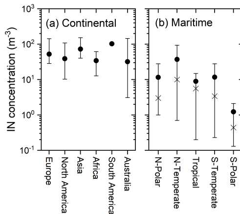
Figure 2. (a) Regionally averaged continental IN concentrations at -15\text{ }^{\circ}\text{C} (surface-based measurements, Bigg and Stevenson, 1970); (b) Meridional averaged maritime IN concentrations at -15\text{ }^{\circ}\text{C} (shown as dots). Vertical bars indicate the concentration range where 80% of observations lay, excluding the 10% highest and 10% lowest values. Most frequently measured (mode) concentration is indicated by crosses. Continental concentrations in (a) are higher, with a lower variability than maritime IN concentrations in (b).
