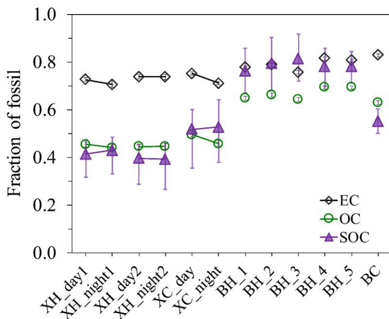
555 Figure 6. Fraction of fossil carbon in EC, OC and SOC ( f_{\text{fossil}}(\text{EC}) , f_{\text{fossil}}(\text{OC}) and f_{\text{fossil}}(\text{SOC}) , respectively). Interquartile ranges (25th–75th percentile) of the median f_{\text{fossil}}(\text{SOC}) are shown as vertical bars in purple. Uncertainties of ^{14}\text{C} -apportioned f_{\text{fossil}}(\text{EC}) and f_{\text{fossil}}(\text{OC}) are indicated but are too small to be visible.
