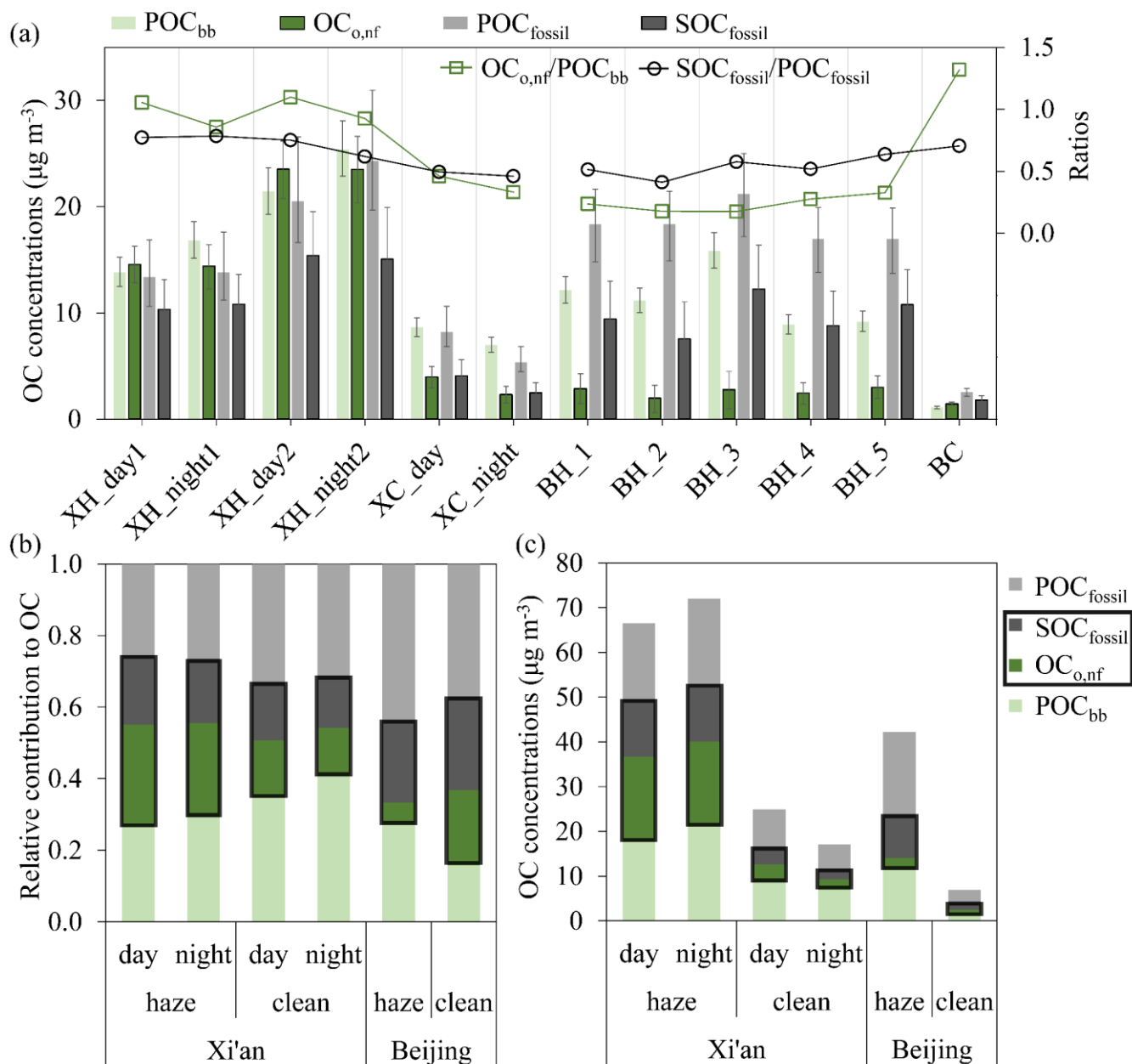
550 Figure 5. (a) Concentrations of \text{POC}_{\text{bb}} , \text{OC}_{\text{o,nf}} , \text{POC}_{\text{fossil}} and \text{SOC}_{\text{fossil}} ( \mu\text{g m}^{-3} ), and the mass ratio of \text{OC}_{\text{o,nf}}/\text{POC}_{\text{bb}} and \text{SOC}_{\text{fossil}}/\text{POC}_{\text{fossil}} of each sample. The error bars indicate the interquartile range (25th–75th percentile) of the median concentrations. Averaged fraction (b) and concentration (c) of \text{POC}_{\text{bb}} , \text{OC}_{\text{o,nf}} , \text{POC}_{\text{fossil}} and \text{SOC}_{\text{fossil}} in total OC during haze and clean periods in Xi'an and Beijing, China. The data are given in Table S4.
