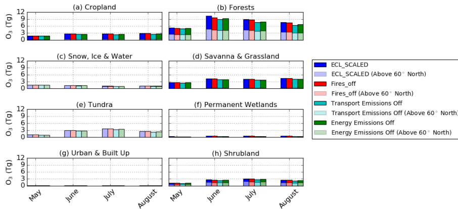
Figure 11 – Quantity of ozone deposited to modified IGBP MODIS NOAA land surface cover categories per month for total domain (solid bars) and for the section of the domain north of 60°N (pale bars).
