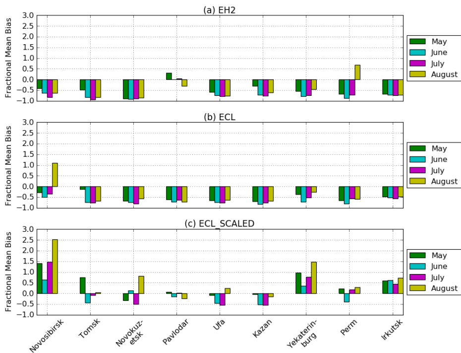
Figure 5 –Fractional mean bias of monthly simulated tropospheric column \text{NO}_2 for major cities (population >100,000) within Western Siberia when compared with OMI values. Panel (a) shows results using the EH2 anthropogenic emission inventory. Panel (b) shows results using the ECL anthropogenic emission inventory. Panel (c) shows results using the ECL_SCALED anthropogenic emission inventory.
