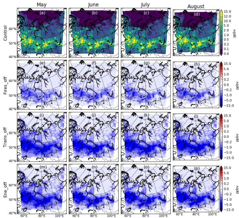
Figure 7 – Simulated control and sensitivity run changes in surface NO 2 concentrations. Panels (a)–(d) show monthly means of WRF-Chem surface NO 2 for May-August using ECL_SCALED emissions . Panels (e)–(h) show monthly means of WRF-Chem Surface NO 2 with all fire emissions switched off in domain (fires_off simulation) minus control simulation for May-August . Panels (i)–(l) show monthly means of WRF-Chem Surface NO 2 with all transport emissions switched off in domain (trans_off) minus control simulation for May-August . Panels (m)–(p) show monthly means of WRF-Chem Surface NO 2 with all energy emissions switched off in domain (ene_off) minus control simulation for May-August .
