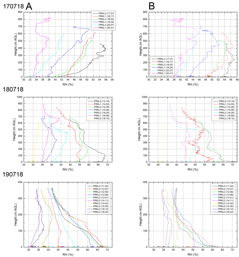
Figure 9. Vertical profiles of relative humidity measured by BME280 Arduino sensor from July 16 th – July 19 th , solid lines (left column A)–ascend data and dashed lines (right column B)–descend data
