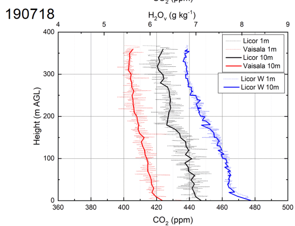
Figure 14. CO 2 and water vapor vertical profiles measured with Licor LI-840A and Vaisala GMP343 on July 16 th -19 th . Data plotted as 1 meter (dotted lines) and 10 meter averages (solid lines). Please note different height on daily figures.
