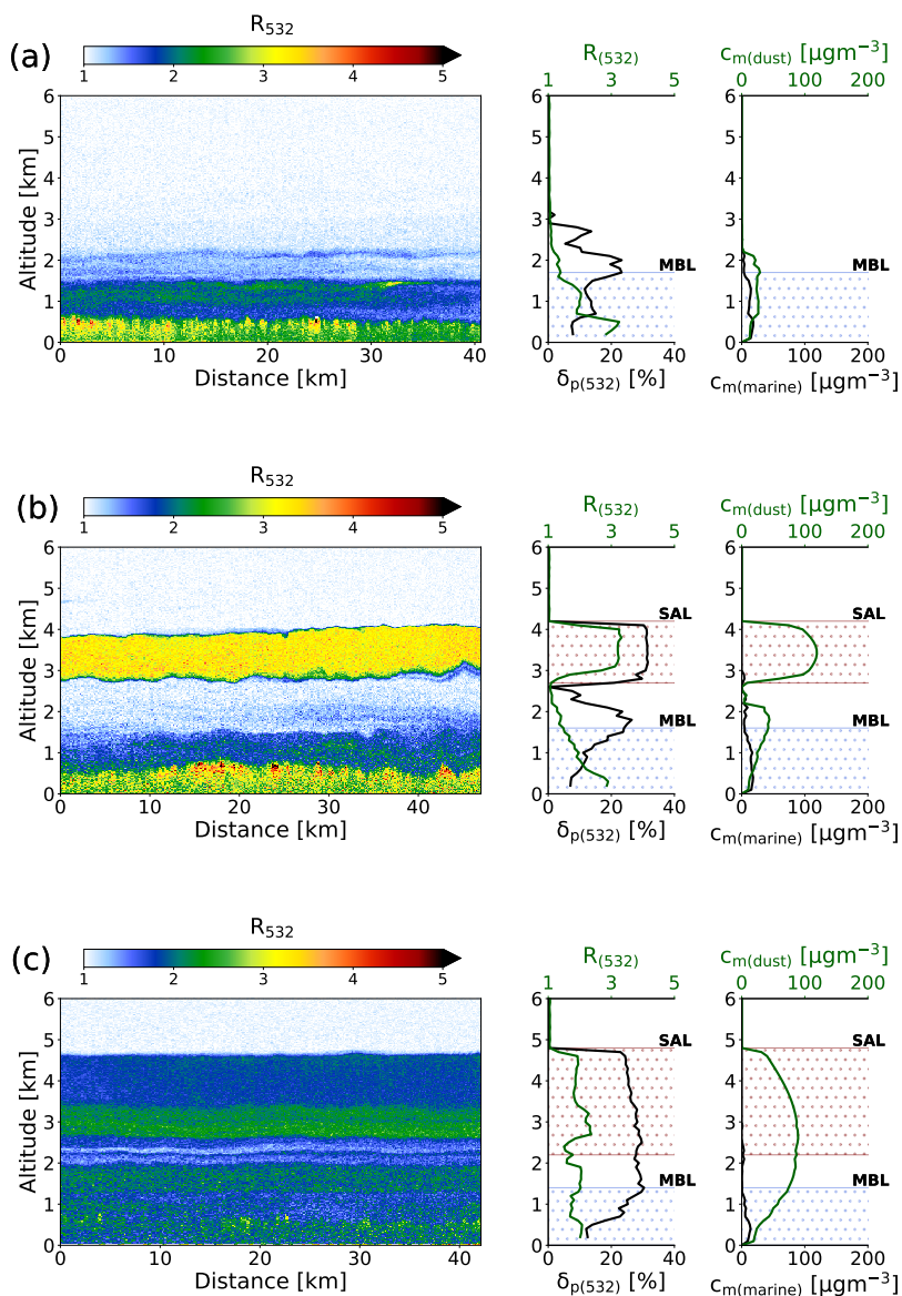
Figure 2. Left: cross-sections of WALES backscatter ratio R_{(532)} ; Middle: averaged profiles of particle linear depolarization ratios \delta_{p(532)} and backscatter ratio R_{(532)} ; Right: derived aerosol mass concentrations ( c_{m(\text{dust})} (red) and c_{m(\text{marine})} (blue)) for case (a) and (b) on 19 Aug 2016 as well as case (c) on 12 Aug 2016.
