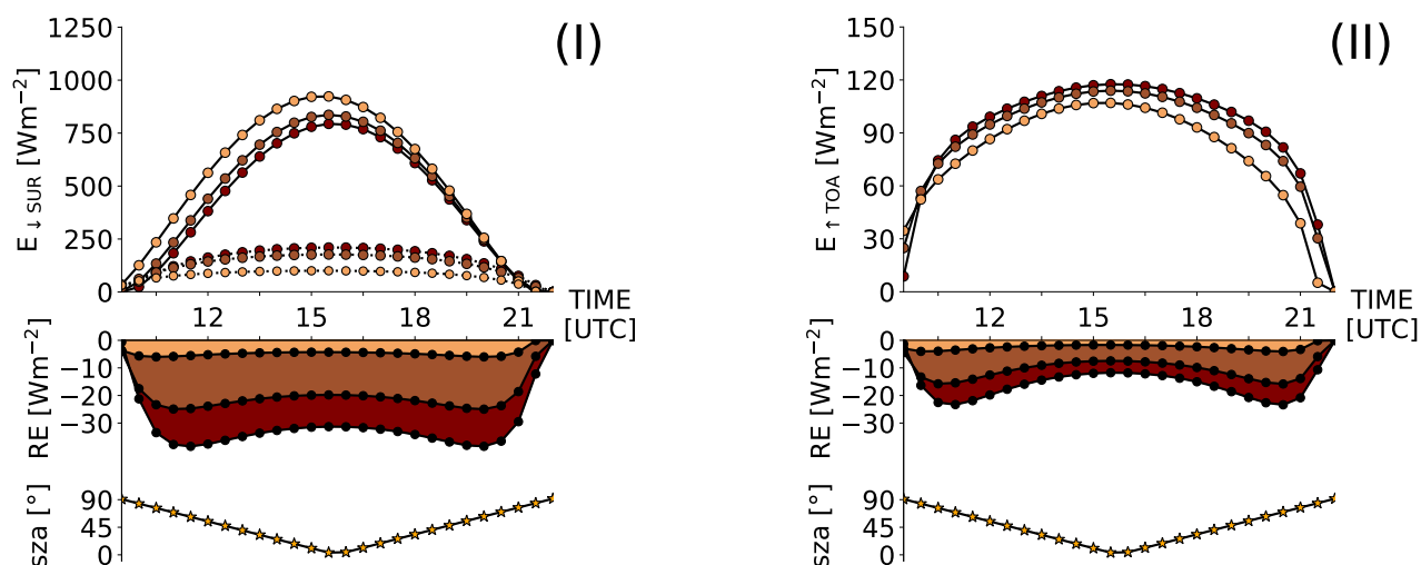
Figure 5. Top: Diurnal cycles of the modeled down-welling short-wave irradiances at surface level (I - E_{\downarrow\text{SUR}} : direct (solid), diffuse (dashed)) and up-welling short-wave irradiances at top of the atmosphere (II - E_{\uparrow\text{TOA}} ). Due to the different measurement locations and small differences in corresponding solar zenith angles (sza) calculated curves are slightly shifted in x-direction. Bottom: The corresponding diurnal cycles of the modeled Saharan dust short-wave radiative effects (RE) at surface level (I) and top of the atmosphere (II). A representative sza for the whole measurement region is shown at the bottom ( 11^{\circ}N and 55^{\circ}W ). Colors indicate the three cases: light-orange (case (a)), orange (case (b)), dark-orange (case (c)).
