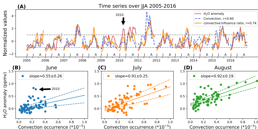
Figure 1. (A) Time series of normalized 100-hPa (red line) MLS water vapor anomaly (zonal mean removed), (blue line) convective occurrence from GridRad, and (orange line) the convective influence ratio in the back trajectory experiments. All data are 5-day averages over the NA region ( 25^{\circ}\text{N} - 50^{\circ}\text{N} , 70^{\circ}\text{W} - 130^{\circ}\text{W} ) during June, July, August 2005-2016. For the convective frequency, we use linear interpolation to estimate the value at 100 hPa. The convective influence ratio is the fraction of the MLS observations that encounter deep convection, as determined by the back trajectory calculations. (B-D) Joint distribution of convection and water vapor time series during 2005-2016 divided into (B) June, (C) July, and (D) August. Solid lines show the linear fit, and dashed lines show the 95% significant level margin of error of the slope bar (accounting for auto-correlation). To account for the time for the water vapor to spread out, each data point is a 10-day average of convection, with water vapor averaged over the last five days of the averaging period for convection.
