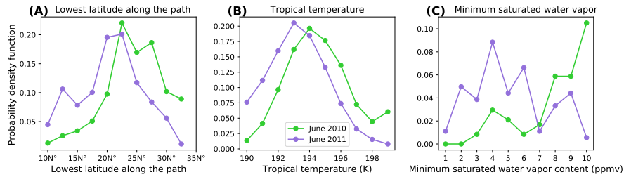
Figure 6. PDF of (A) lowest latitude along the path in the back trajectory experiments (B) mean tropical temperature (K) obtained from ERAi (0°-20°N, 70°W-130°W), and (C) minimum saturation water vapor mixing ratio (ppmv) in the back trajectory experiment results. Minimum saturation water vapor mixing ratios and lowest latitude are the minimum values along the path after the parcels encounter deep convection in the back trajectory model and prior to being observed by MLS.
