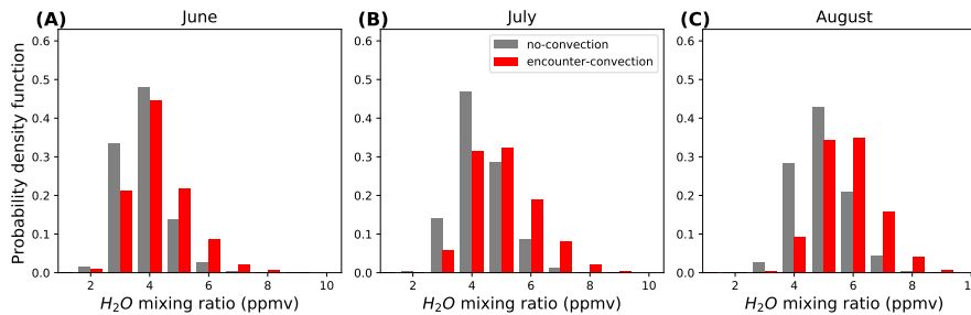
Figure 2. Probability density function of MLS water vapor observations at 100 hPa averaged over NA ( 25^{\circ}\text{N} - 50^{\circ}\text{N} , 70^{\circ}\text{W} - 130^{\circ}\text{W} ) in (A) June, (B) July, and (C) August 2005-2016. The observations are divided into two groups: (red) those whose back trajectory encounters convection and (grey) those that do not.
