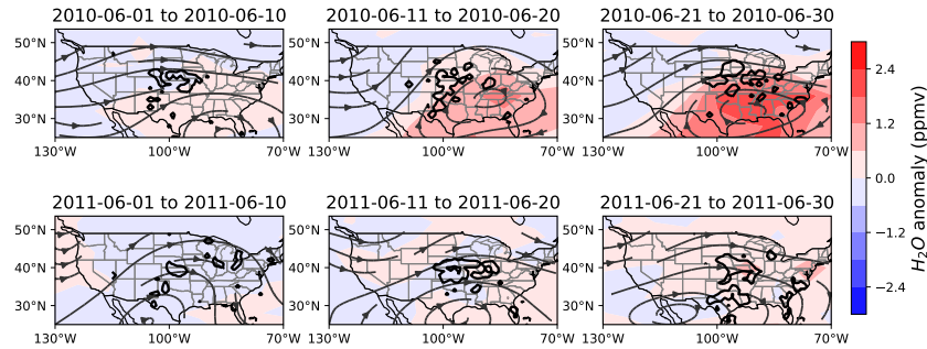
Figure 5. Ten day average water vapor anomaly (ppmv) at 100 hPa (after removing the zonal mean) during (top) June 2010 and (bottom) June 2011. Thick black contours are the 10 -5 contours of GridRad deep convection, and stream lines are horizontal velocity at 100 hPa obtained from ERAi averaged over the same period.
