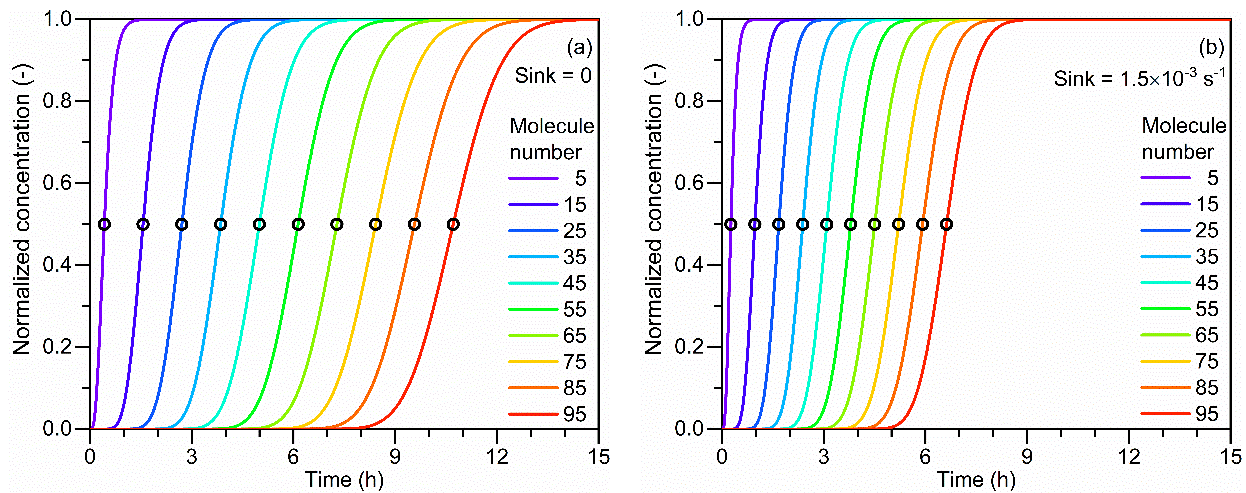
Figure 1 The principle of the appearance time method and the impact of the external sink. (a) Normalized particle concentrations as a function of time. The concentrations are normalized by dividing their corresponding maximum concentrations. The number concentration of the condensation vapor is assumed to be constantly 5 \times 10^6 \text{ cm}^{-3} . Particle coagulation sink and other sinks are assumed to be negligible. Particle size is indicated by the molecule number contained in every single particle. The open scatters indicate the 50% appearance time corresponding to each particle size. (b) A constant external sink of 1.5 \times 10^{-3} \text{ s}^{-1} is considered and other simulation conditions are the same as a). Note that due to the assumption of the size-independent coagulation coefficient, the appearance time in this figure deviates from their typical values in real new particle formation events.
